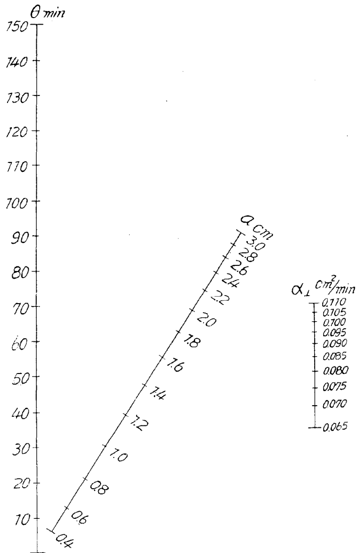
Fig. 31 Nomograph of \theta_{eq} = \frac{18.4a^2}{\alpha \pi^2}
