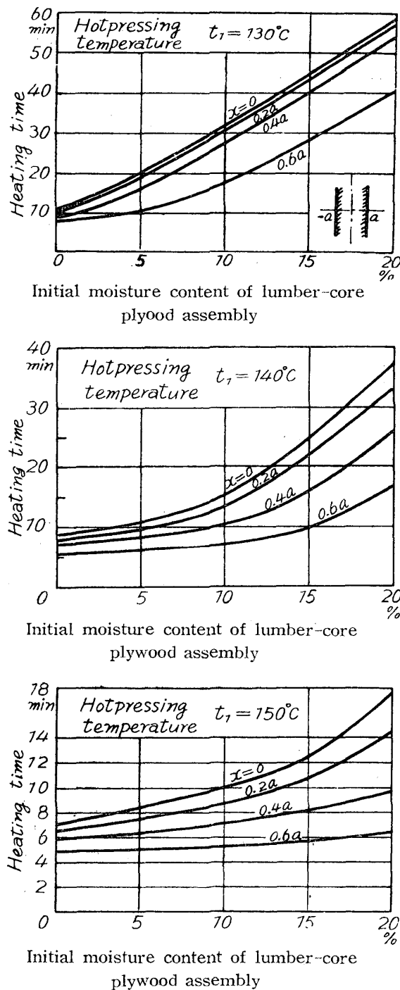
Fig. 44 Standard diagram of time required to reach 120^\circ\text{C} at each line x=0 , 0.2a , 0.4a and 0.6a at total thickness of plywood 2\text{cm} ( a=1 ). Initial wood temperature 20^\circ\text{C} .
