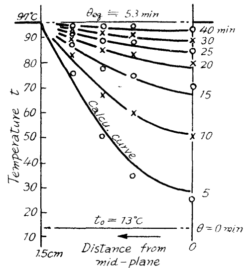
Fig. 24 Temperature distribution (Steaming), Fagus 3 cm thickness
