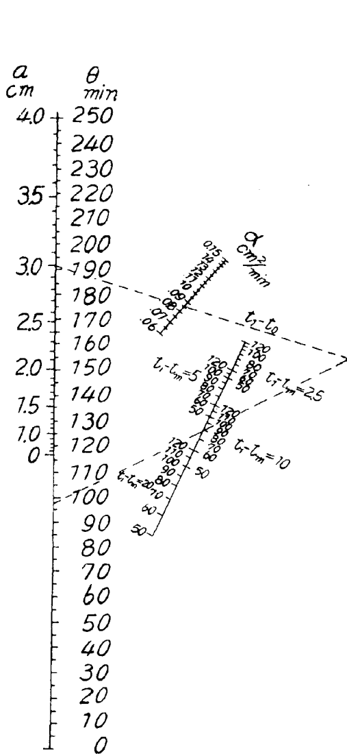
Fig. 30 Nomograph of \frac{t_1 - t_m}{t_1 - t_o} = \frac{4}{\pi} e^{-\alpha \left( \frac{\pi}{2a} \right)^2 \theta}
