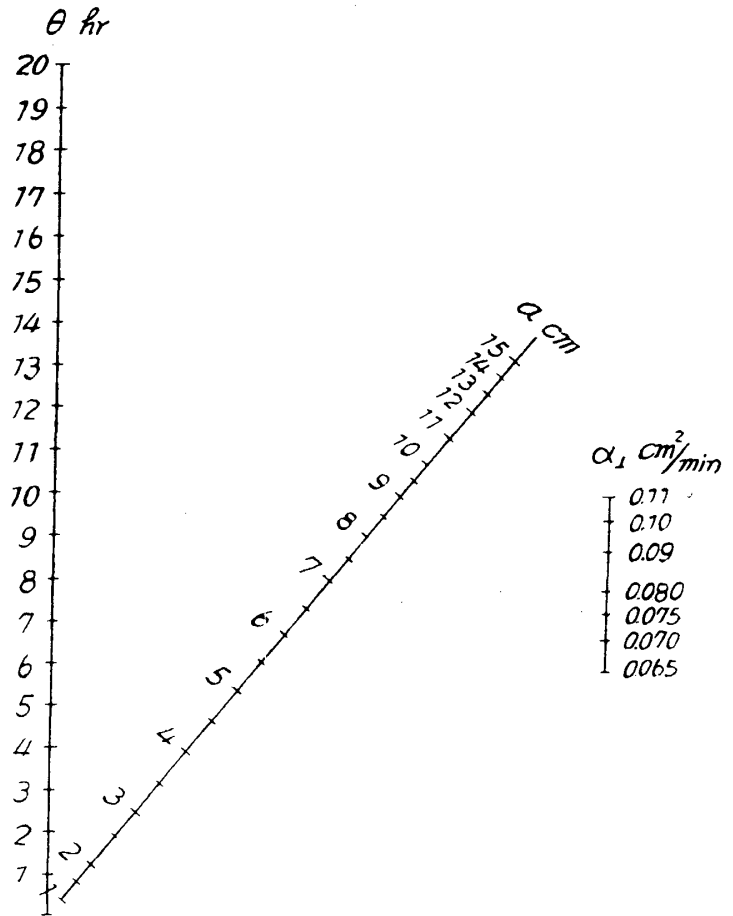
Fig. 38 Nomograph of \theta_{eq} = \frac{0.795a^2}{\alpha}
