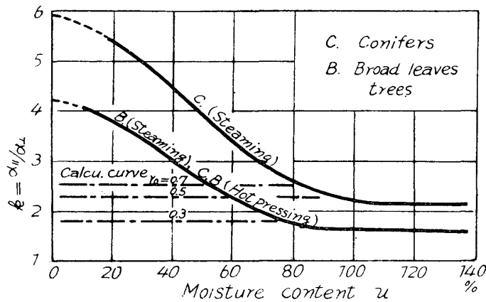
Fig. 26 Relation k = \alpha_{//} / \alpha_{\perp} and the moisture content
