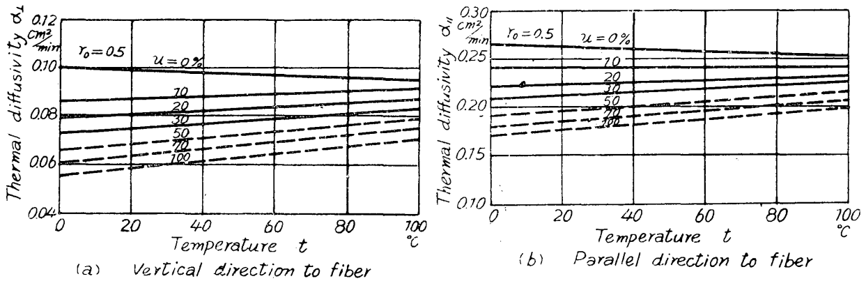
Fig. 11 Relation between the temperature and the thermal diffusivity
