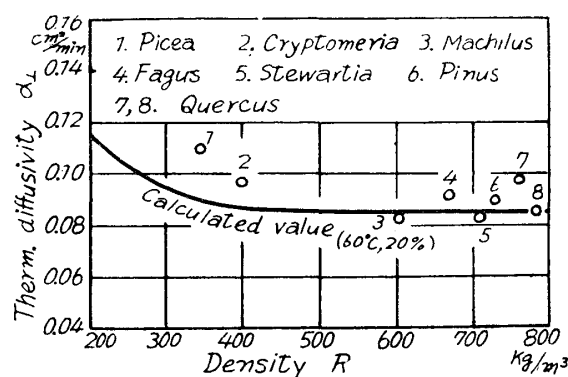
Fig. 19 Relation between the density and the thermal diffusivity (Steaming)
