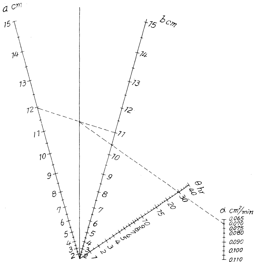
Fig. 35 Nomograph of \theta_{eq} = \frac{1.86}{a \left( \frac{1}{a^2} + \frac{1}{b^2} \right)}
