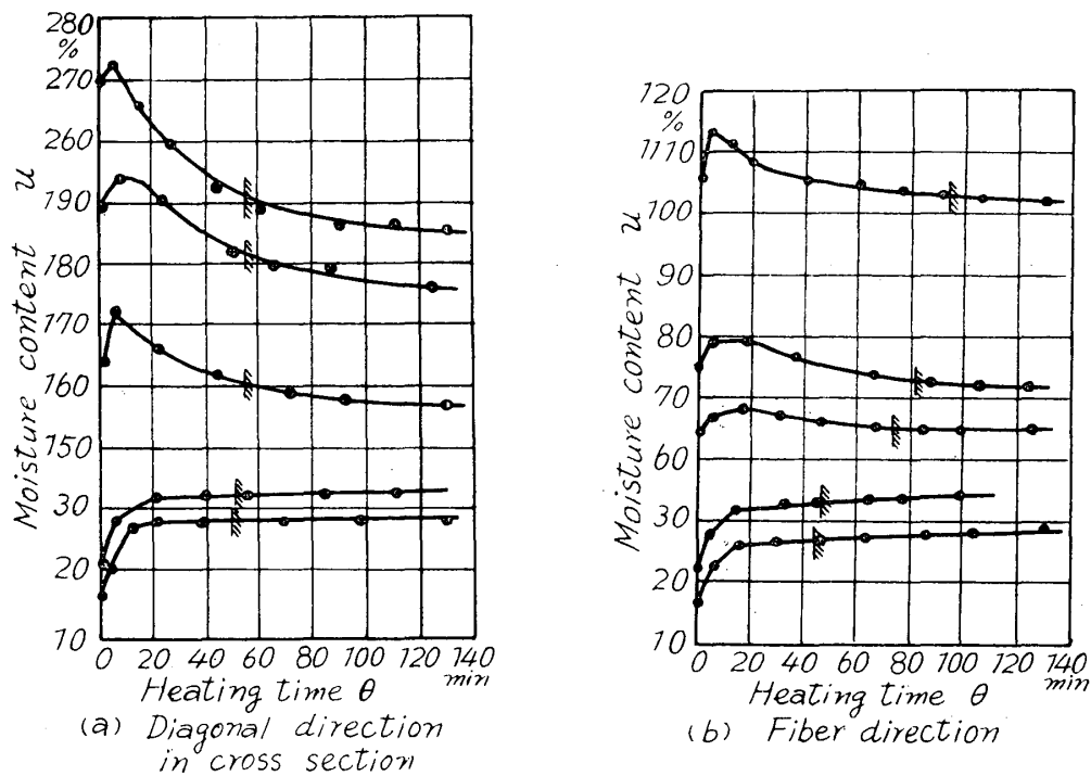
Fig. 27 Change of moisture content in Cryptomeria (Steaming)
