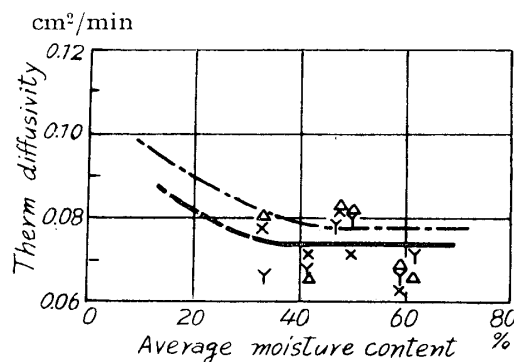
Fig. 47 Relation of \alpha_{\perp} to the average moisture content of all-veneer plywood (Hotpressing)
