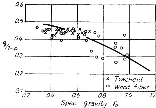
Fig. 7 Relation between q/1-p and the spec. gravity
