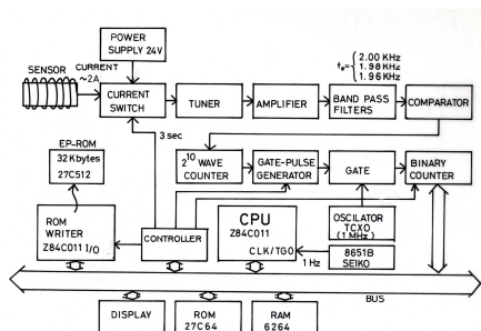
Fig.7. Block diagram of the proton magnetometer system, OSMAN2 (after Oshiman, 1989).
