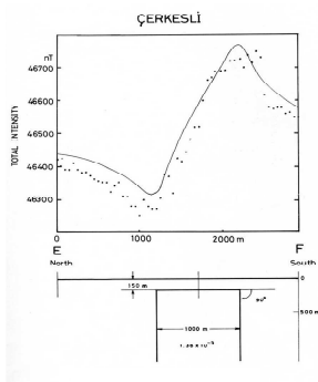
Fig.6. The magnetic anomaly observed at Cerklesli (dots) and the anomaly (solid line) calculated from the best fit 2D magnetic dyke model (after Isikara et al. , 1985).
