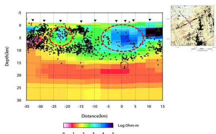
Fig.11. Two-dimensional resistivity structure along the Atotsugawa fault deduced from wide-band MT data (after Yoshimura et al. , 2006).
