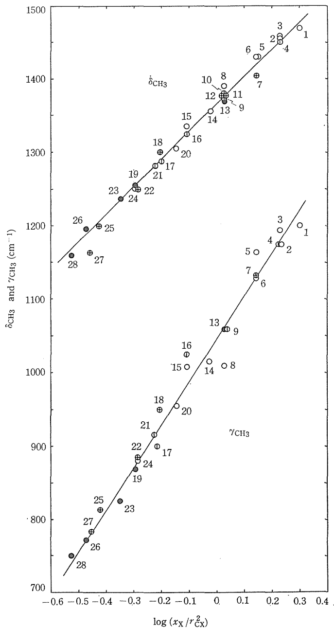
Fig. 1. Plot of \delta_{\text{CH}_3} and \gamma_{\text{CH}_3} against \log(x_X/r_{\text{CX}}^2) for (\text{CH}_3)_n\text{XH}_{m-n} and (\text{CH}_3)_n\text{XD}_{m-n} molecules.
