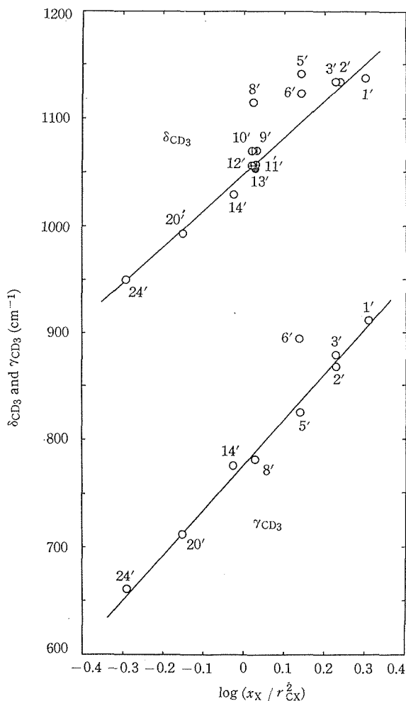
Fig. 4. Plot of \delta_{\text{CD}_3} and \gamma_{\text{CD}_3} against \log(x_{\text{X}}/r_{\text{CX}}^2) for (\text{CD}_3)_n\text{XH}_{m-n} and (\text{CD}_3)_n\text{XD}_{m-n} molecules.
