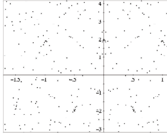
Figure 1. Graph of \Re(f(x))
