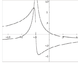
Figure 2. Graph of \Re(h(x)) and \Im(h(x))
