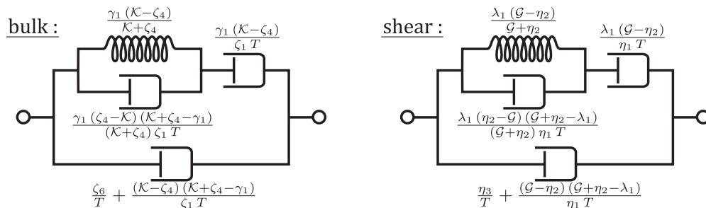
FIG. 10. Schematic structure of the bulk part (left) and the shear part (right). Note that the contribution of \tau_{\mu\nu}^{(q)} is omitted for simplicity.
