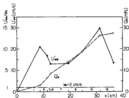
Fig. 7 Variation of water discharge and shear velocity along the main channel at maximum subsurface run-off stage.
