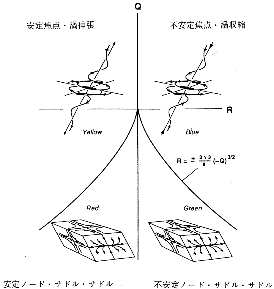
図 5 Identification of local non-degenerate flow topologies in the plane P = 0 .
