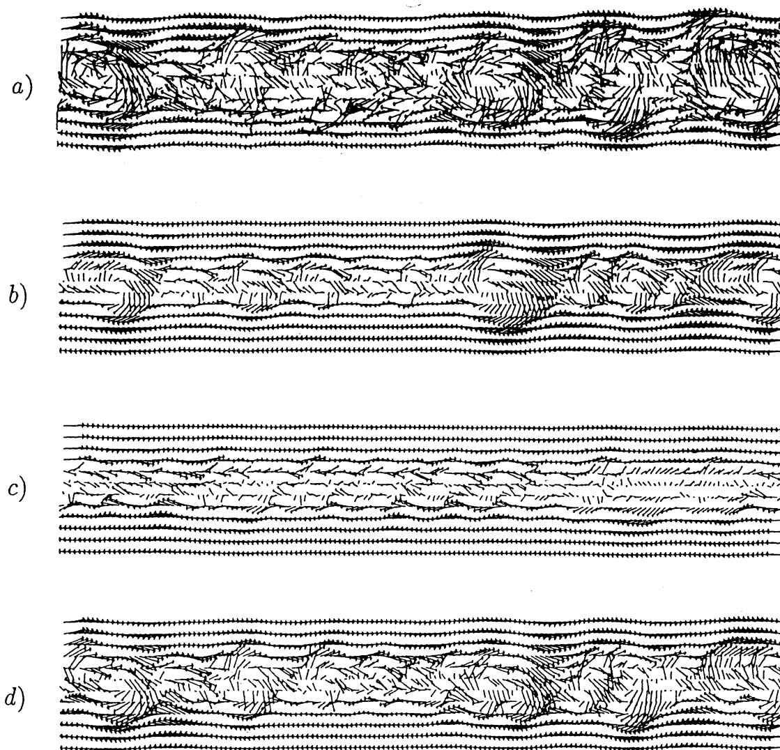
Fig. 2 Instantaneous flow patterns in the mixing layer, experiment I: a) Original directly measured velocity field. b) Contribution of first mode of the POD uv . c) Contribution of the second mode. d) Contribution of the first three modes.
