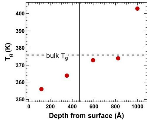
Fig. 6 Distribution of glass transition temperature T_g in 5-layer thin film
