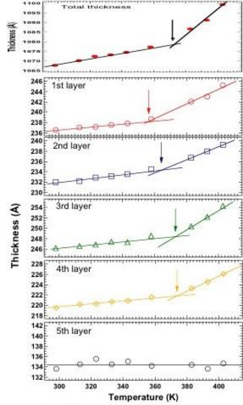
Fig. 5 Temperature dependence of film thickness of each layer.
