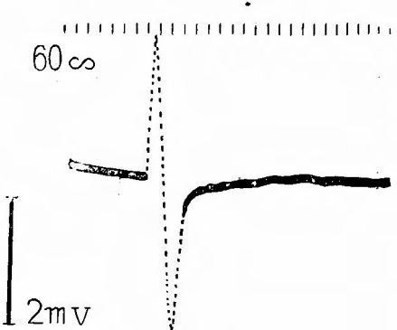
Fig. 6 Reinnervation voltage.
