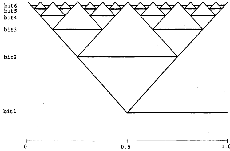
Figure 1: Gray code Embedding of real numbers.
