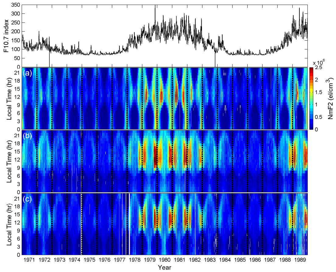
Figure 2. The daily variations of the 10.7 cm solar radio flux, F10.7 index (in unit of 10^{-22}\text{Wm}^{-2}\text{Hz}^{-1} ), and the NmF2 at (a)AIJ6N, (b)LN047, and (c)MG560 stations during 1971 to 1989.
