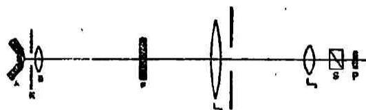
Fig. 1. Arrangement of the apparatus for illuminating the photographic plate by infra-red light.
