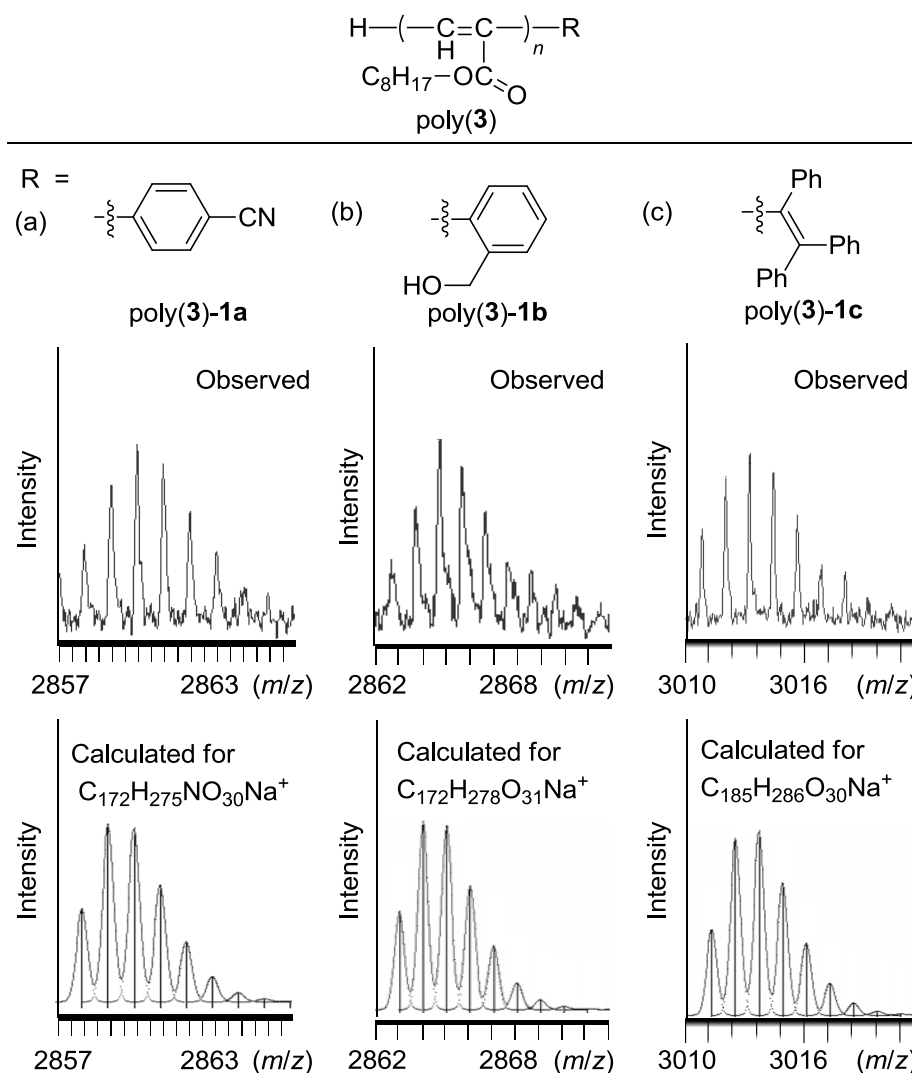
Figure 6. Selected isotope patterns in the MALDI-TOF mass spectra observed (enlarged view of the data presented in Figure 5) and calculated for (a) poly(3)-1a, (b) poly(3)-1b and (c) poly(3)-1c.
