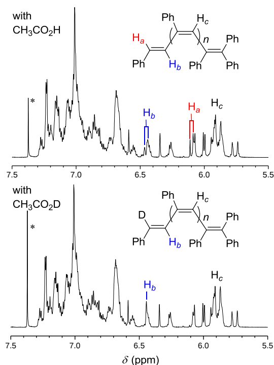
Figure 9. ^1\text{H} NMR spectra (700 MHz) in \text{CD}_2\text{Cl}_2 of poly(PA) quenched with \text{CH}_3\text{CO}_2\text{H} and \text{CH}_3\text{CO}_2\text{D} . *: \text{CHCl}_3 contamination from the preparative HPLC purification. The chemical shifts are calibrated to the \text{CH}_2\text{Cl}_2 signal (5.33 ppm, not shown). 32
