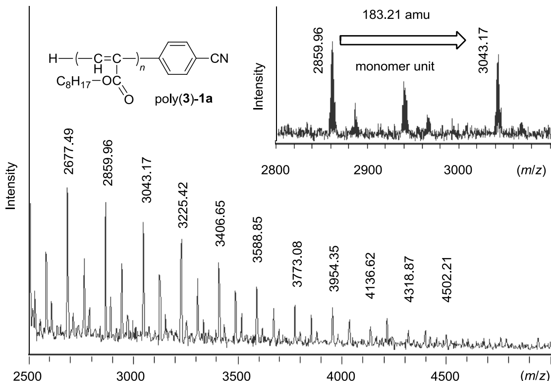
Figure 4. MALDI-TOF mass spectrum of poly(3)-1a acquired with DHB/NaTFA matrix. The inset shows a partial amplification.
