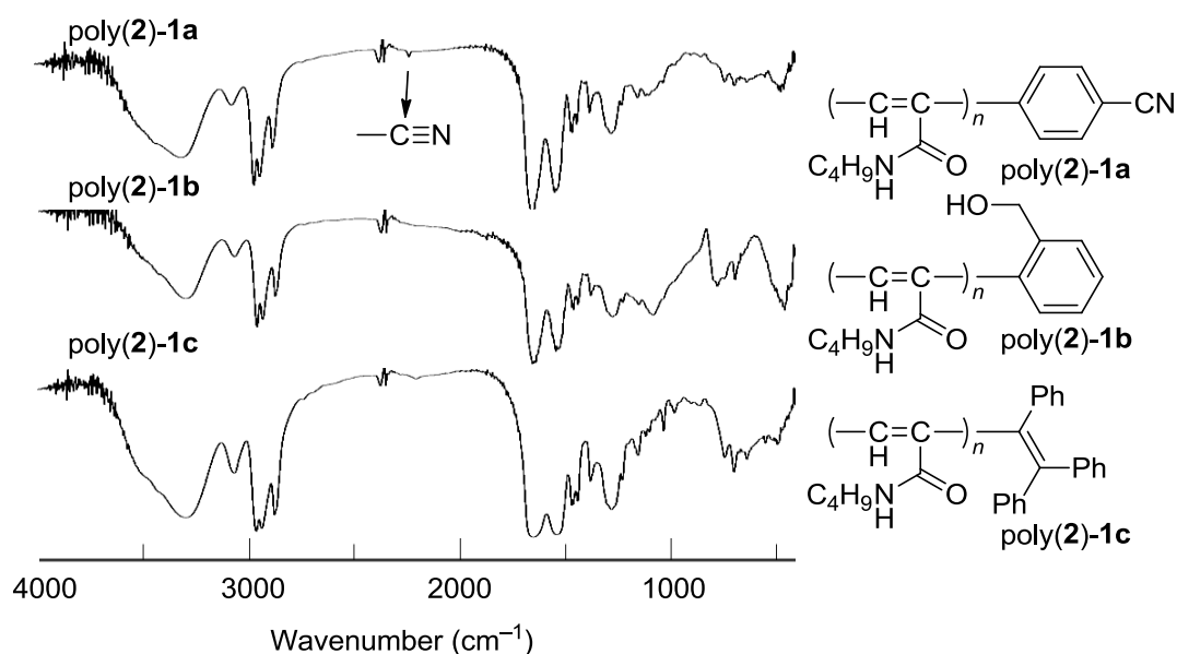
Figure 3. IR spectra of poly(2)-1a, poly(2)-1b and poly(2)-1c (KBr pellet).
