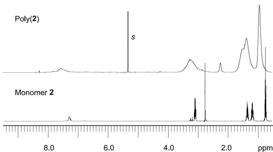
Figure 2. ^1\text{H} NMR spectra of poly(2) and monomer 2 measured in \text{CDCl}_3 at r.t. (s: solvent).
