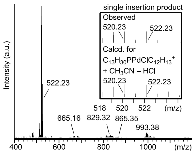
Figure 11. ESI-mass spectrum of a mixture of 1 /AgOTf and 4 (1:1). Inset: expanded experimental and calculated isotope patterns of a peak.
