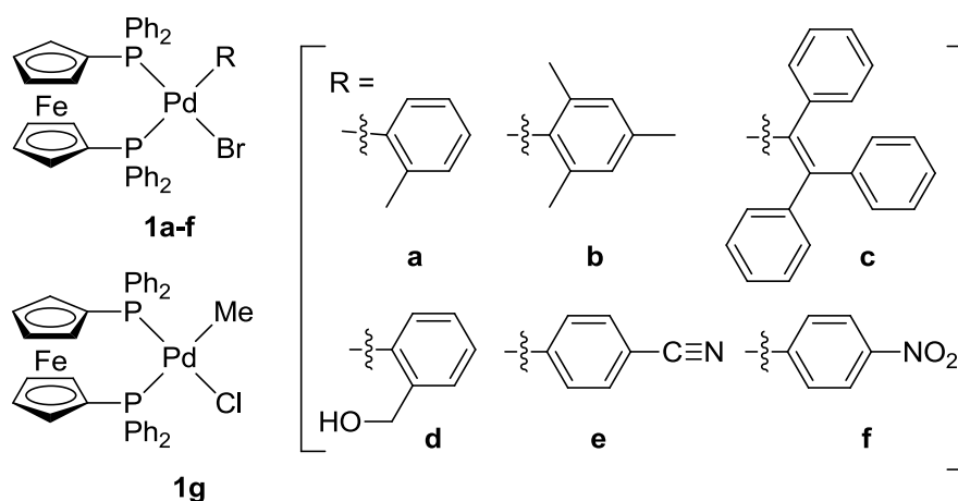
Chart 1. Pd catalysts 1a–g bearing a variety of R groups.
