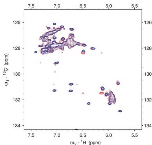
Figure 10. ^1\text{H} – ^{13}\text{C} HSQC NMR spectra (700 MHz) in \text{CD}_2\text{Cl}_2 of poly(PA) obtained by the polymerization quenched with \text{CH}_3\text{CO}_2\text{H} (red) and \text{CH}_3\text{CO}_2\text{D} (blue).
