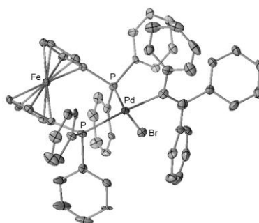
Figure 1. X-ray structure of 1c (a selected molecule among two in the unit cell, described with 30% probability ellipsoids)
