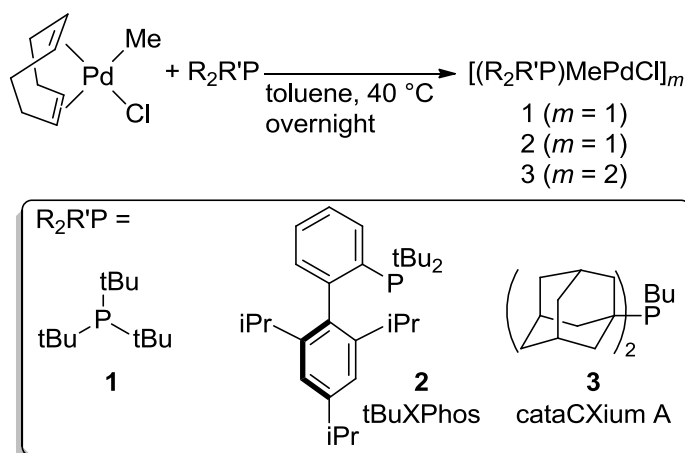
Scheme 1. Synthesis of bulky monophosphine-ligated palladium complexes
