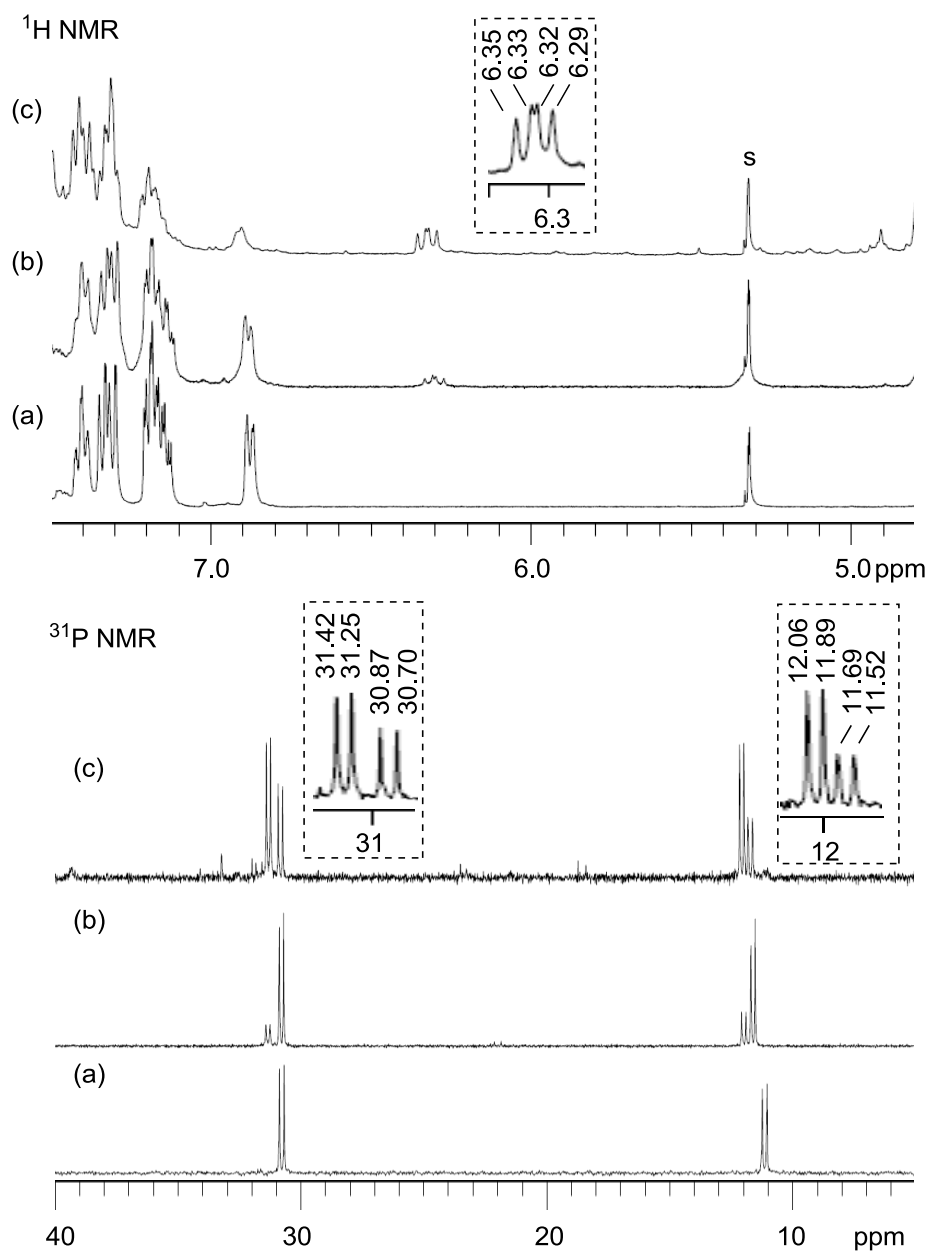
Figure 7. ^1\text{H} and ^{31}\text{P} NMR spectra of (a) 1\text{aOTf} , (b) 1\text{aOTf} + 1 equivalent of 5 , (c) 1\text{aOTf} + 3 equivalents of 5 measured in \text{CD}_3\text{CN}/\text{CD}_2\text{Cl}_2 = 1/3 (v/v), [1\text{aOTf}]_0 = 34 mM at r.t. (s: solvent)
