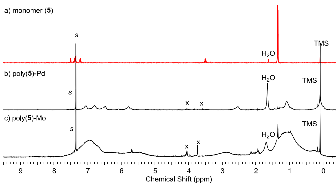
Figure 3. ^1\text{H} NMR spectra of: a) monomer 5 ; b) poly( 5 ) synthesized by the polymerization using t\text{Bu}_3\text{PPdMeCl} ( 6 )/AgOTf (Table 1, entry 9) and, c) poly( 5 ) synthesized by \text{MoCl}_5/\text{SnBu}_4 (Table 1, entry 10) measured in \text{CDCl}_3 at room temperature (s: solvent, x: impurity).
