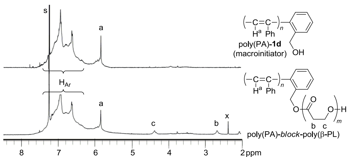
Figure 7. ^1\text{H} NMR spectra of macroinitiator, poly(PA)-1d, and poly(PA)-block-poly( \beta -PL) [in \text{CDCl}_3 , s: solvent, x: impurity].
