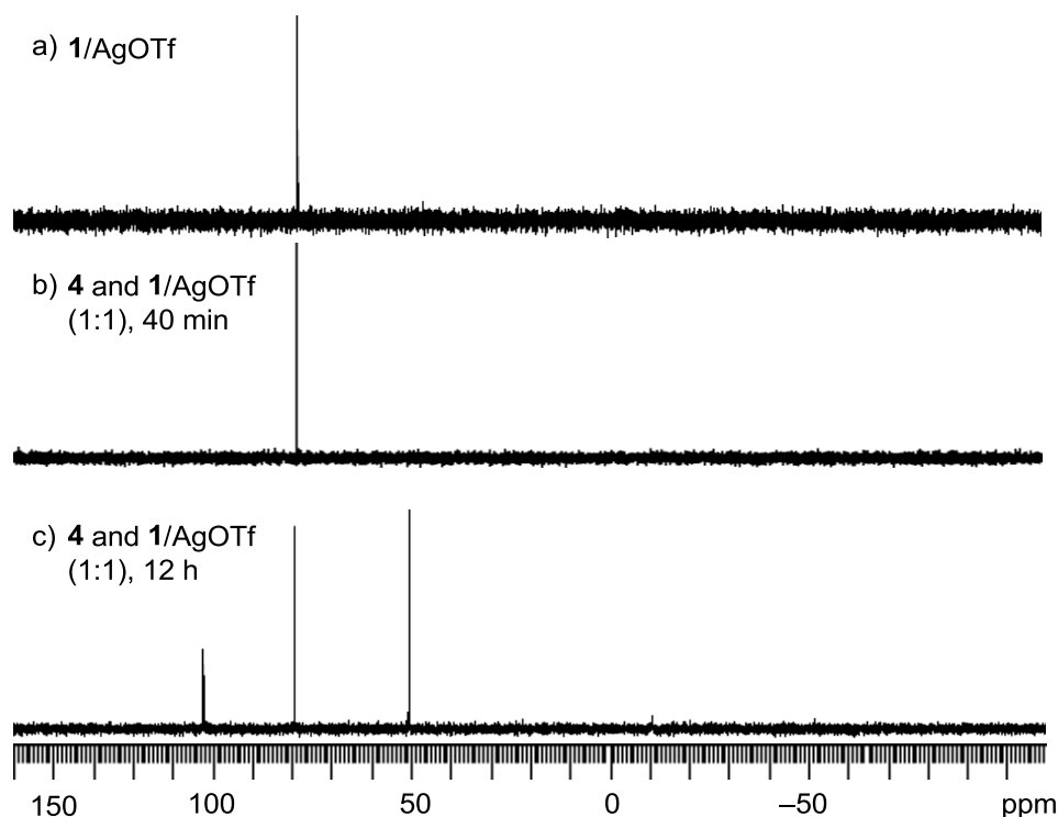
Figure 10. ^{31}\text{P} NMR spectra of: a) 1 /AgOTf, b) 1 /AgOTf and 4 (1:1) after 40 min of reaction; c) 1 /AgOTf and 4 (1:1) after 12 h of reaction. Detailed reaction conditions are described in Scheme 4 and the experimental section. The spectra were measured at 50 °C in \text{C}_6\text{D}_6 .
