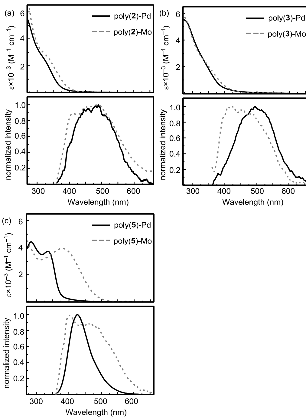
Figure 9. UV-vis absorption (top of a, b and c) and emission (bottom of a, b and c) spectra of poly(2) (a), poly(3) (b) and poly(5) (c) synthesized by the polymerization using t\text{Bu}_3\text{PPdMeCl} (6)/AgOTf (solid line) and \text{MoCl}_5/\text{SnBu}_4 (dotted line) measured in THF at room temperature ( c = 0.02 \text{ mM} ). Excitation wavelength: 320 nm.
