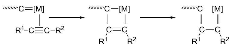
Scheme 2. Metathesis mechanism for the polymerization of acetylene monomers.
