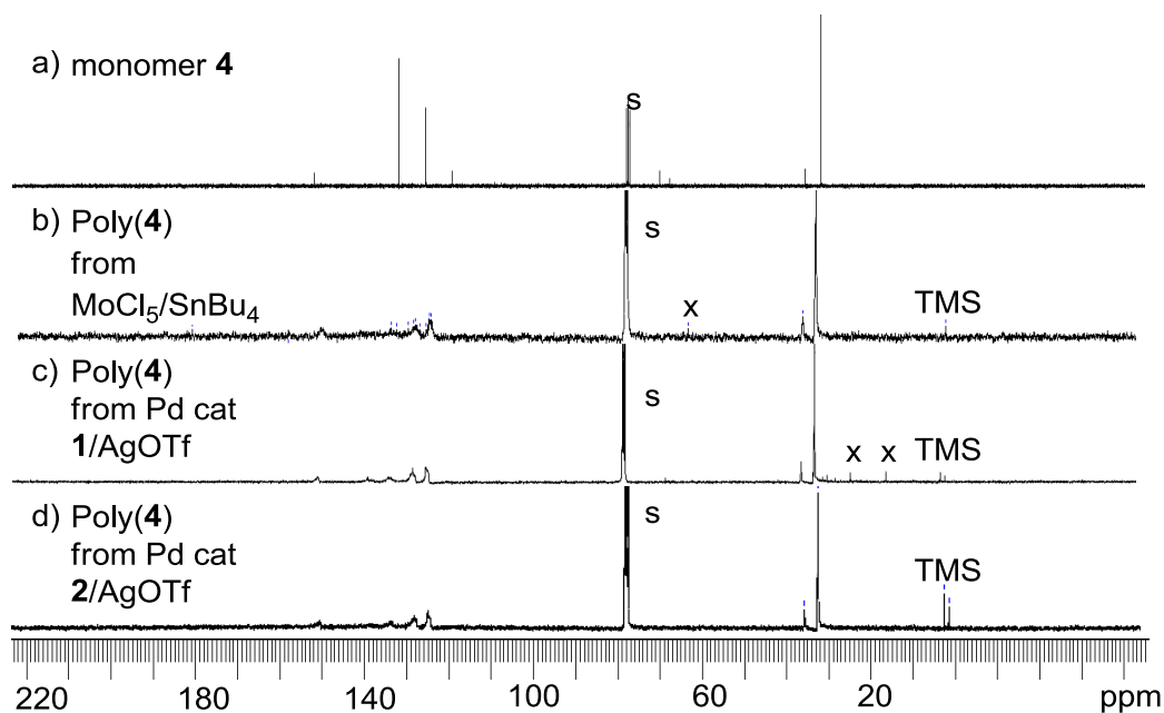
Figure 6. ^{13}\text{C} NMR spectra of: a) monomer 4; b) poly(4) synthesized by \text{MoCl}_5/\text{SnBu}_4 (Table 1, entry 4); c) poly(4) synthesized by Pd catalyst 1/ \text{AgOTf} (Table 1, entry 1) and d) poly(4) synthesized by Pd catalyst 2/ \text{AgOTf} (Table 1, entry 2). All spectra were measured in \text{CDCl}_3 at rt. (s: solvent, x: impurity).
