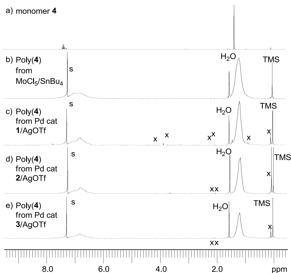
Figure 5. 1 H NMR spectra of: a) monomer 4 ; b) poly( 4 ) synthesized by MoCl 5 /SnBu 4 (Table 1, entry 4); c) poly( 4 ) synthesized by Pd catalyst 1 /AgOTf (Table 1, entry 1); d) poly( 4 ) synthesized by Pd catalyst 2 /AgOTf (Table 1, entry 2) and e) poly( 4 ) synthesized by Pd catalyst 3 /AgOTf (Table 1, entry 3). All spectra were measured in CDCl 3 at rt. (s: solvent, x: impurity).
