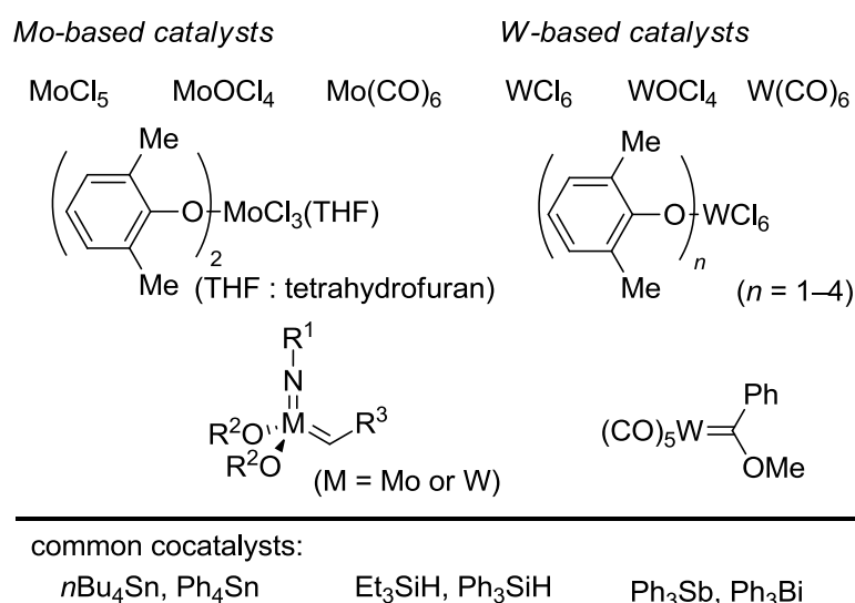
Chart 1. Common early transition metal catalysts
