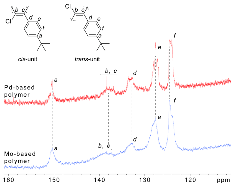
Figure 7. Expansion of ^{13}\text{C} NMR (150 MHz) spectra of poly(4)s synthesized by: upper) Pd catalyst 1/ \text{AgOTf} (entry 1 in Table 1) and lower) \text{MoCl}_5/\text{SnBu}_4 (entry 4 in Table 1). The spectra were measured in \text{CDCl}_3 at rt.
