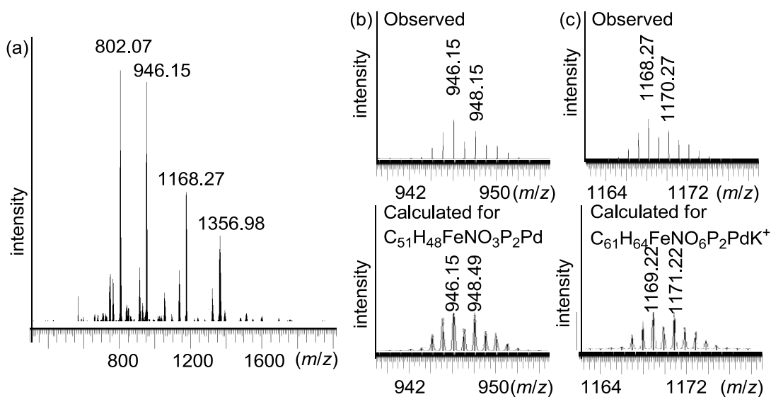
Figure 8. (a) ESI-mass spectrum of a mixture of 1aOTf and 3 equivalents of 5 . (b) and (c): Isotope patterns in the ESI-mass spectra observed and calculated for single and double insertion products, respectively.
