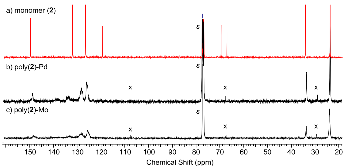
Figure 4. ^{13}\text{C} NMR spectra of: a) monomer 2 ; b) poly( 2 ) synthesized by the polymerization using t\text{Bu}_3\text{PPdMeCl} ( 6 )/AgOTf (Table 1, entry 3) and, c) poly( 2 ) synthesized using \text{MoCl}_5/\text{SnBu}_4 (Table 1, entry 4) measured in \text{CDCl}_3 at room temperature (s: solvent, x: impurity).
