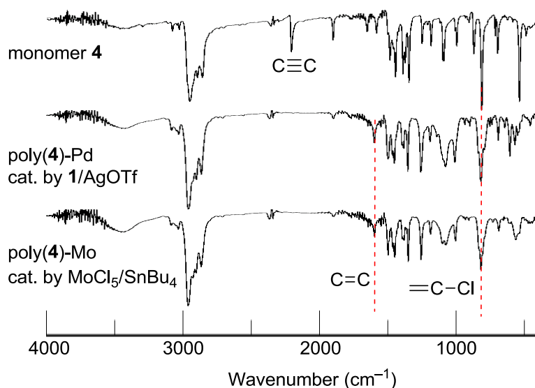
Figure 2. IR spectra of monomer 4 , poly( 4 ) obtained by the 1/AgOTf catalytic system (Table 1, entry 1) and poly( 4 ) obtained by the MoCl 5 /SnBu 4 catalytic system (Table 1, entry 4).
