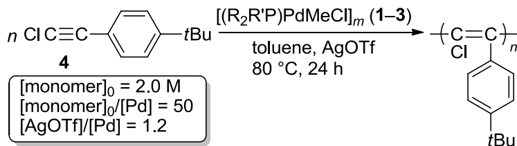
Scheme 2. Polymerization of 1-chloro-2-(4- tert -butyl)phenylacetylene ( 4 ) by (R 2 R'P)PdMeCl ( 1–3 )/AgOTf
