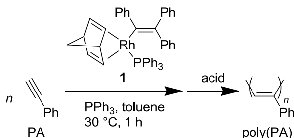
Scheme 2. Polymerization of PA using 1 as a catalyst.
