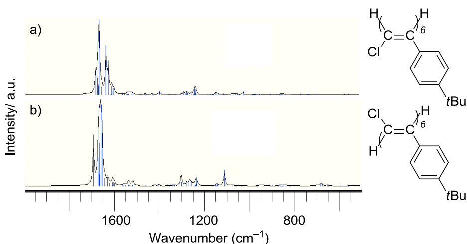
Figure 4. Raman spectra of a hexamer of 4 featuring: a) cis -stereochemistry and b) trans -stereochemistry simulated by the DFT (B3LYP/6-31G*) calculations.
