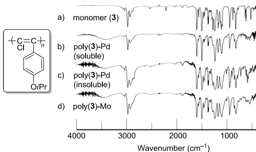
Figure 7. IR spectra of: a) monomer 3 ; b) poly( 3 ) synthesized by the polymerization using t\text{Bu}_3\text{PPdMeCl} ( 6 )/AgOTf (Table 1, entry 5), c) insoluble fraction of poly( 3 ) synthesized using t\text{Bu}_3\text{PPdMeCl} ( 6 )/AgOTf (Table 1, entry 5) and, d) poly( 3 ) synthesized using \text{MoCl}_5/\text{SnBu}_4 (Table 1, entry 6) measured by the KBr pellet method.
