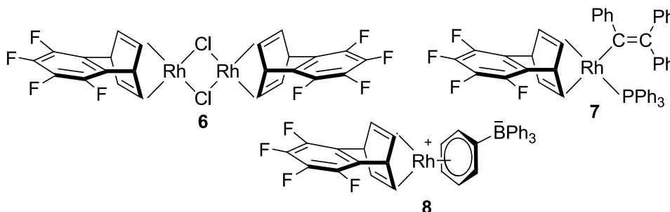
Chart 3. Tetrafluorobenzobarrelene-based Rh catalysts.
