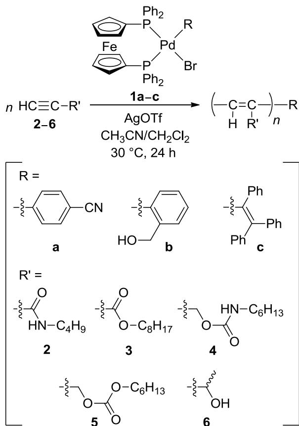
Scheme 1. Polymerization of monosubstituted polar acetylene monomers 2–6 by well-defined Pd catalysts 1a–c /AgOTf
