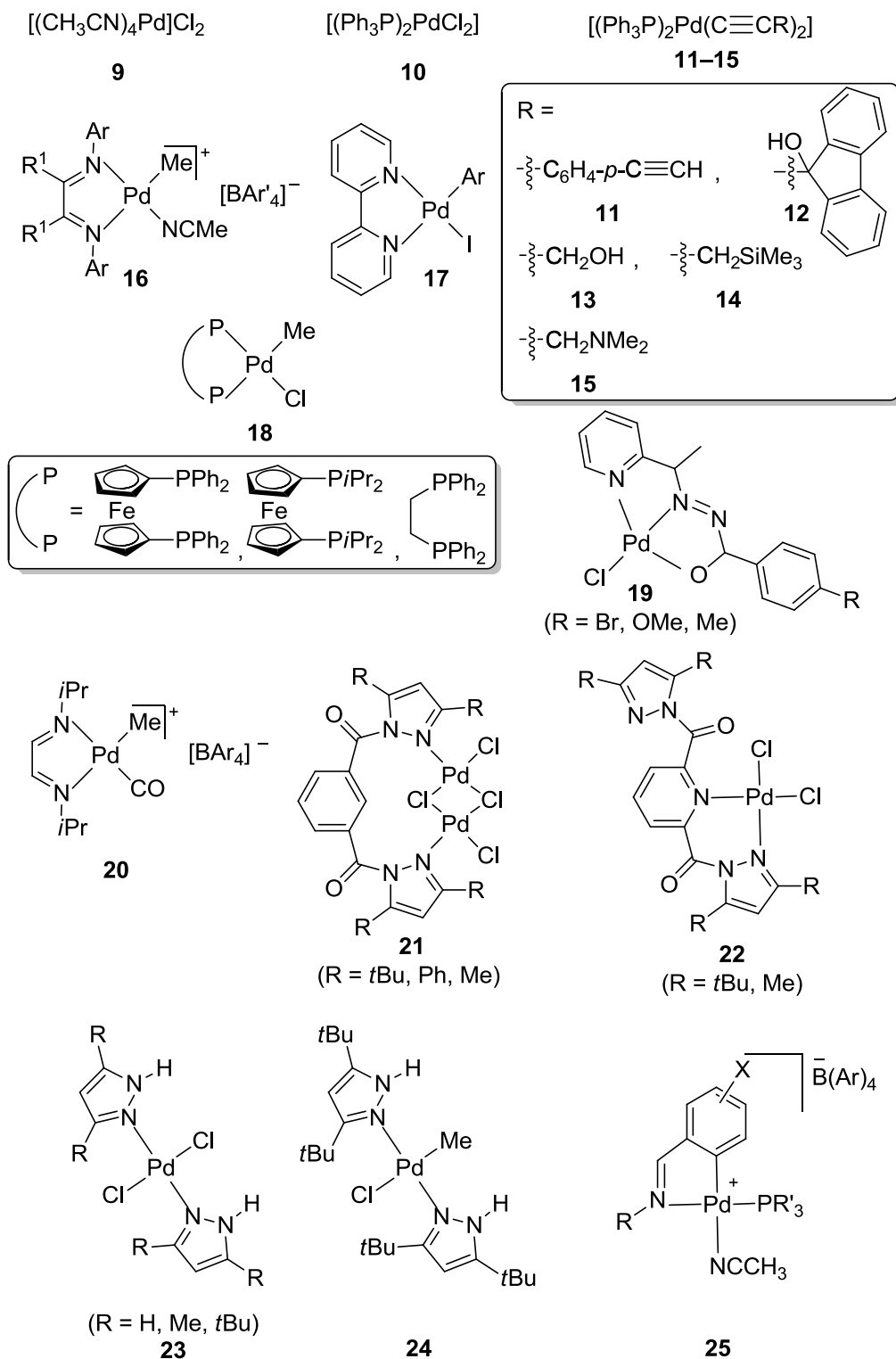
Chart 4. Pd catalysts employed for the polymerization of substituted acetylenes.
