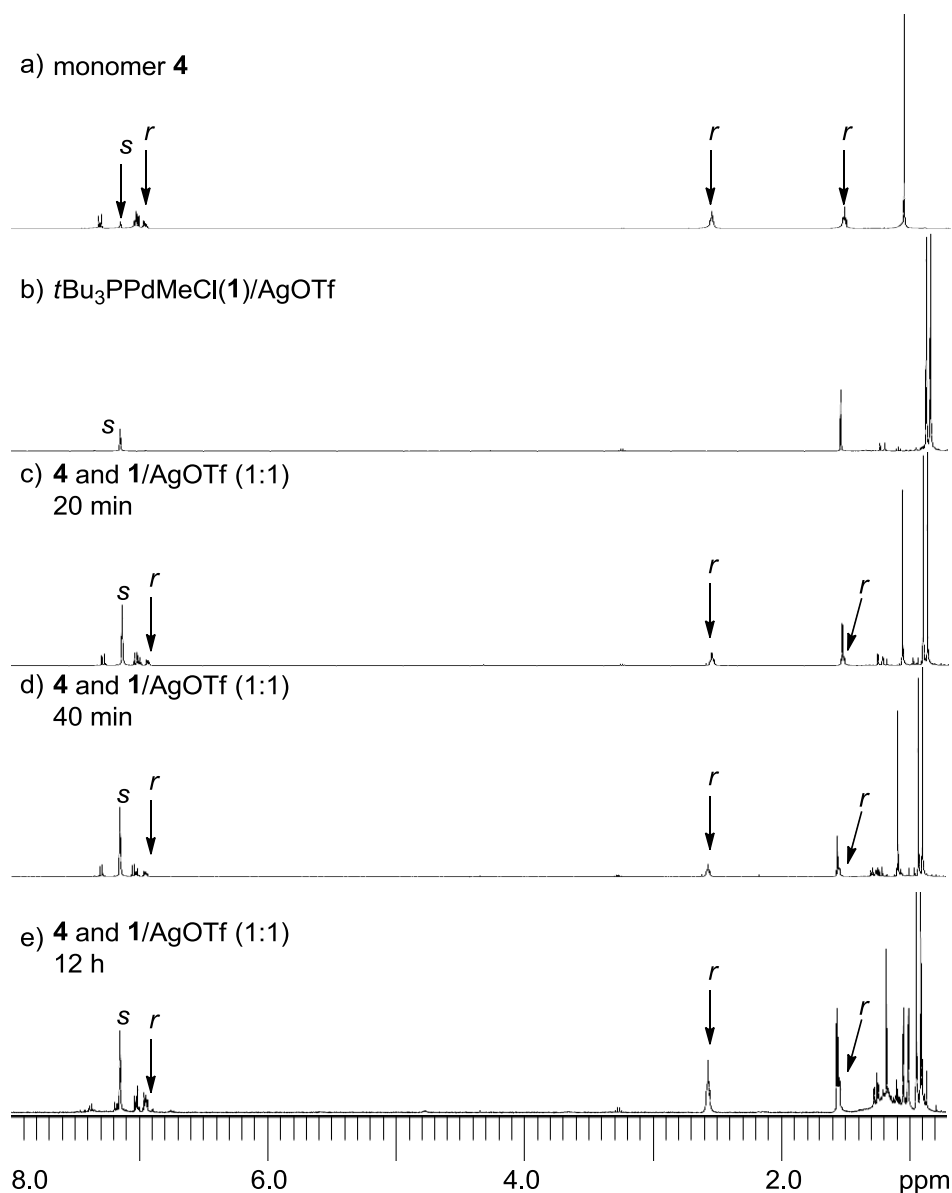
Figure 8. ^1\text{H} NMR spectra of: a) monomer 4 and 1,2,3,4-tetrahydronaphthalene ( r ); b) 1 / \text{AgOTf} ; c) 1 / \text{AgOTf} and 4 (1:1) after 20 min of reaction; d) 1 / \text{AgOTf} and 4 (1:1) after 40 min of reaction; e) 1 / \text{AgOTf} and 4 (1:1) after 12 h of reaction. Detailed reaction conditions are described in Scheme 4 and the experimental section. The spectra were measured at 50°C in \text{C}_6\text{D}_6 ( s : solvent).
