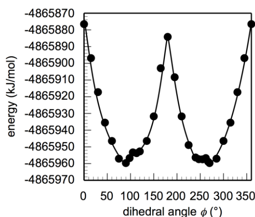
Figure 3. Relationship between the dihedral angle ( \phi ) values of P–Rh–C=C and energies of 1 calculated by the B3LYP/LANL2DZ method.
