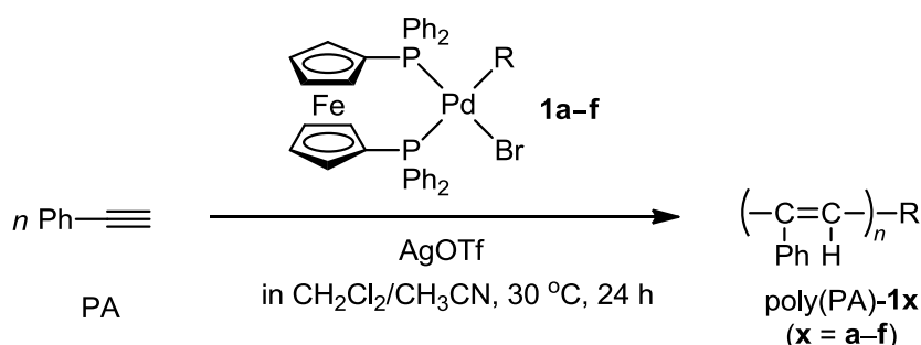
Scheme 1. Polymerization of PA with Pd catalysts 1a–f .
