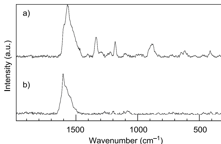
Figure 3. Raman spectra of: a) poly( 4 )-1 (Table 1, entry 1) and b) poly( 4 )-Mo (Table 1, entry 4).
