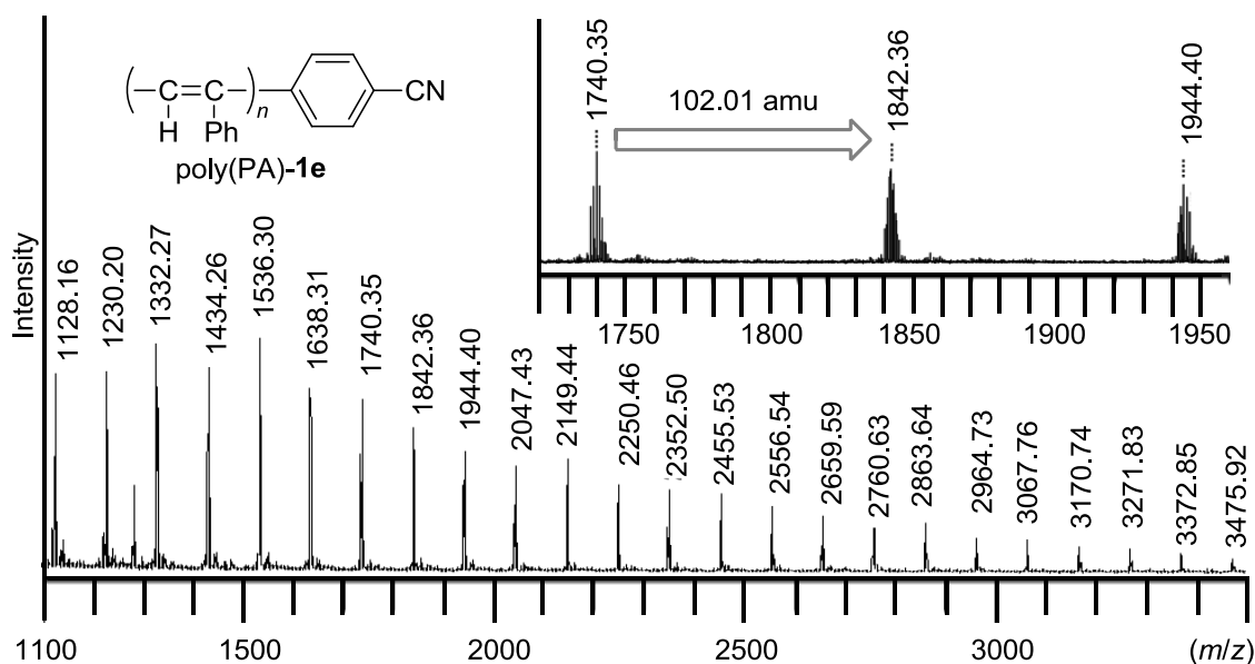
Figure 3. MALDI-TOF mass spectrum of poly(PA)-1e acquired with DCTB/AgTFA matrix.
