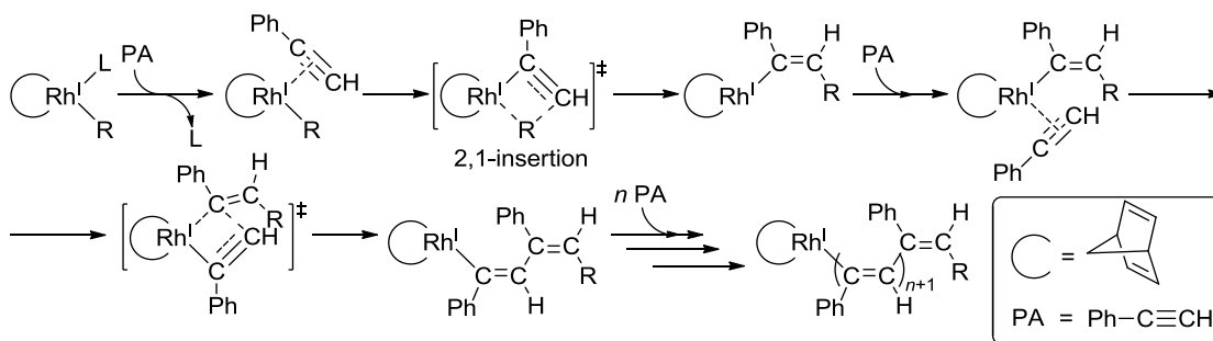
Scheme 3. Proposed mechanism for the Rh-catalyzed polymerization of phenylacetylene (PA).
