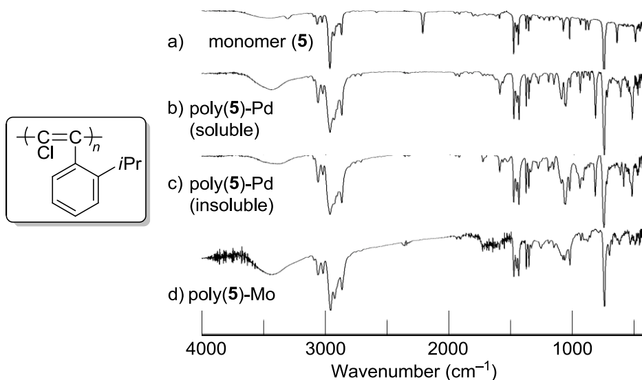
Figure 8. IR spectra of: a) monomer 5 ; b) poly( 5 ) synthesized by the polymerization using t\text{Bu}_3\text{PPdMeCl} ( 6 )/AgOTf (Table 1, entry 9), c) insoluble fraction of poly( 5 ) synthesized using t\text{Bu}_3\text{PPdMeCl} ( 6 )/AgOTf (Table 1, entry 9) and, d) poly( 5 ) synthesized using \text{MoCl}_5/\text{SnBu}_4 (Table 1, entry 10) measured by the KBr pellet method.
