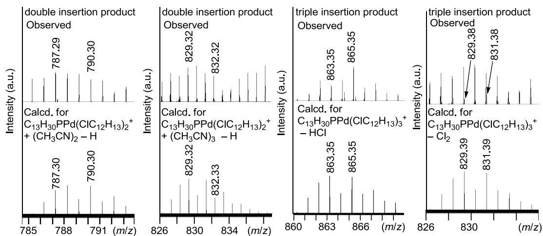
Figure 12. Amplification for some of the observed and calculated signals in the ESI-mass spectrum of a mixture of 1 /AgOTf and 4 (1:1) (Figure 11).
