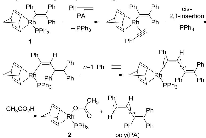
Scheme 3. Polymerization pathway of PA using 1 as an initiator.
