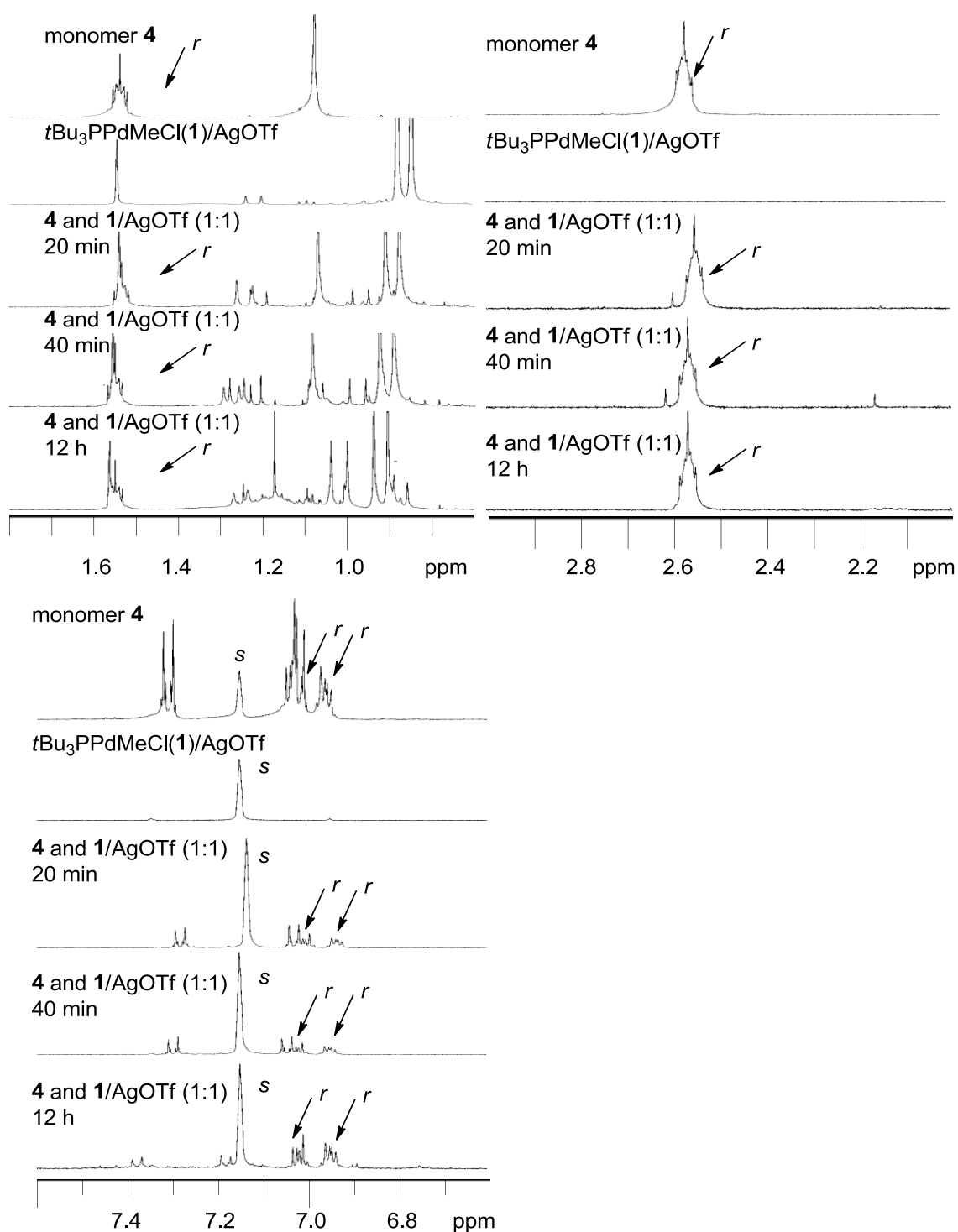
Figure 9. Expansion of key regions in the ^1\text{H} NMR spectra shown in Figure 8. Detailed reaction conditions are displayed in Scheme 4 and the experimental section. The spectra were measured at 50^\circ\text{C} in \text{C}_6\text{D}_6 (s: solvent; r: 1,2,3,4-tetrahydronaphthalene).
