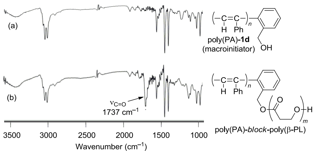
Figure 6. IR spectra of (a) macroinitiator, poly(PA)-1d, and (b) poly(PA)-block-poly( \beta -PL).
