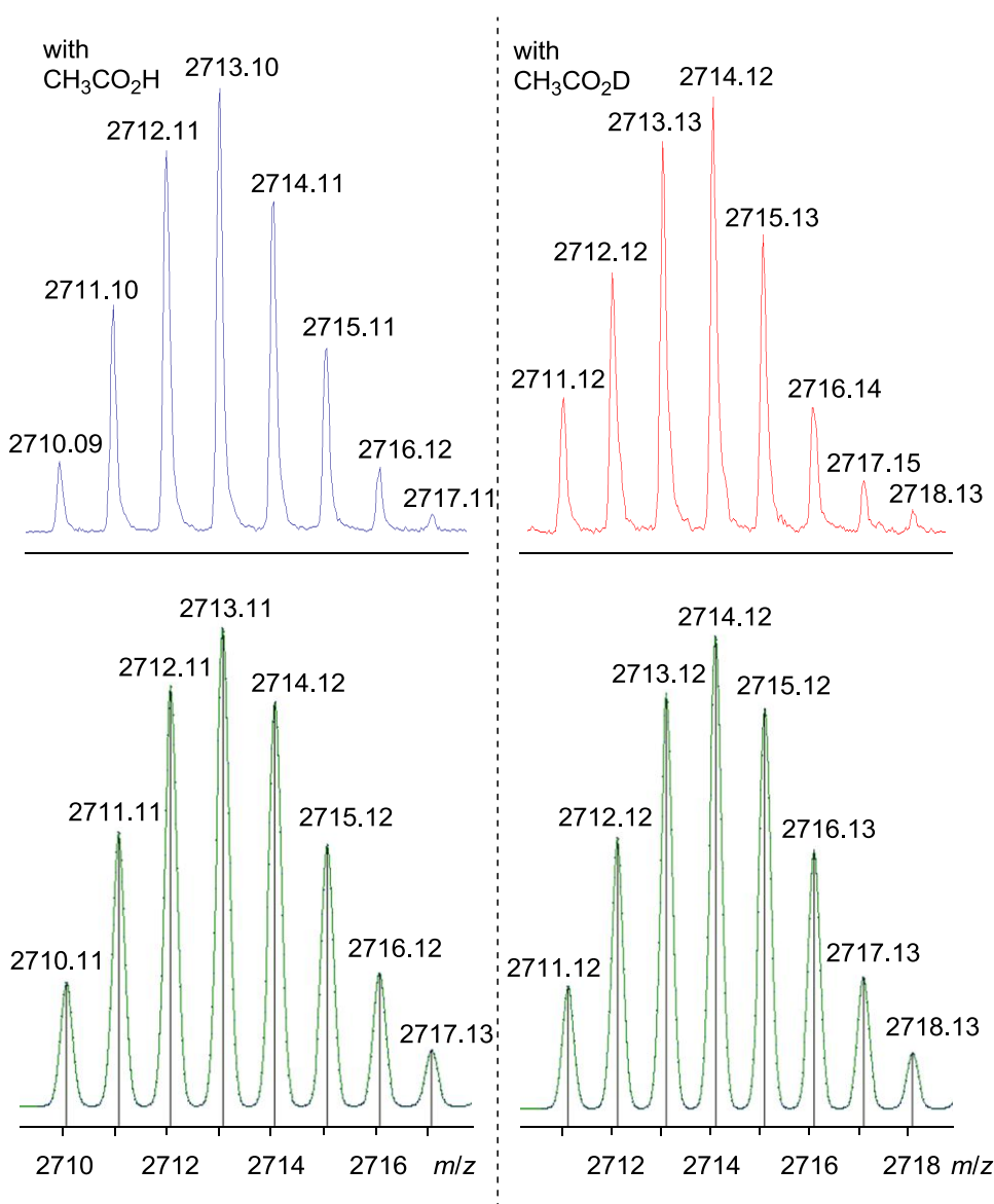
Figure 8. Isotope patterns of the observed (top) and calculated (bottom) MALDI-TOF mass spectra for poly(PA) quenched with \text{CH}_3\text{CO}_2\text{H} and \text{CH}_3\text{CO}_2\text{D} .
