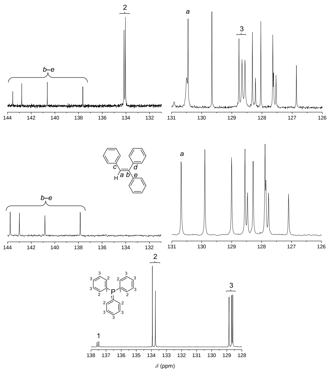
Figure 5. ^{13}\text{C} (100 MHz) NMR spectra of a mixture of 1 and 100 equiv of \text{CH}_3\text{CO}_2\text{H} ( [\mathbf{1}]_0 = 2.55 \times 10^{-2} \text{ M} ) (upper), triphenylethylene (middle), and \text{PPh}_3 (bottom) measured in \text{CD}_2\text{Cl}_2 .
