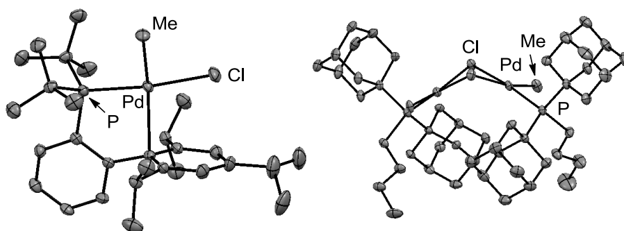
Figure 1. ORTEP drawing of 2 (left) and 3 (right). The thermal ellipsoids were set at 50% probability.
