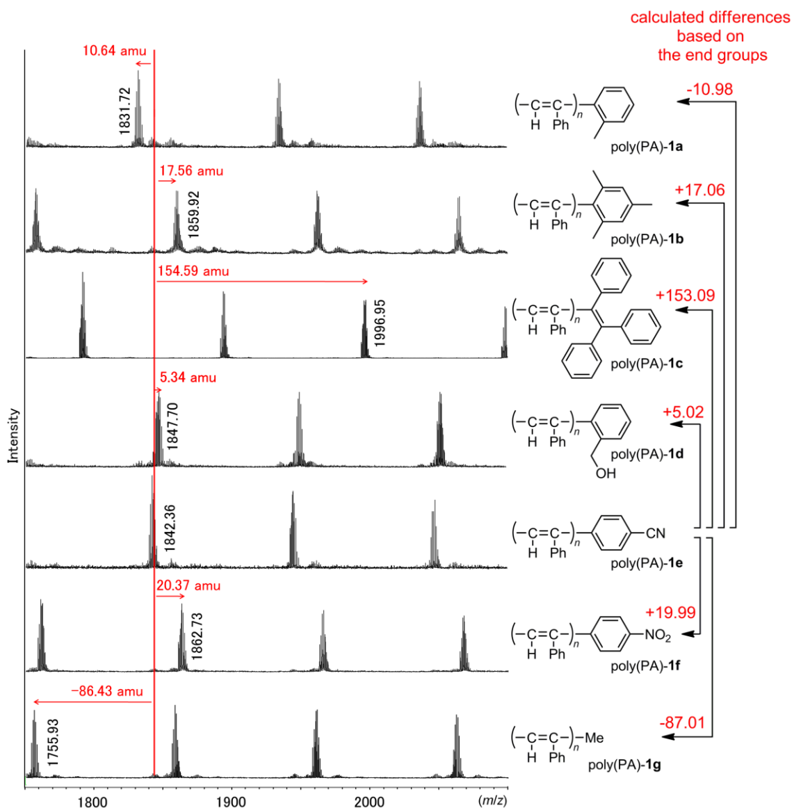
Figure 4. Relationship between mass peak differences and the end groups of the poly(PA)s in the MALDI-TOF mass spectra.
