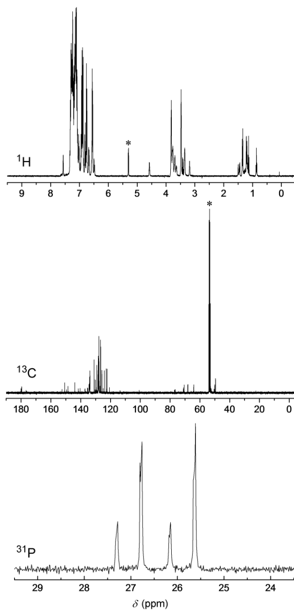
Figure 1. ^1\text{H} (400 MHz), ^{13}\text{C} (100 MHz) and ^{31}\text{P} (162 MHz) NMR spectra of 1 measured in \text{CD}_2\text{Cl}_2 ( [\mathbf{1}] = 2.55 \times 10^{-2} \text{ M} ) at room temperature. * indicates the solvent.
