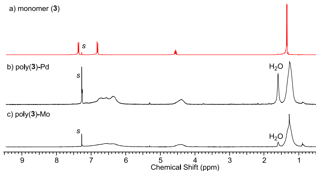
Figure 2. ^1\text{H} NMR spectra of: a) monomer 3 ; b) poly( 3 ) synthesized by the polymerization using t\text{Bu}_3\text{PPdMeCl} ( 6 )/AgOTf (Table 1, entry 5) and, c) poly( 3 ) synthesized using \text{MoCl}_5/\text{SnBu}_4 (Table 1, entry 6) measured in \text{CDCl}_3 at room temperature (s: solvent).
