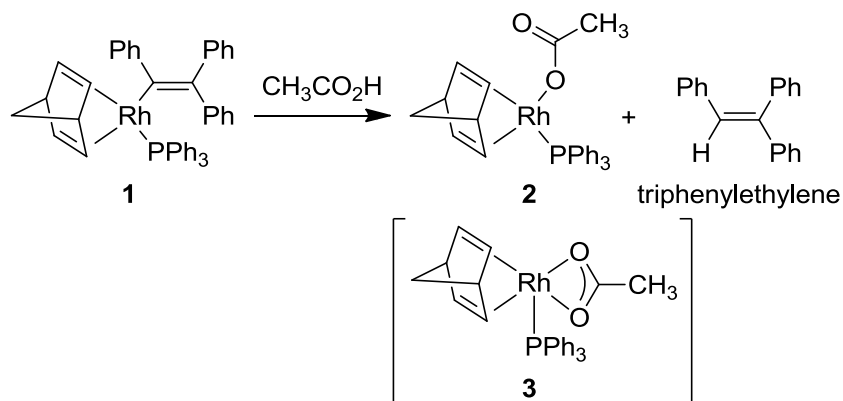
Scheme 1. Reaction of 1 with CH 3 CO 2 H
