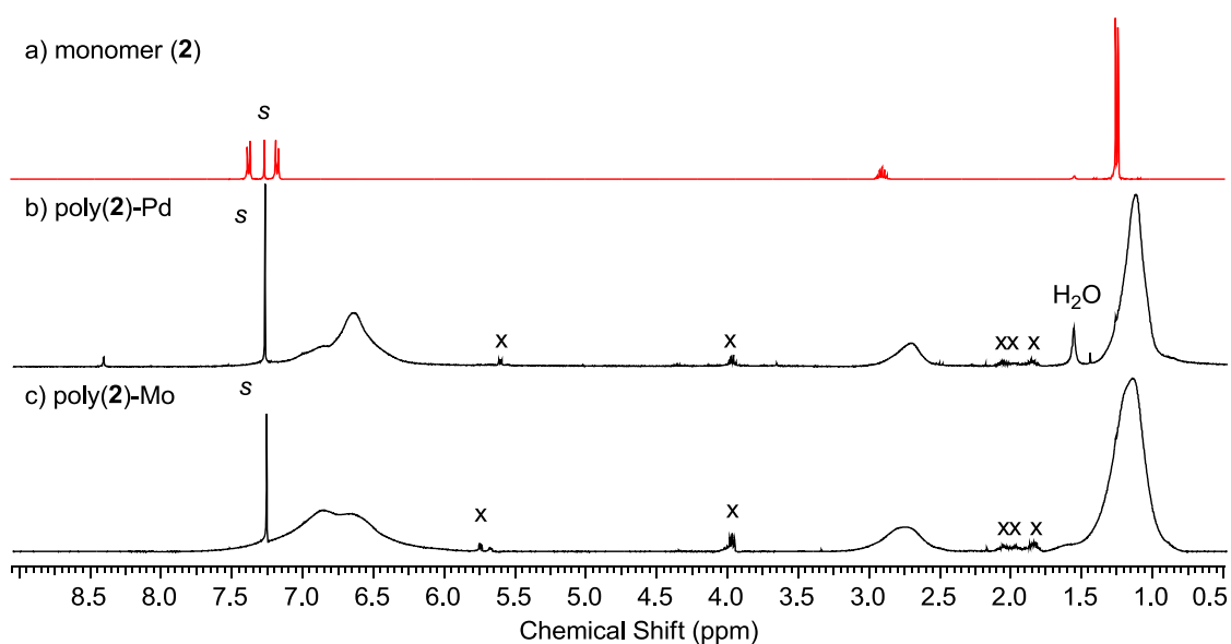
Figure 1. ^1\text{H} NMR spectra of: a) monomer 2 ; b) poly( 2 ) synthesized by the polymerization using t\text{Bu}_3\text{PPdMeCl} ( 6 )/AgOTf (Table 1, entry 3) and, c) poly( 2 ) synthesized using \text{MoCl}_5/\text{SnBu}_4 (Table 1, entry 4). All spectra were measured in \text{CDCl}_3 at room temperature (s: solvent, x: impurity).
