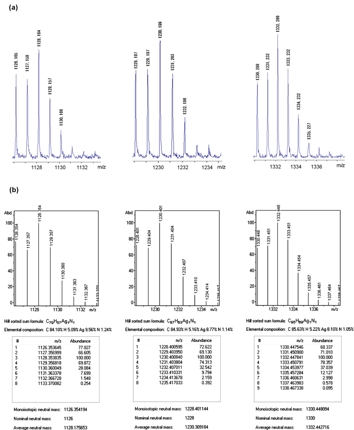
Figure 5. The results of (a) MALDI-TOF mass spectra of poly(PA)- 1e and (b) the simulated isotope patterns of an Ag^+ adduct of poly(PA) terminated with a phenylethynyl and a p -cyanophenyl group at polymer chain ends [thus, PhC\equiv C-(CH=CPh)_n-C_6H_4-p-CN ]. From left to right, the three sets of peaks correspond to the polymers with n = 8, 9 , and 10 , respectively. The simulated isotope patterns of the Ag^+ adducts appear fitting to the data actually measure
