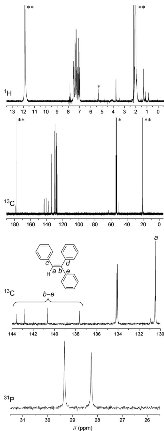
Figure 4. ^1\text{H} (400 MHz), ^{13}\text{C} (100 MHz) and ^{31}\text{P} (162 MHz), NMR spectra of a mixture of 1 and 100 equiv of \text{CH}_3\text{CO}_2\text{H} measured in \text{CD}_2\text{Cl}_2 ( [\mathbf{1}]_0 = 2.55 \times 10^{-2} \text{ M} ). *: Solvent. **: \text{CH}_3\text{CO}_2\text{H} . No change was observed between spectra of the samples recorded immediately after mixing of the reagents, or spectra that were acquired one day later.
