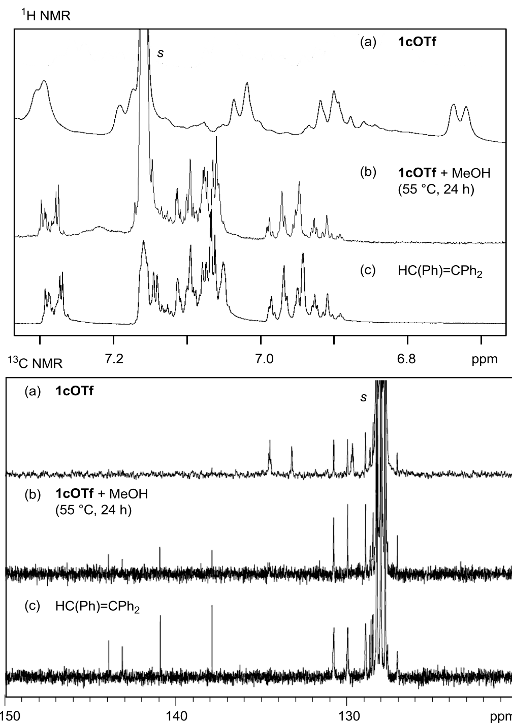
Figure 1. 1 H and 13 C NMR spectra of (a) 1cOTf , (b) 1cOTf + 50 equivalents of MeOH after heating at 55 °C for 24 h and (c) pure HC(Ph)=CPh 2 measured in CD 3 CN/C 6 D 6 = 1/3 (v/v), [ 1cOTf ] 0 = 25 mM at r.t. (s: solvent).
