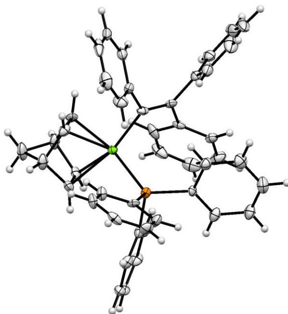
Figure 2. ORTEP drawing of molecular structure of 1 (50% probability ellipsoids).
