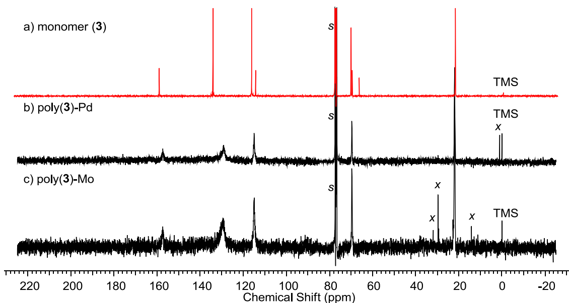
Figure 5. ^{13}\text{C} NMR spectra of: a) monomer 3 ; b) poly( 3 ) synthesized by the polymerization using t\text{Bu}_3\text{PPdMeCl} ( 6 )/AgOTf (Table 1, entry 5) and, c) poly( 3 ) synthesized by \text{MoCl}_5/\text{SnBu}_4 (Table 1, entry 6) measured in \text{CDCl}_3 at room temperature (s: solvent, x: impurity).
