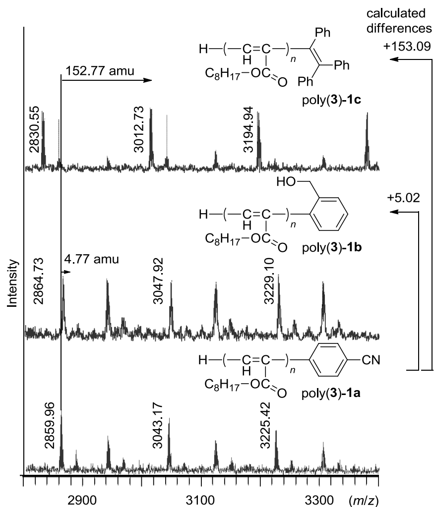
Figure 5. Comparison between the MALDI-TOF mass spectra of the poly(3) series obtained by the polymerizations initiated with 1a , 1b and 1c .
