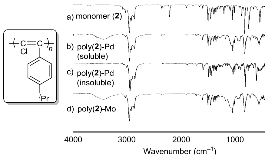
Figure 6. IR spectra of: a) monomer 2 ; b) poly( 2 ) synthesized by the polymerization using t Bu 3 PPdMeCl ( 6 )/AgOTf (Table 1, entry 3), c) insoluble fraction of poly( 2 ) synthesized using t Bu 3 PPdMeCl ( 6 )/AgOTf (Table 1, entry 3) and, d) poly( 2 ) synthesized using MoCl 5 /SnBu 4 (Table 1, entry 4) measured by the KBr pellet method.
