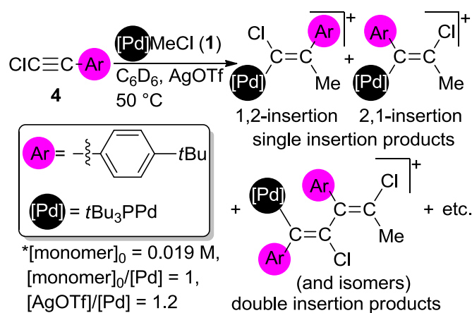
Scheme 4. Stoichiometric reaction between 1 /AgOTf and 4 (1:1). The counteranion ( \text{OTf}^- ) was omitted for clarity.
