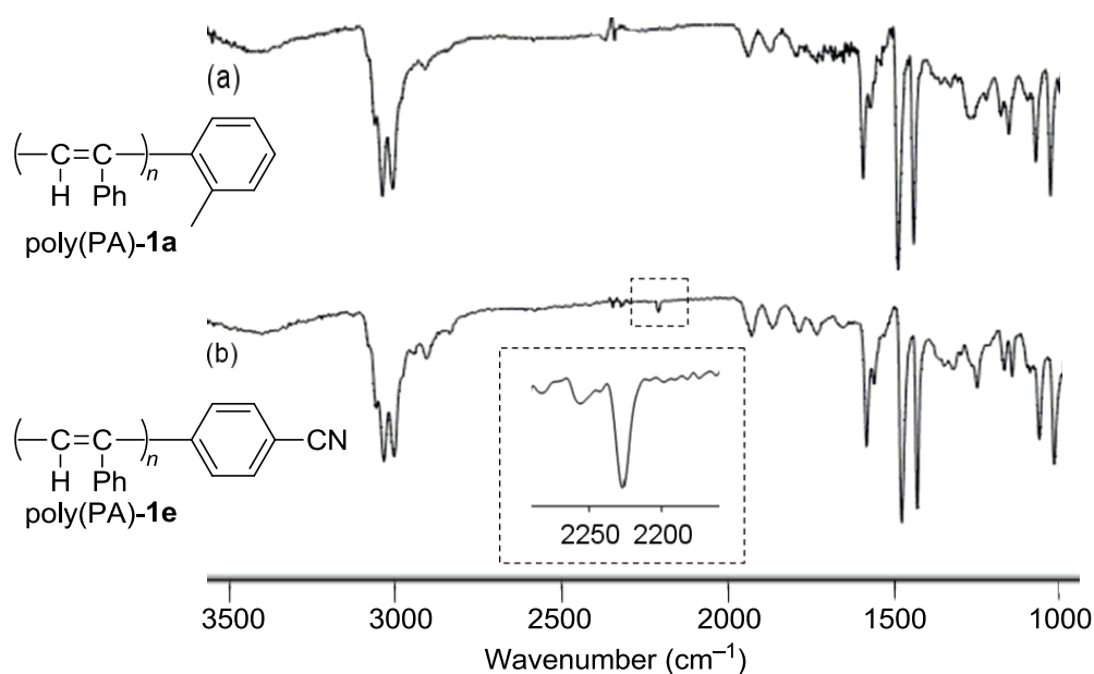
Figure 2. IR spectra of (a) poly(PA)- 1a and (b) poly(PA)- 1e .
