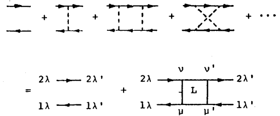
Fig. 1. Diagrams for \mathcal{H}_{\mathbf{p}\lambda, \mathbf{p}'\lambda'}^a(\omega_m, \varepsilon_n) . The full lines refer to \mathcal{S}_{\lambda\lambda'}^{\alpha\beta}(\mathbf{p}, \varepsilon_n) , where index 1 or 2 at the end of lines represent upper suffix \alpha, \beta of \mathcal{S}_{\lambda\lambda'}^{\alpha\beta} ; the dotted lines refer to quantities like n_i u_{\mathbf{p}\lambda, \mathbf{p}'\lambda'}^2 . The arrows on the phonon lines are drawn in order to perform our calculations in the same way as that for particle system.
