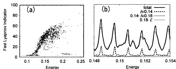
Figure 1: (a)Relation of FLI and trajectory energy. (b)Decomposition of spectrum.
