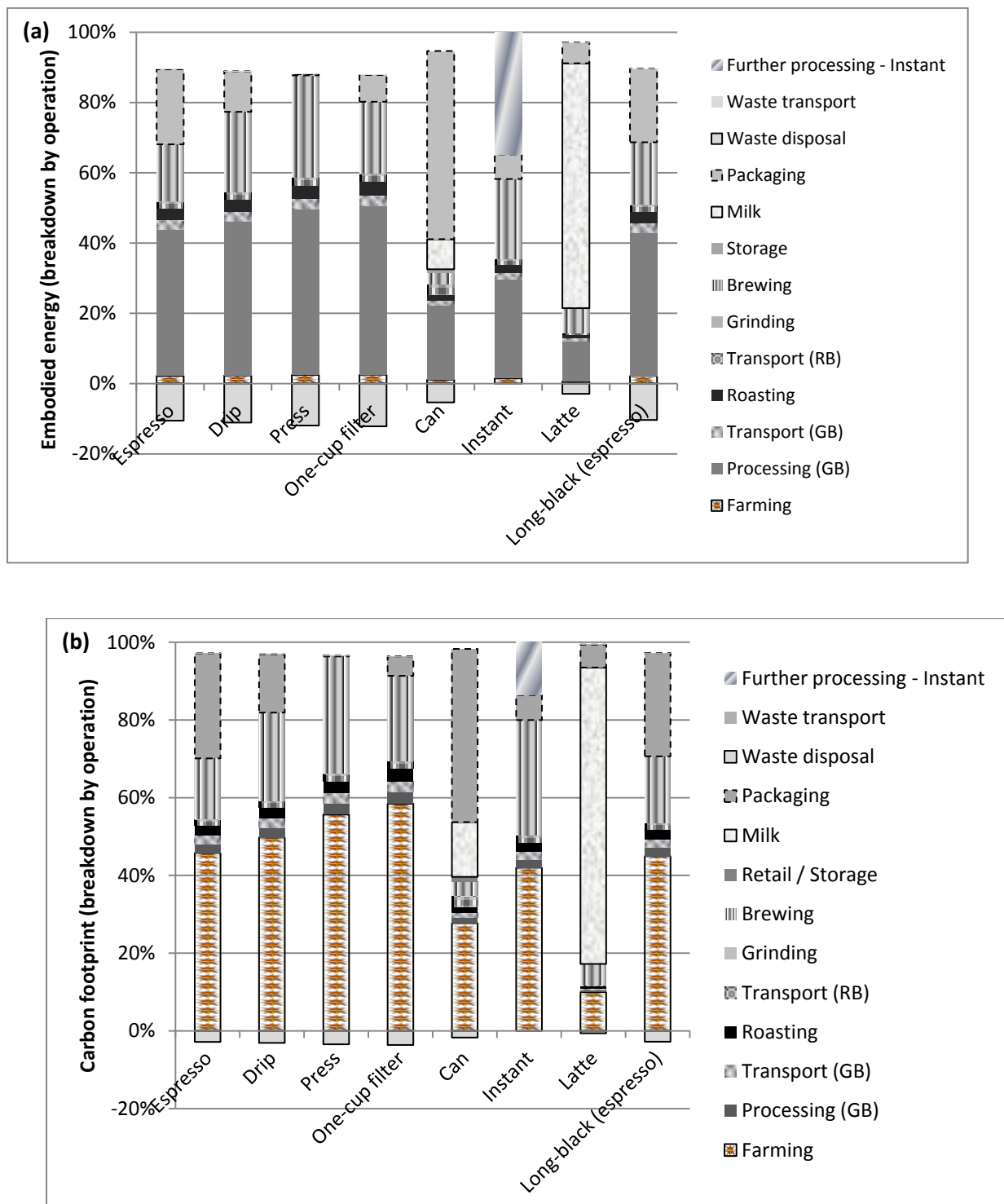
Figure 5: Breakdown by operation for (a) Embodied energy and (b) carbon footprint of alternative coffee products
