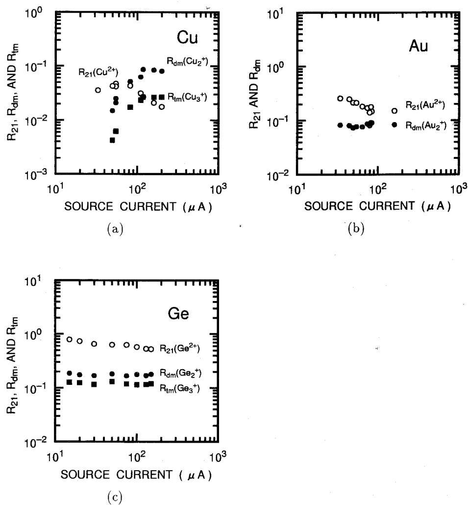
Figure 2.14: Relative currents of molecular ions as a function of I_s . (a) Cu, (b) Au, and (c) Ge ion sources.
