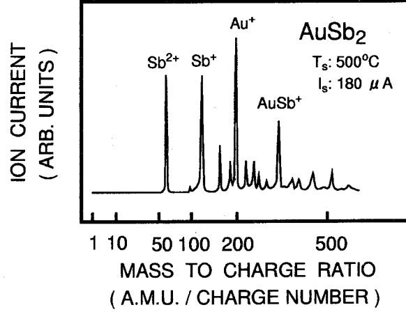
Figure 4.9: Typical mass spectrum of AuSb 2 ion source.
