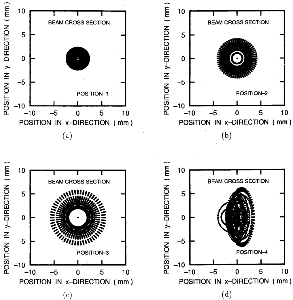
Figure 5.14: Calculated cross-section of the beam with energy spread of \pm 100 eV. V_{\text{pre}}=18 kV, and V_{\text{post}}=14 kV.
