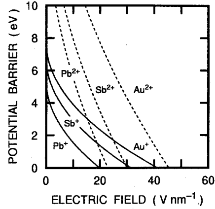
Figure 4.15: Potential barrier for element Pb, Au, and Sb. Image hump model was used to calculate the barrier.
