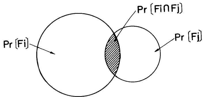
Fig. 4.3 Probability of Two-Events-Occurrence
