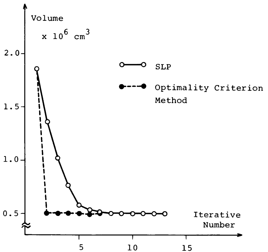
Fig. 3.19 Comparison of Optimality Criterion Method and SLP
