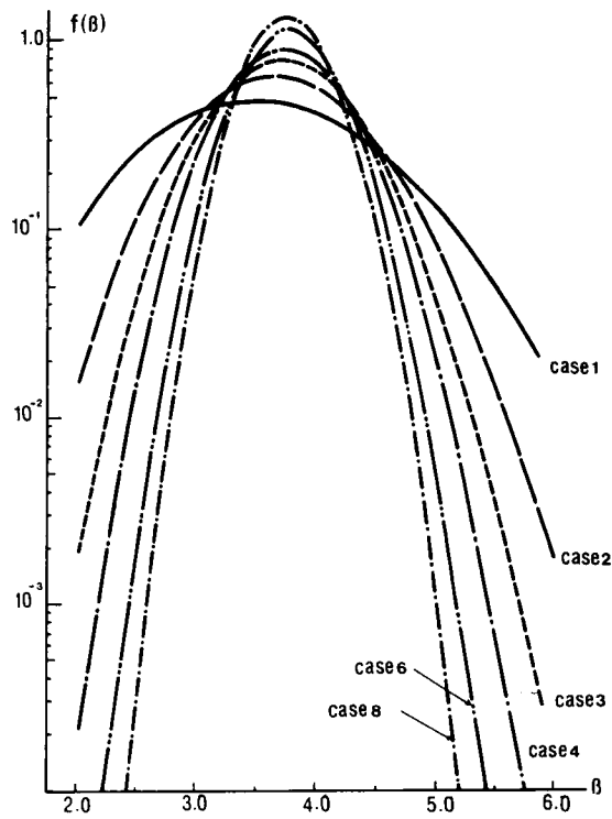
Fig. 5.1 Probability Density Function of Saset Index
