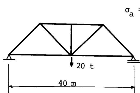
Fig. 2.19 Pratt Truss and Warren Truss
