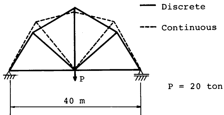
Fig. 2.25 Optimal Configuration of Truss with Discrete Components
