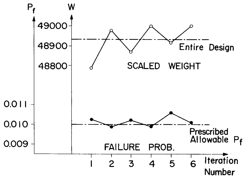
Fig. 4.18 Convergence of Decomposition Method
