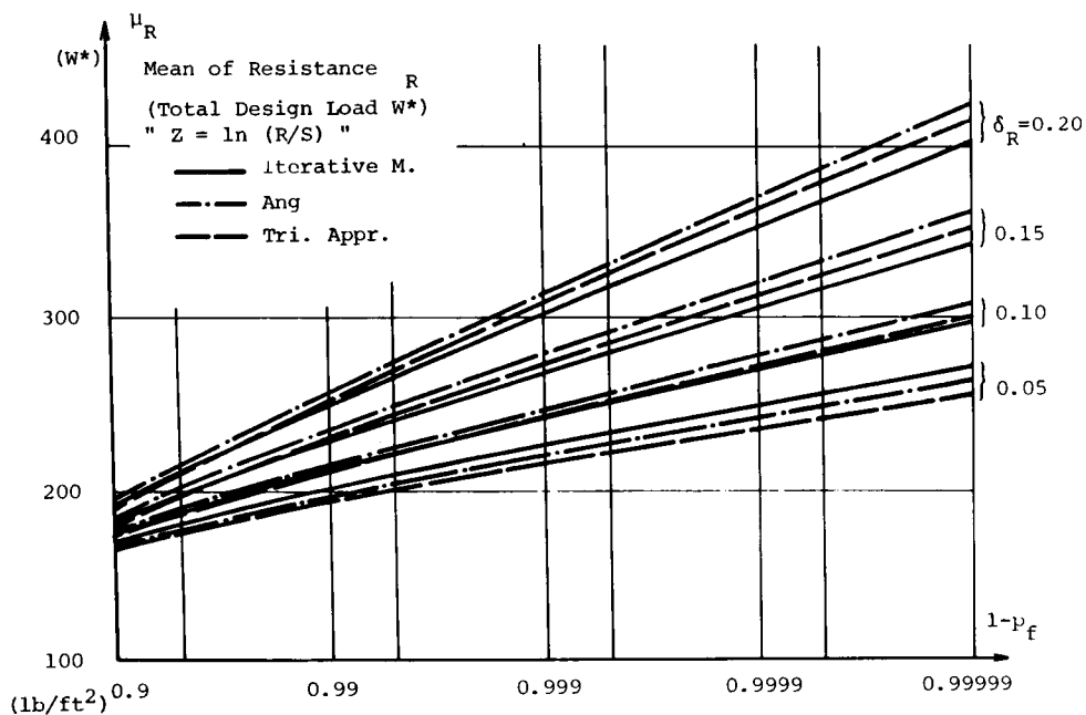
Fig. 6.6 Mean Value of Resistance ( Z = ln ( R/S ) )
