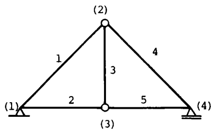
Fig. 2.4 Triangular Truss
