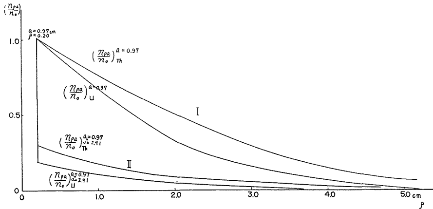
Fig. 1. Theoretical values of (n_{\rho a}/n_0)_U and (n_{\rho a}/n_0)_{Th} as a function of \rho .
