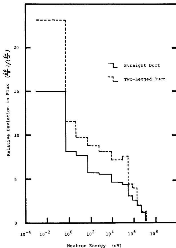
Fig.5 Flux deviation introduced by the 10% deviation in the total albedo data in all groups.
