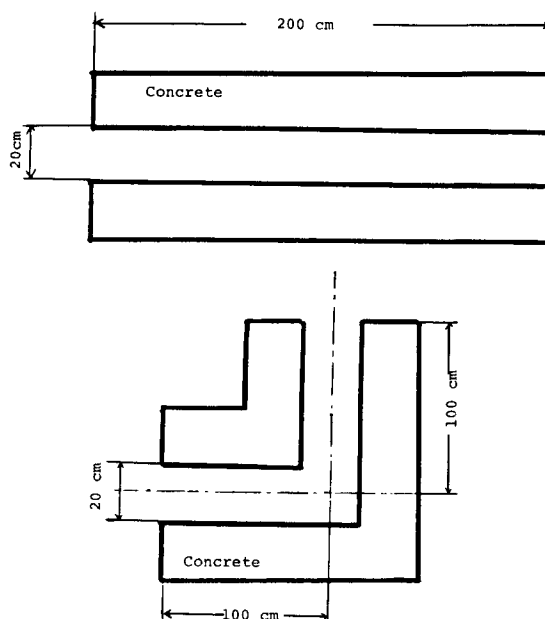
Fig.1 Concrete duct arrangements for the test calculation.
