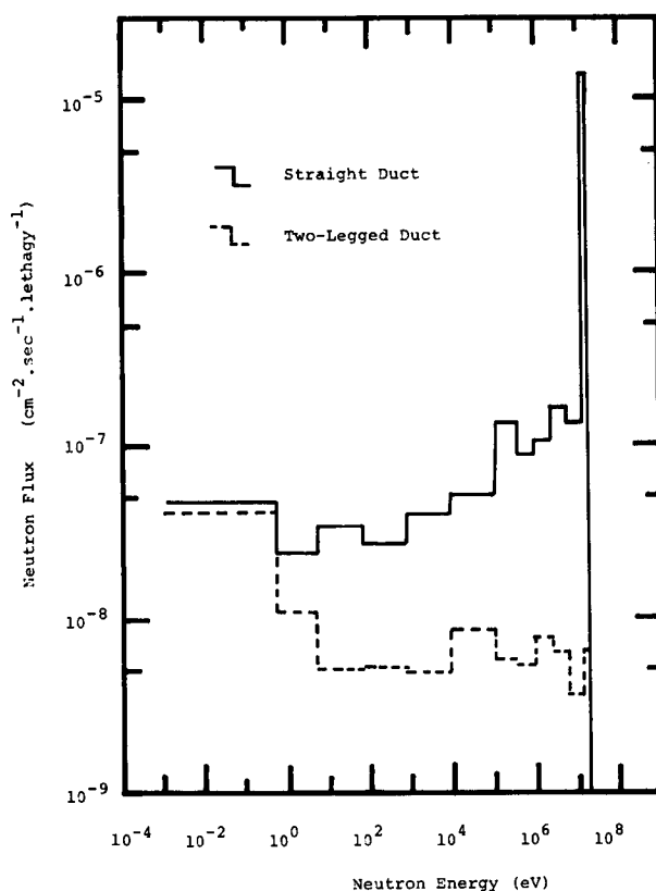
Fig.2 Results of the albedo Monte Carlo calculation.
