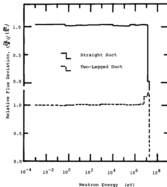
Fig.3 Flux deviation caused by the 10% deviation in the total albedo data of the 1st group.
