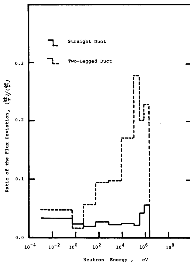
Fig.4 Flux deviation due to the 10% deviation in the total albedo data in the 4th group.
