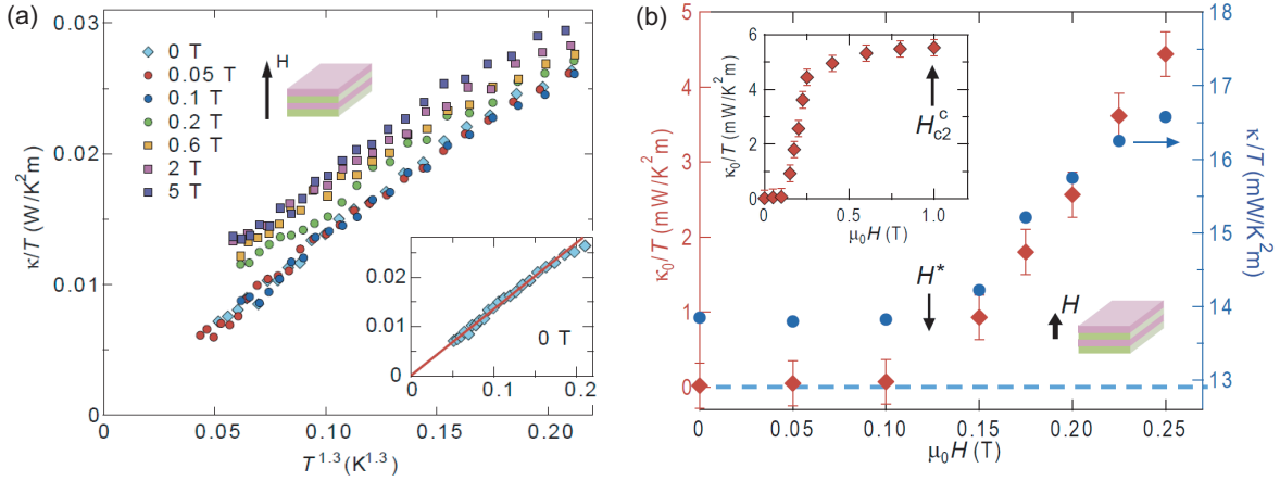
Figure 3.5: (a) Thermal conductivity divided by temperature \kappa/T of \text{NdO}_{0.71}\text{F}_{0.29}\text{BiS}_2 plotted against T^{1.3} in several magnetic fields applied parallel to the c -axis. Inset: \kappa/T vs T^{1.3} in zero field. The solid line represents a linear fit to the data below 0.3 K [33]. (b) Field dependence of the residual linear term \kappa_0/T (red diamonds) and \kappa/T at T = 170 mK (blue circles) for \mathbf{H} \parallel c . The residual term \kappa_0(H)/T is determined by fitting \kappa(T)/T at different fields below 0.3 K with \kappa_0/T + aT^{1.3} , where \kappa_0/T and a are fitting parameters. Both \kappa_0/T and \kappa/T at T = 170 mK are independent of the magnetic field up to H^* . Inset shows \kappa_0/T in an extended field range. The superconducting upper critical field along c -axis H_{c2}^c is determined by the field dependence of the electrical resistivity at 0.2 K [33].
