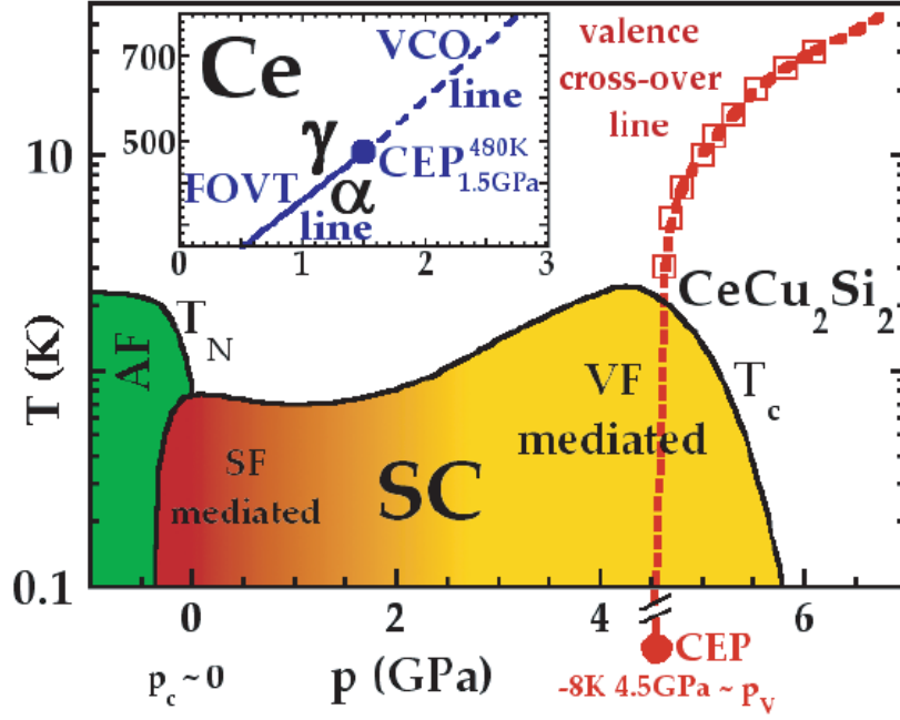
Figure 4.17: T - p phase diagram in pure \text{CeCu}_2\text{Si}_2 [113]. Valence crossover line and its critical end point (CEP) are determined by the pressure dependence of the resistivity data. T_c reaches its maximum at CEP. Inset shows the T - p phase diagram of elementary Ce. The first order valence transition (FOVT) line and the valence crossover (VCO) line have been determined by several measurements [115, 116].
