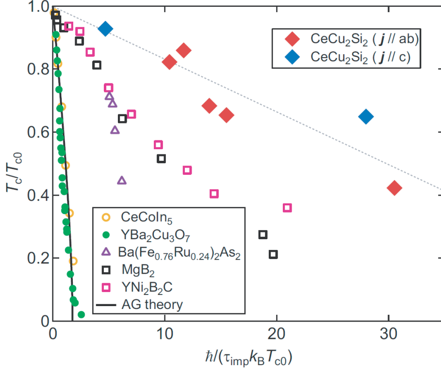
Figure 5.8: Comparison of impurity effect of \text{CeCu}_2\text{Si}_2 with those of other superconductors. Suppression of superconducting transition temperature T_c/T_{c0} as a function of dimensionless scattering rate \hbar/\tau_{\text{imp}}k_B T_{c0} , where \tau_{\text{imp}} is the impurity scattering time estimated from residual resistivity \rho_0 and the penetration depth, \tau_{\text{imp}} = \mu_0\lambda_{ab}\lambda_c/\rho_0 . The solid line shows the prediction of the Abrikosov-Gorkov (AG) theory for an isotropic s -wave superconductor with magnetic impurities. We also plot the data for Sn-substituted \text{CeCoIn}_5 ( d -wave) [22], electron-irradiated \text{YBa}_2\text{Cu}_3\text{O}_{7-\delta} ( d -wave) [138], electron-irradiated \text{Ba}(\text{Fe}_{0.76}\text{Ru}_{0.24})_2\text{As}_2 (possibly s_{\pm} -wave) [141], and neutron-irradiated \text{MgB}_2 [139] and \text{YNi}_2\text{B}_2\text{C} [140]. The value of T_{c0} is estimated by extrapolating two initial data points to zero 1/\tau_{\text{imp}} limit. Rather weak pair-breaking effect in \text{Ba}(\text{Fe}_{0.76}\text{Ru}_{0.24})_2\text{As}_2 has been attributed to a large imbalance between intra- and inter-band scattering [141]. For \text{MgB}_2 data, we use the value of \lambda_{ab}(0) = \lambda_c(0) = 100 \text{ nm} [142]. For \text{YNi}_2\text{B}_2\text{C} data, we use \lambda_{ab}(0) = 110 \text{ nm} [143] and \lambda_c(0) = \lambda_{ab}(0)H_{c2}^{ab}/H_{c2}^c = 140 \text{ nm} [144], where H_{c2}^{ab} and H_{c2}^c are upper critical field parallel and perpendicular to the ab plane.
