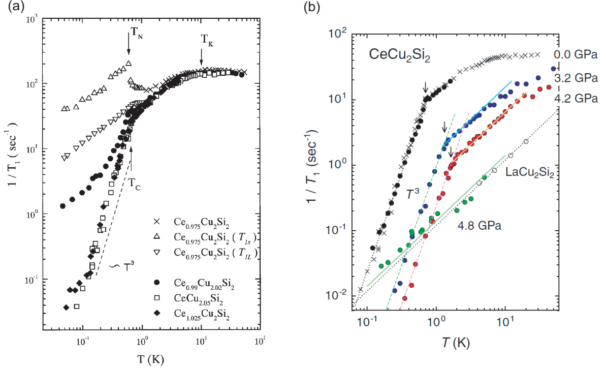
Figure 4.20: (a) 1/T_1 vs T in polycrystalline \text{Ce}_x\text{Cu}_{2+y}\text{Si}_2 at ambient pressure [106]. \text{CeCu}_{2.05}\text{Si}_2 and \text{Ce}_{1.025}\text{Cu}_2\text{Si}_2 exhibit superconductivity below T_c . T_N and T_K denote the AFM transition temperature and Kondo temperature, respectively. (b) 1/T_1 vs. T under several pressures in polycrystalline \text{CeCu}_{2.05}\text{Si}_2 [117].
