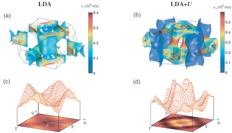
Figure 4.4: The Fermi surface of CeCu 2 Si 2 calculated by (a), (c) LDA calculations [86] and (b), (d) the renormalized band method [87].
