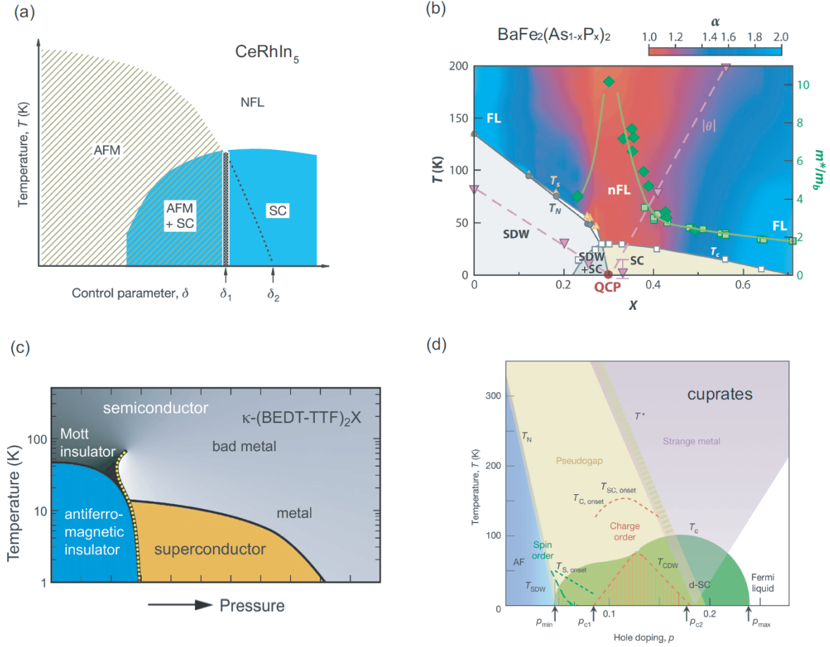
Figure 1.1: Phase diagram of several strongly correlated materials. (a) heavy-fermion superconductor CeRhIn 5 [8], (b) Fe-pnictide BaFe 2 (As 1-x P x ) 2 [9], (c) organic \kappa -(BEDT-TTF) 2 X [10] and (d) high- T_c cuprates [11].
