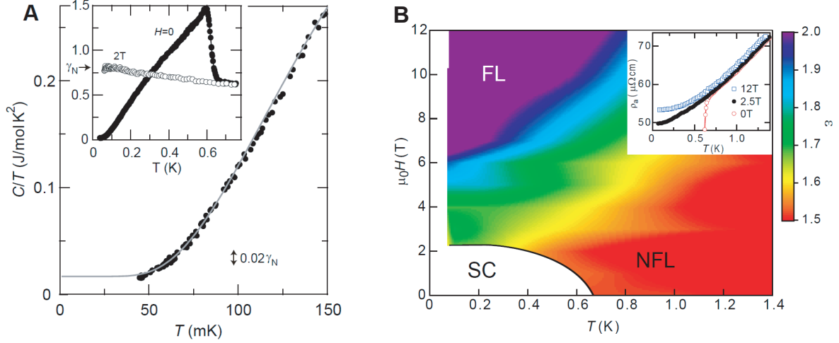
Figure 5.3: (A) Inset shows the specific heat divided by temperature C/T in zero field and in the normal state at \mu_0 H = 2\text{ T} for \mathbf{H} \parallel ab plane. The main panel shows C/T at low temperatures. The gray solid line is an exponential fit of the data, yielding \Delta = 0.39\text{ K} . (B) H - T phase diagram with color-coding of T -exponent ( \epsilon ) of the in-plane electrical resistivity, \rho(T) = \rho_0 + AT^\epsilon for \mathbf{H} \parallel c . Inset shows the T -dependence of \rho(T) in zero field and in magnetic fields of 2.5 and 12 T applied along the c axis.
