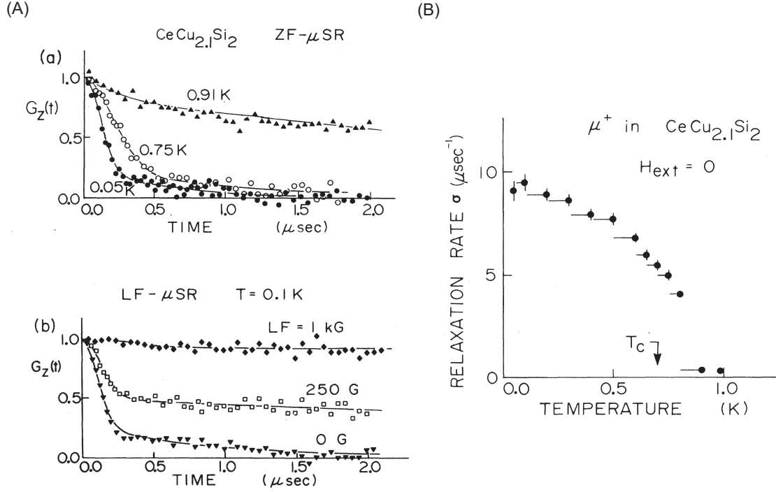
Figure 4.7: \mu\text{SR} measurements on a polycrystalline sample of \text{CeCu}_{2.1}\text{Si}_2 . (A) Muon-spin-relaxation function G_z(t) (a) in zero field and (b) at T = 0.1\text{ K} in longitudinal external fields. (B) Muon-spin-depolarization rate \sigma vs. T in zero field [91].
