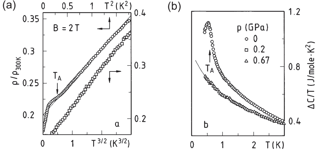
Figure 4.13: (a) \rho/\rho_{300K} vs. T^2 (upper scale) and \rho/\rho_{300K} vs. T^{3/2} (lower scale), (b) \gamma vs T at B = 2 T and at p = 0, 0.2 , and 0.67 GPa in an A -type \text{CeCu}_2\text{Si}_2 polycrystal [100].
