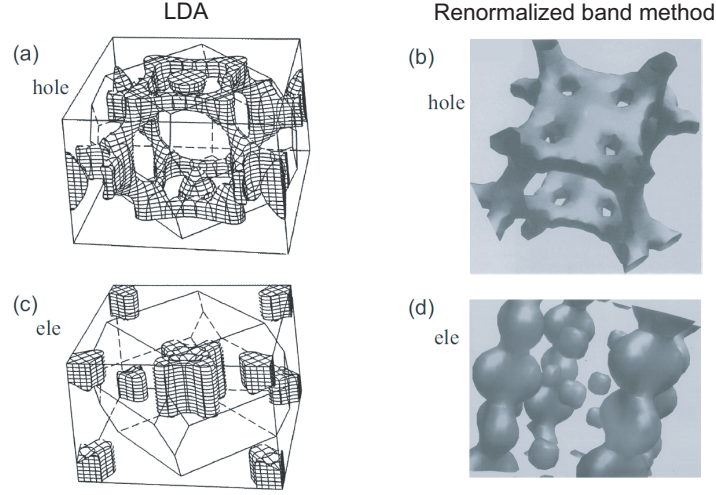
Figure 4.4: The Fermi surface of CeCu 2 Si 2 calculated by (a), (c) LDA calculations [86] and (b), (d) the renormalized band method [87].
