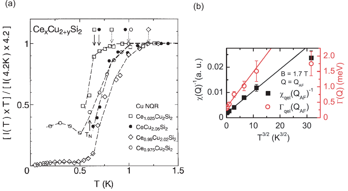
Figure 4.15: (a) Cu-NQR intensity multiplied by temperature I \times T vs T normalized by I \times T at 4.2 K in polycrystal \text{Ce}_x\text{Cu}_{2+y}\text{Si}_2 [106]. \text{CeCu}_{2.05}\text{Si}_2 and \text{Ce}_{1.025}\text{Cu}_2\text{Si}_2 exhibit bulk superconductivity. Dotted and solid arrows indicate T_m and T_c , respectively. (b) Neutron scattering results for Q = Q_{\text{AF}} at B = 1.7 T [107]. \chi^{-1}(Q_{\text{AF}}) vs T^{3/2} (black symbols) and \Gamma(Q_{\text{AF}}) vs. T^{3/2} (red symbols) in the normal state. The small residual value at T = 0 is due to the fact that this sample is slightly away from the AF QCP.
