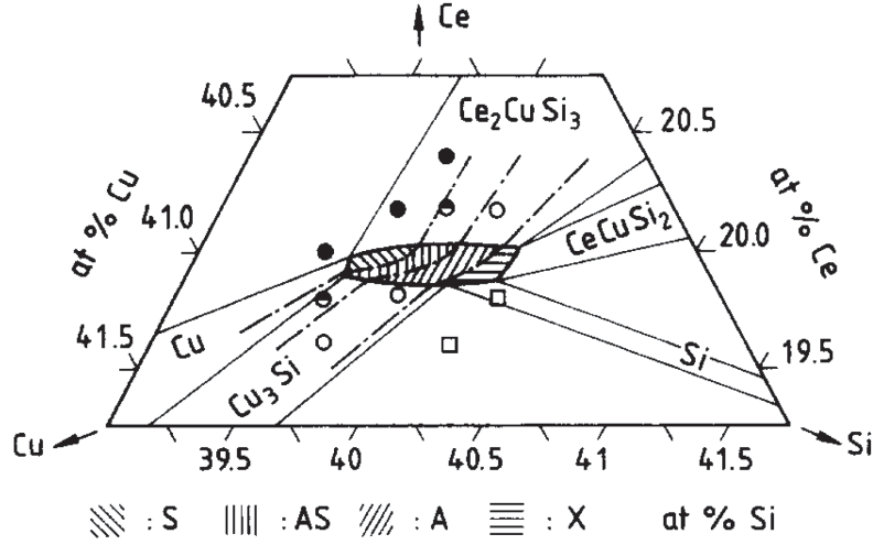
Figure 4.3: The ternary phase diagram for various Ce : Cu : Si compositions (dashed: \text{CeCu}_2\text{Si}_2 homogeneity range) [84]. “A” (○), “S” (●), and “A/S” (circle with upper half black) represent the antiferromagnetic order phase, superconducting phase, and competition phase between them, respectively.
