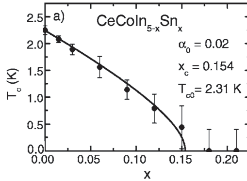
Figure 1.7: Superconducting transition temperature T_c vs. Sn doping x of the d -wave superconductor CeCoIn 5- x Sn x . The solid line represents the AG pair-breaking formula. Experimental results are well fitted by the AG formula [22].
