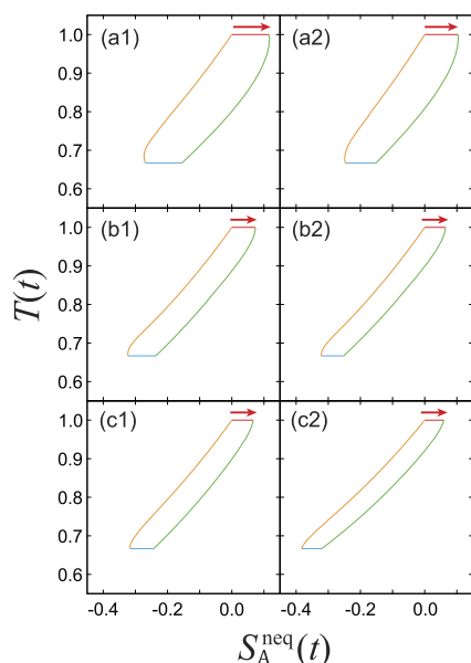
FIG. 4. T(t)-S_A^{\text{neq}}(t) diagrams for the thermostatic Stirling engine in the classical case (1, left column) and quantum case (2, right column) for (a) A = 0.5 (weak), (b) A = 1.0 (intermediate), and (c) A = 1.5 (strong) SB coupling strengths, respectively. Each cycle starts with a red arrow, and the four curves represent (i) hot isothermal (red), (ii) from hot to cold (green), (iii) cold isothermal (blue), and (iv) from cold to hot (orange) processes, respectively.
