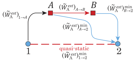
FIG. 7. Schematic for deriving the principle of DL non-equilibrium minimum work expressed by Eq. (B3). We consider two non-equilibrium states A and B (red square) that are connected by a non-equilibrium process described by the red arrow for A \rightarrow B . The light blue curves A \rightarrow 2 and B \rightarrow 2 represent non-equilibrium-to-equilibrium minimum work paths, whose work is denoted by (\tilde{W}_A^{ext})_{A \rightarrow 2}^{min} and (\tilde{W}_A^{ext})_{B \rightarrow 2}^{min} , respectively.
