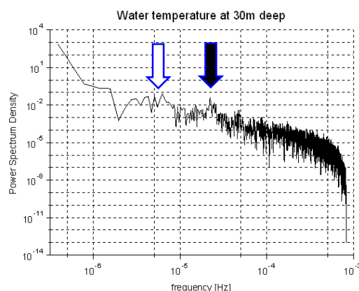
Fig.7 Frequency analysis of water temperature at 30m deep of the observation tower from Aug19 to Sep17
