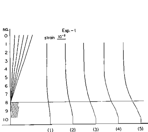
Fig. 2 Mud flow type slide; figures in brackets show accumulated strain values estimated from the variation of electrical resistance of strain gages.
