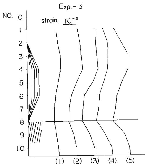
Fig. 4 Protruding of intermediate layer type; figures in brackets show accumulated strain values estimated from the variation of electric resistance of gages.
