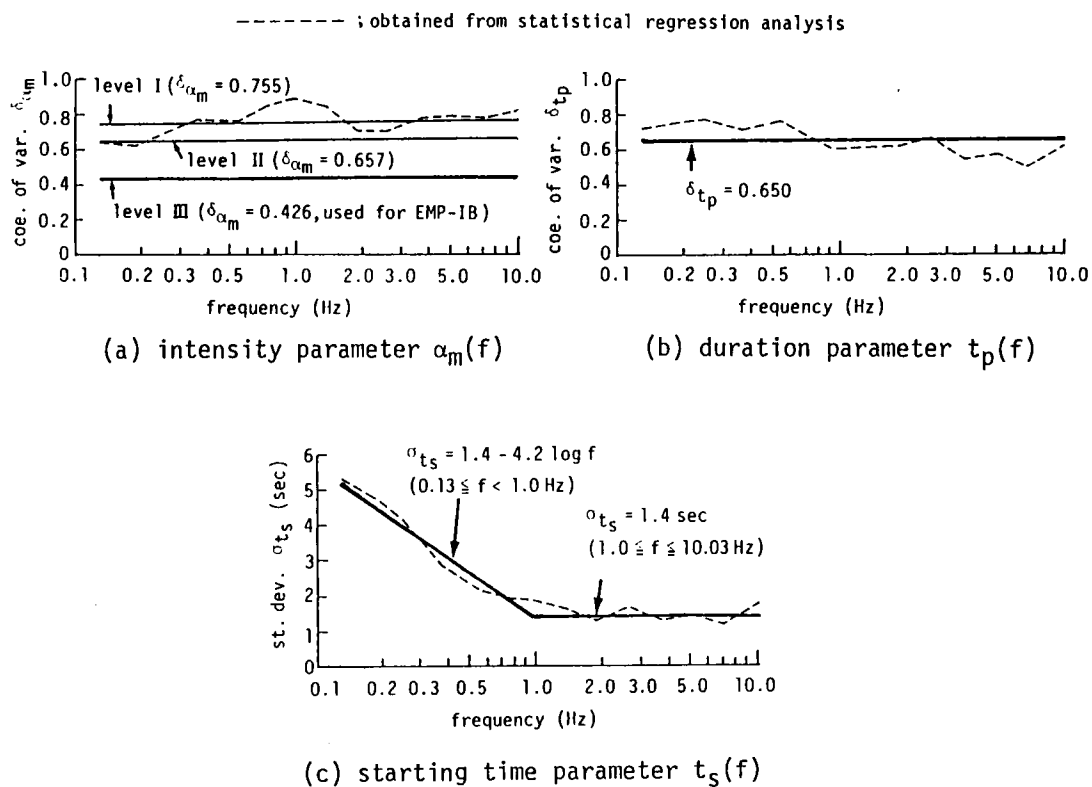
Fig.4.10 Characterization of Prediction Uncertainty for Model Parameters.
