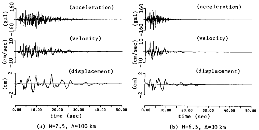
Fig.4.9 Simulated Rock Surface Motion for Combinations of Magnitude and Distance.
