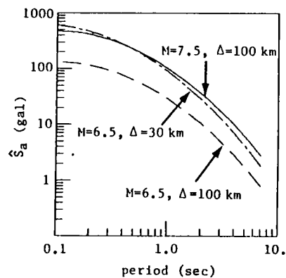
Fig.4.21 Modeled Acceleration Response Spectra for Combinations of Magnitude and Distance.
