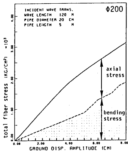
(2) transverse wave
