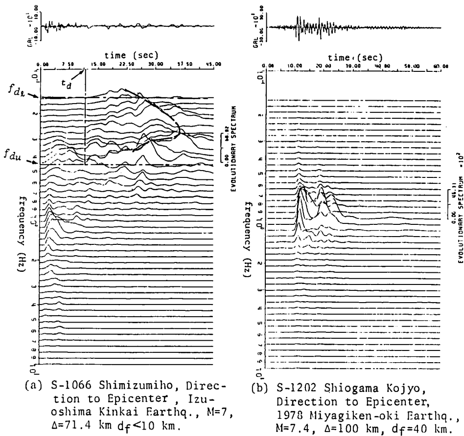
Fig.3.3 Typical Examples of Evolutionary Power Spectra.
