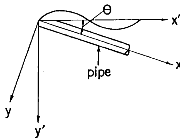
Fig.6.5 Buried Pipe and Horizontally Propagating Seismic Wave.
