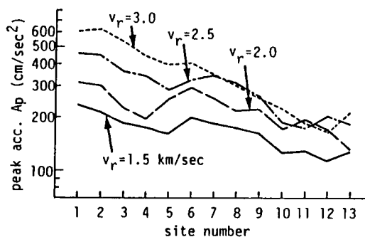
(a) peak acceleration A_p
