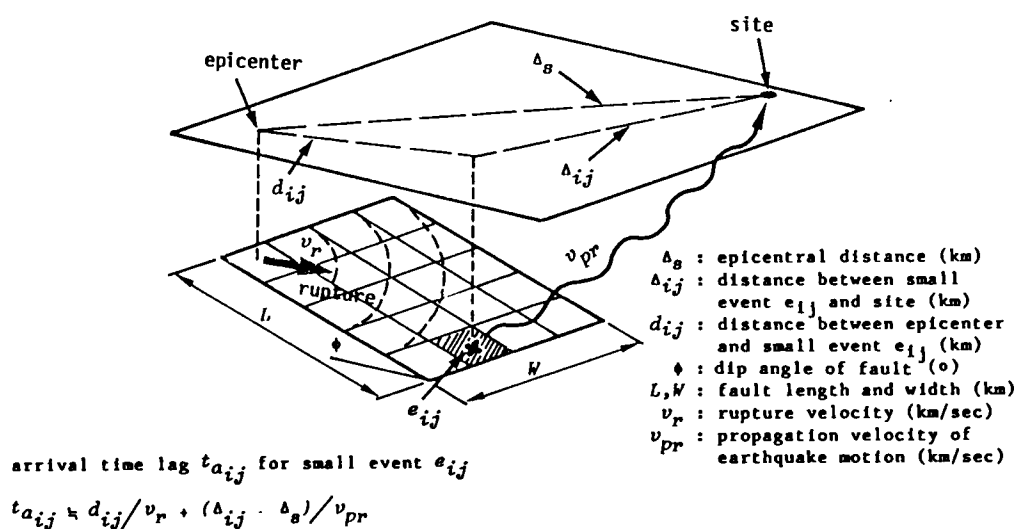
Fig.4.11 Fault Modeling with Multiple Fault Ruptures.
