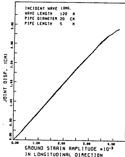
(2) joint displacement in fixed section
