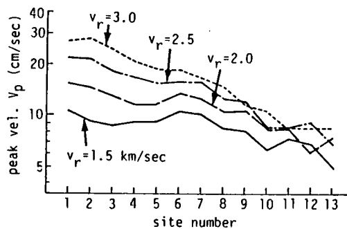
(b) peak velocity V_p
