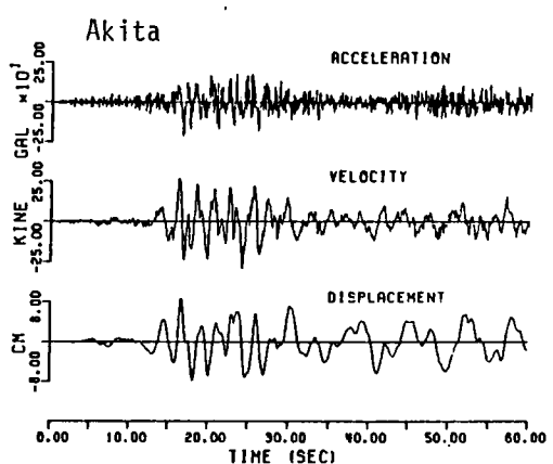
(c) recorded soil surface motion
