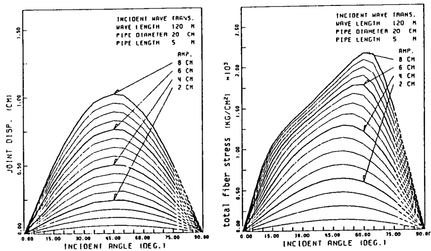
(2) transverse wave
