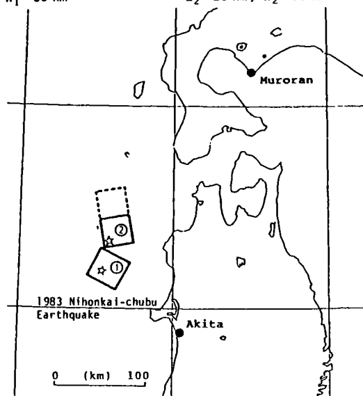
(a) Fault Model for the 1983 Nihonkai-chubu Earthquake (northwest Japan : M=7.7 , M_0=5.8 \times 10^{27} \text{ dyn-cm} )
