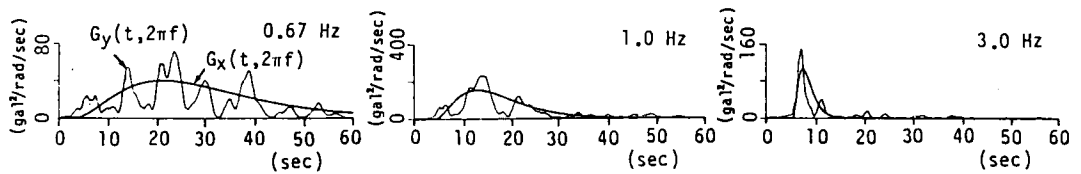
Fig.4.2 Recorded and Simulated Evolutionary Spectra (S-235 Aomori, 1968 Tokachi-oki Earthquake)
