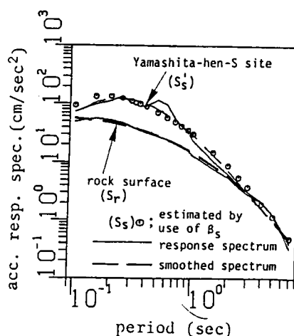
(b) M=6.0, Δ=120 km
