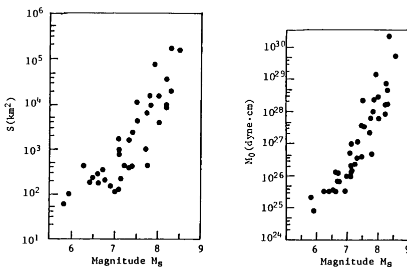
Fig.A-6 Relation between Surface Magnitude M_S , Fault Area S , and Seismic Moment M_0 (Ref.3).
