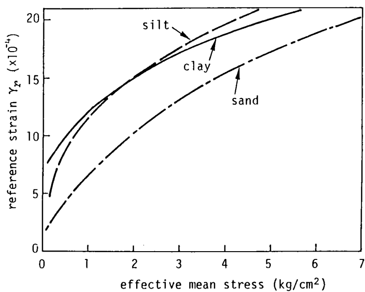
Fig.2.7 Relation between Reference Strain \gamma_r and Effective Mean Stress for Typical Soils(Ref.4).
