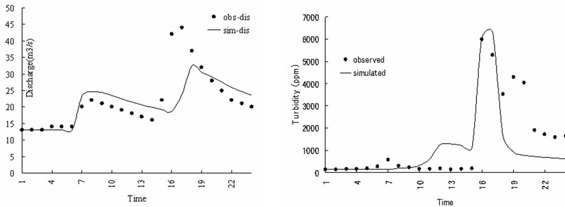
Fig. 6 Simulated and observed discharge and turbidity on 19 September 2005
