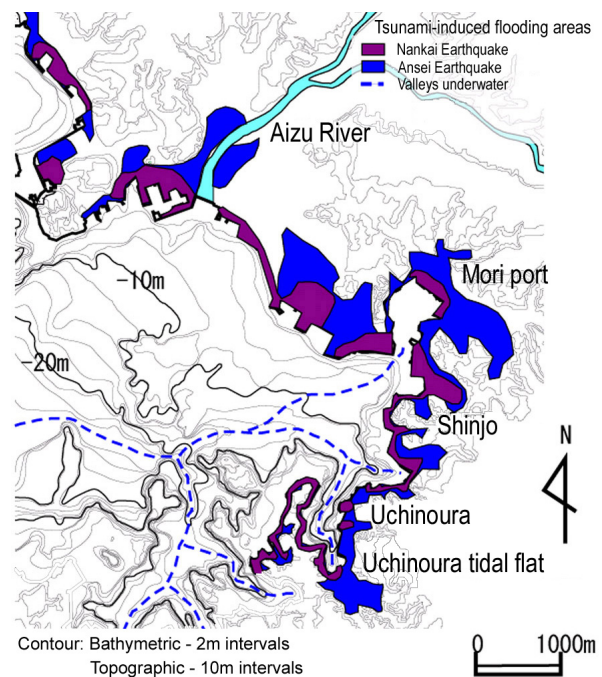
Fig. 27 Tsunami-induced inundation areas along Tanabe Bay
