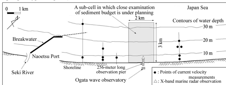
Fig. 16 A sketch showing the extent of Ogata coast with the location of 256-m long observation pier indicated
