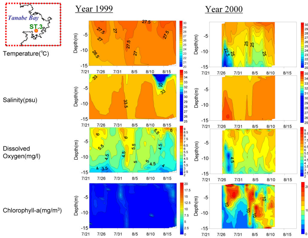
Fig. 25 Predicted performance of seawater temperature, salinity, dissolved oxygen and chlorophyll-a
