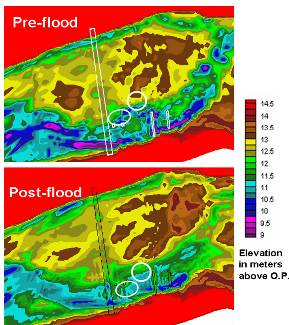
Fig. 13 Calculated evolution of bed topography (Zhang et al. 2007b)
