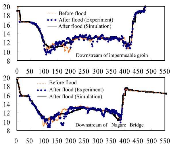
Fig. 14 Evolution of cross-channel profiles (Zhang et al, 2007b)
