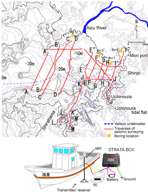
Fig. 28 Lines of seismic profiling performed with STRATA BOX mounted on KAISHO
