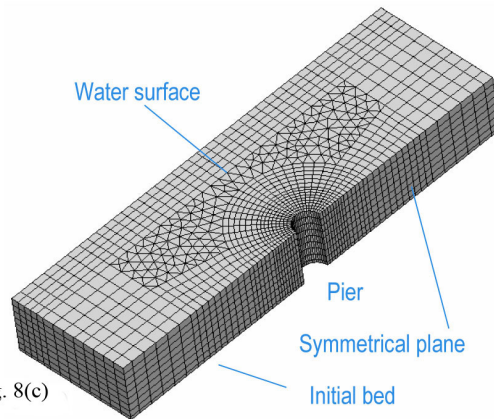
Fig. 8 (a) Experimental conditions for looking at local scour around a pier (after Melville & Raudkivi, 1977); (b) Plan view of a channel; (c) Computational mesh used by Zhang et al. (2007a)
