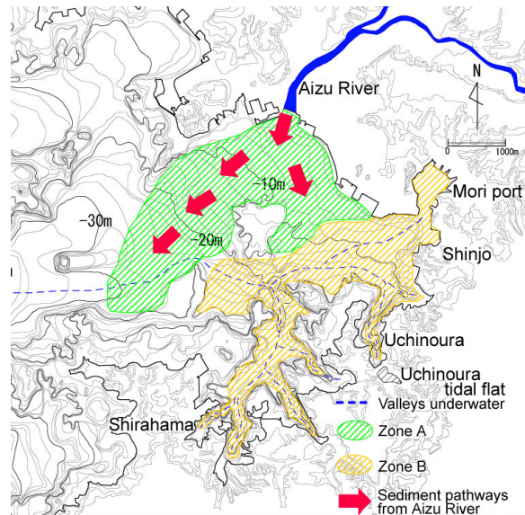
Fig. 29 Identification of distributions of coarse-grained sediment (zone A) and fine-grained sediment (zone B)
