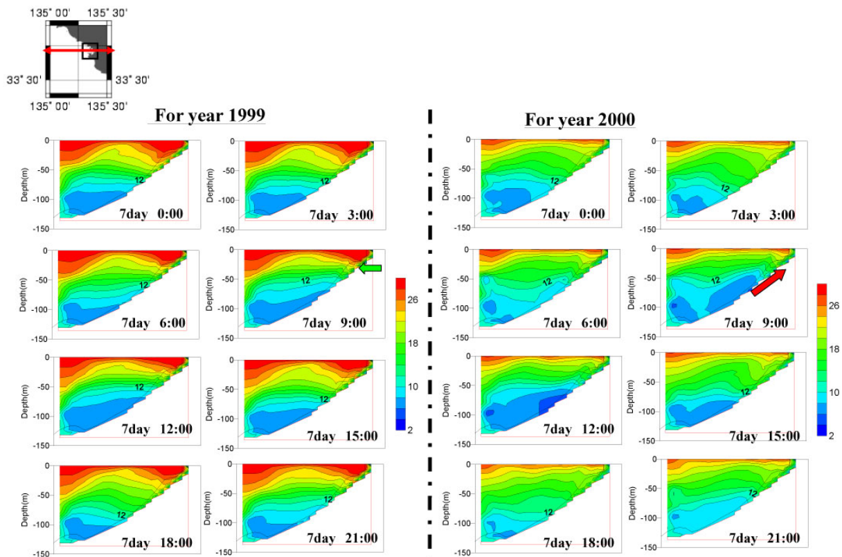
Fig. 26 Calculated profiles of seawater temperature across and beyond Tanabe Bay
