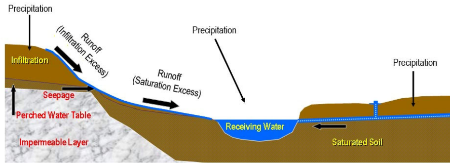
Fig. 2 Pathways of precipitation-derived water flow in hilly watershed
