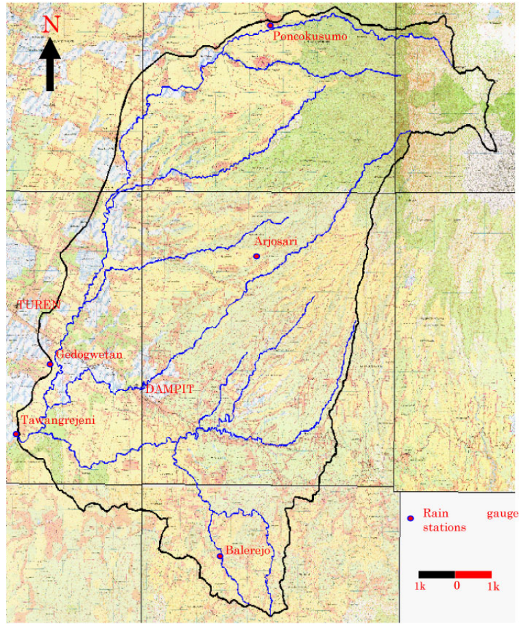
Fig. 5 Lesti Basin in east Java, Indonesia, which extends upstream of Tawangrejeni gauge station
