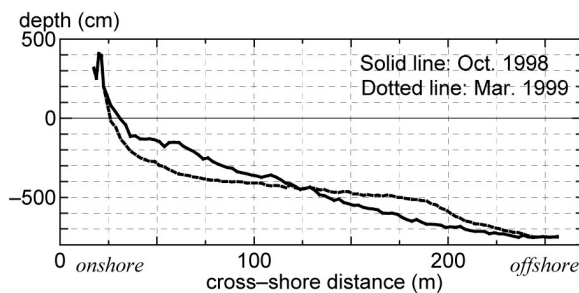
Fig. 18 Measured cross-shore profiles suggesting the occurrence of event-related sediment transport in a period between October 1998 and March 1999
