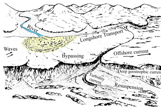
Fig. 1 Schematic of sediment routing system (adapted from Seibold and Berger, 1993)
