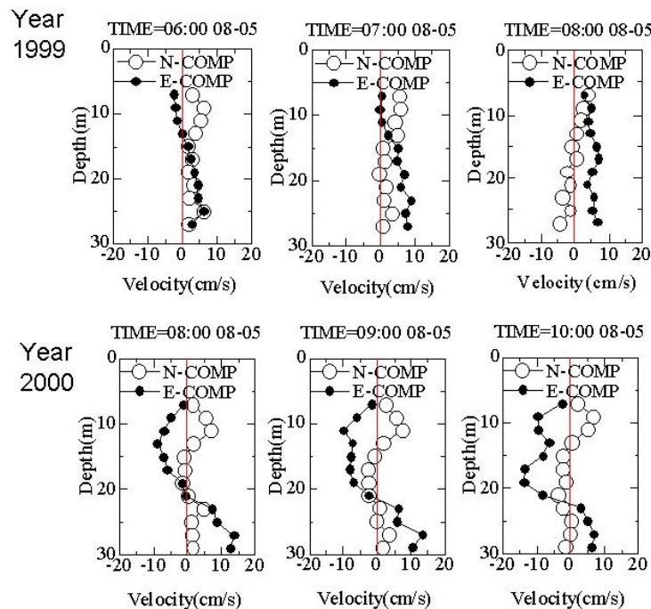
Fig. 24 Observed profiles of flow velocities of seawater
