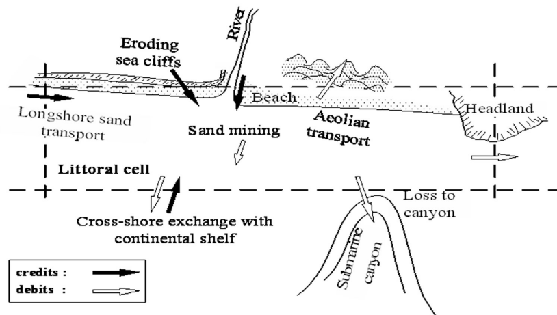
Fig. 15 Principal components involved in the development of a budget of littoral sediment (adapted from Komar, 1998)
