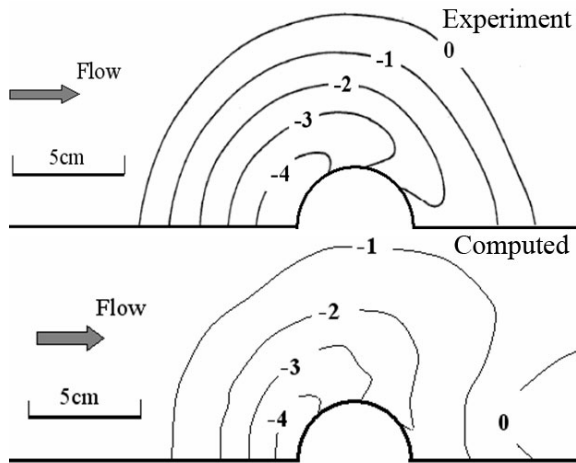
Fig. 9 Comparison between measured and predicted performances of local scour at T=0.5 hours. (Zhang et al. 2007a)
