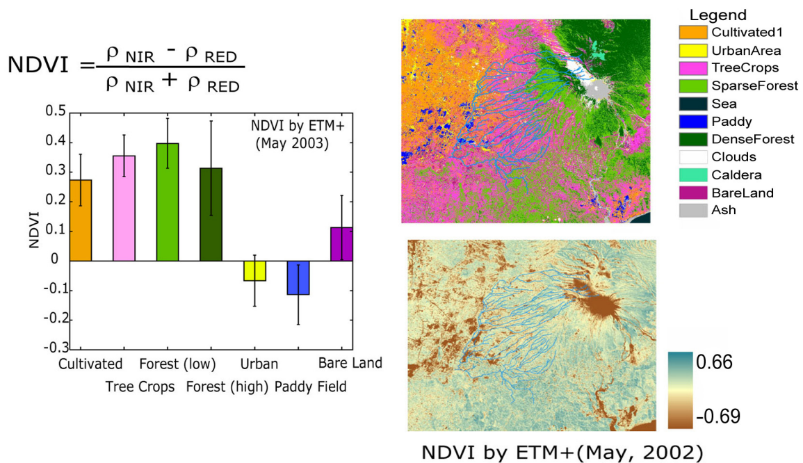
Fig. 4 Correlation of NDVI with land use patterns
