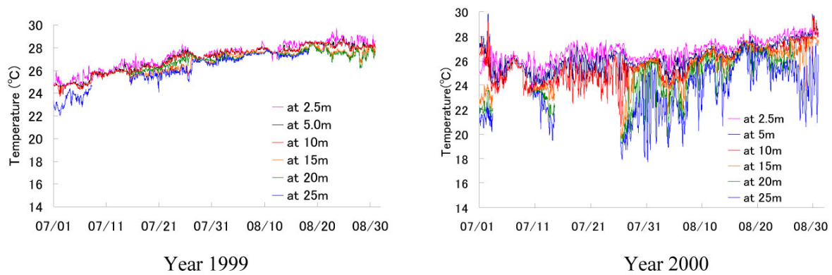
Fig. 23 Measured time histories of seawater temperatures at the observation tower in Tanabe Bay
