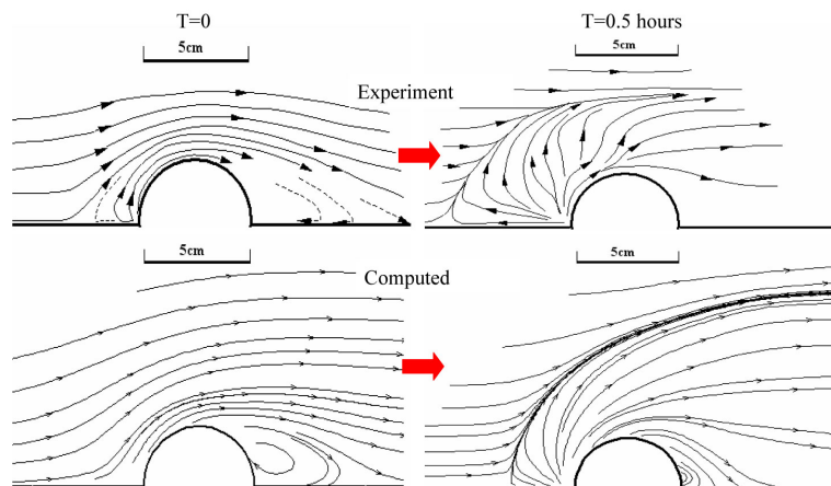
Fig. 10 Measured and predicted evolutions in streamlines at a level of 2mm above the bed (Zhang et al. 2007a)
