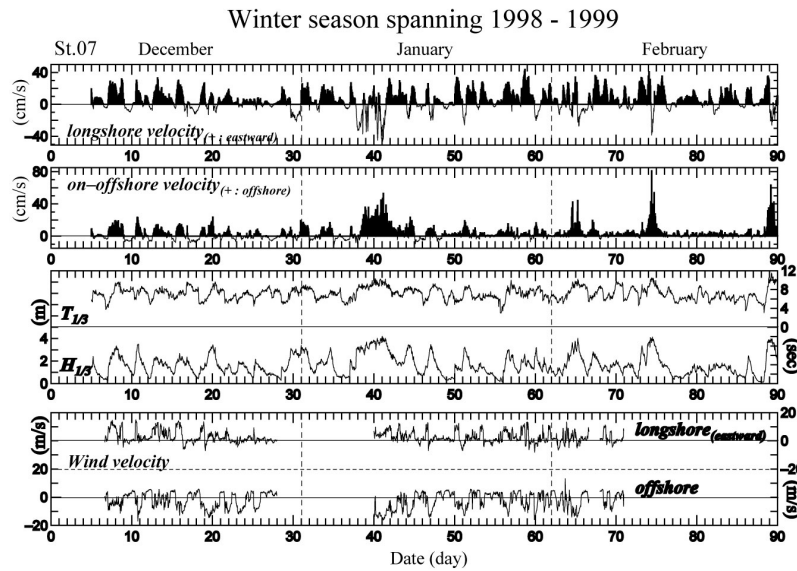
Fig. 17 Measured time histories of current velocities, wave climate and wind velocities that feature winter storminess in Ogata coast (Kato et al., 2002)
