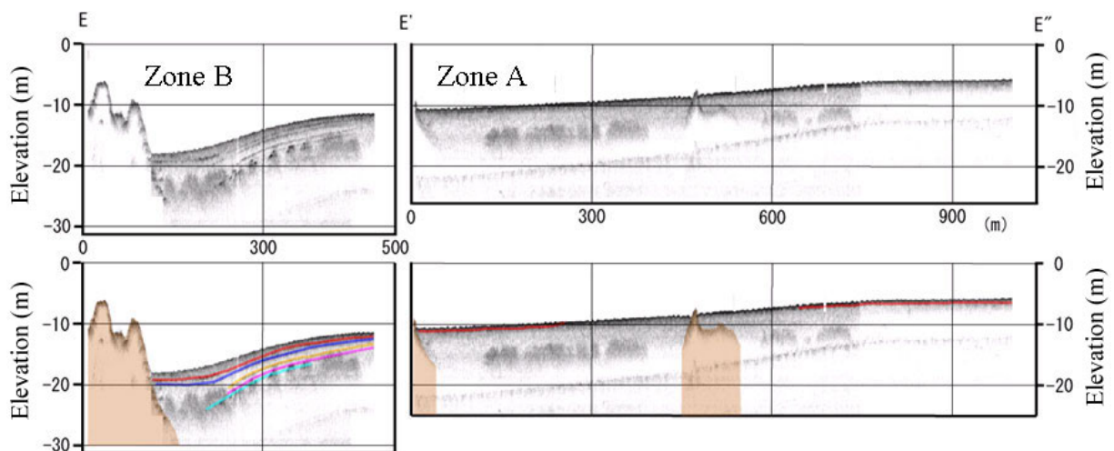
Fig. 30 Comparison of in-line seismic profiles with distinct reflectors captured
