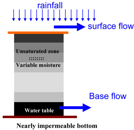
Fig. 2 Pathways of precipitation-derived water flow in hilly watershed
