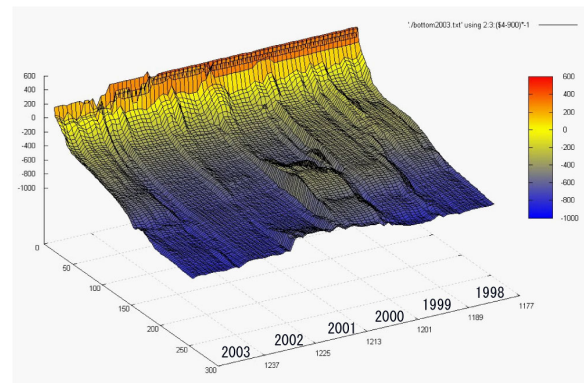
Fig. 19 A snapshot of the measured evolution of seabed profile along the observation pier
