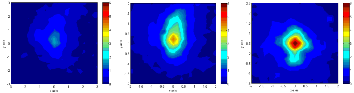
Figure 3.14: Spatial distribution at different distance from second parabolic mirror, 130 mm, 100 mm, and 68 mm (focusing point).
