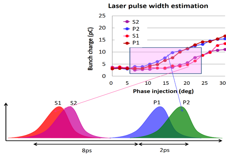
Figure 6.11: Pulse duration in case of the time scale T1 and T2 fixed at 0.2 inch.
