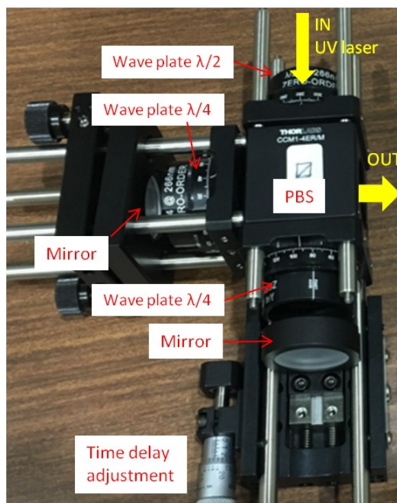
Figure 6.5: Laser pulse stacking (LPS) system.
