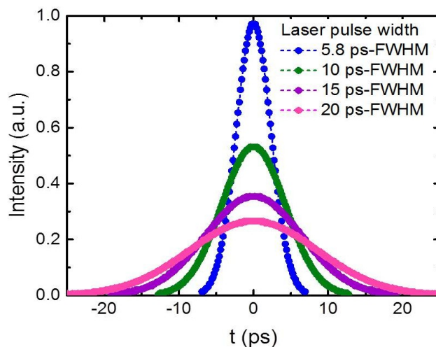
Figure 5.7: Dependence of the longitudinal distribution on the laser pulse width before irradiation with a fixed bunch charge.
