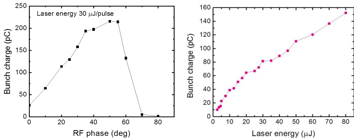
Figure 3.3: (left) Bunch charge as a function of RF phase using laser energy of 30 \mu\text{J/pulse} and (right) laser energy vs. bunch charge at a suitable RF phase of about 12 degrees for bunch compression.
