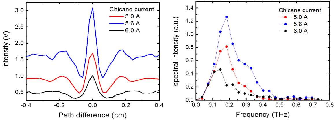
Figure 4.13: (left) Interferogram and (right) frequency spectrum from CTR measurement with the bunch charge of 60 pC at different chicane current.
