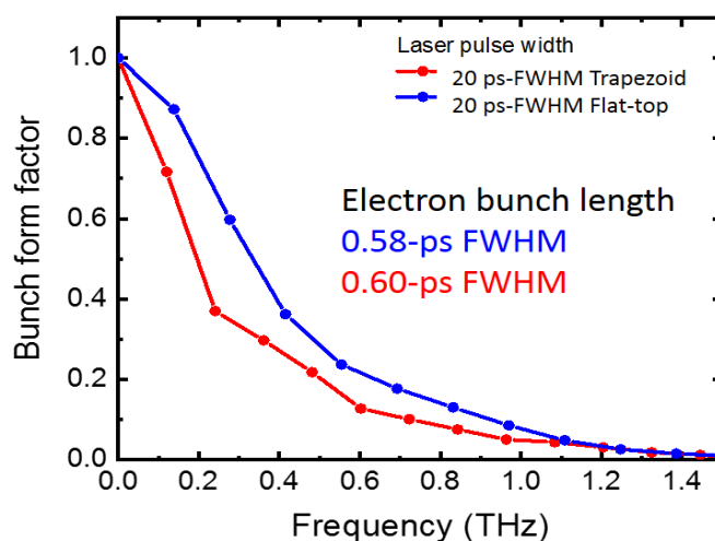
Figure 6.15: Bunch form factor performed by GPT simulation at bunch charge of 100 pC.
