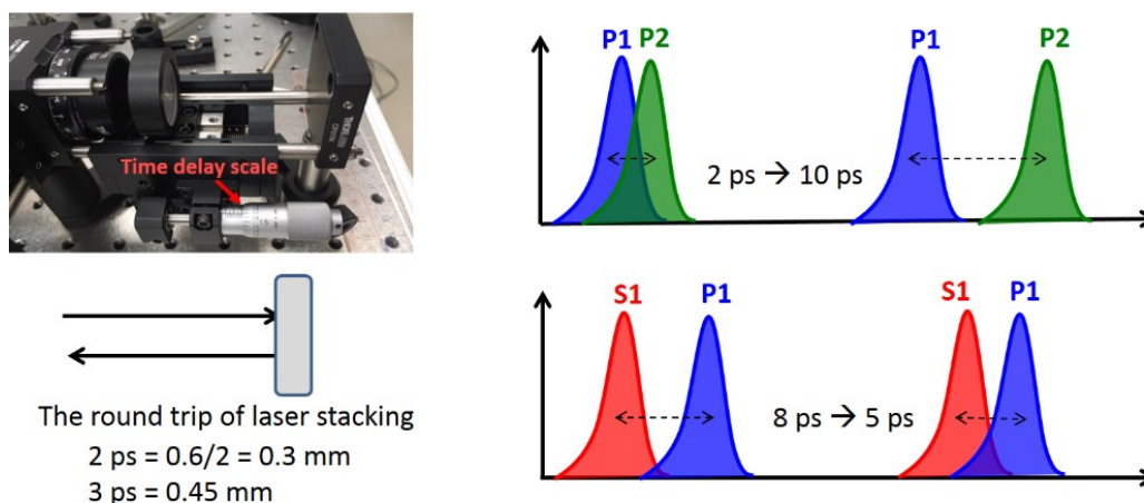
Figure 6.12: Time delay adjustment and the pulse duration arrangement for double stages of laser pulse stacking to obtain 20 ps-FWHM.
