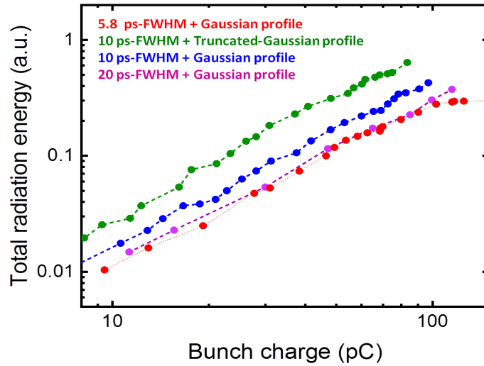
Figure 6.23: Total radiation energy of THz-CUR with the undulator gap of 50 mm (0.51 THz) as a function of bunch charge by using truncated-Gaussian and Gaussian transverse distribution.
