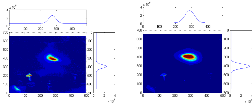
Figure 4.21: Electron beam profile on screen monitor inside undulator at the bunch charge of 60 pC and 160 pC.
