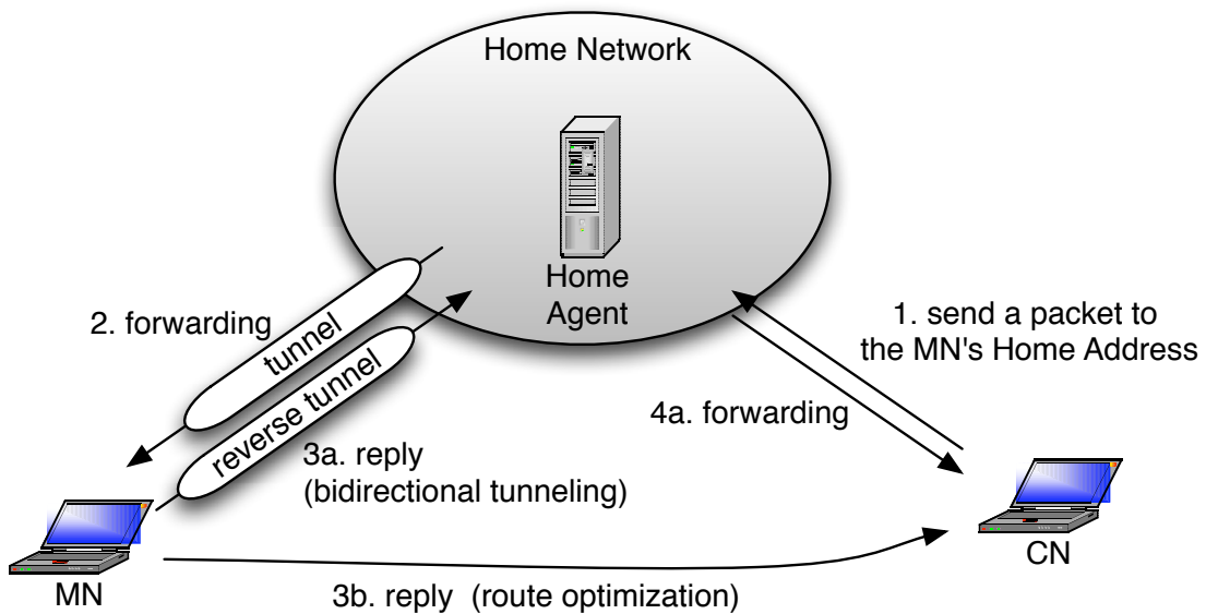
Figure 1: Mobile IPv6
