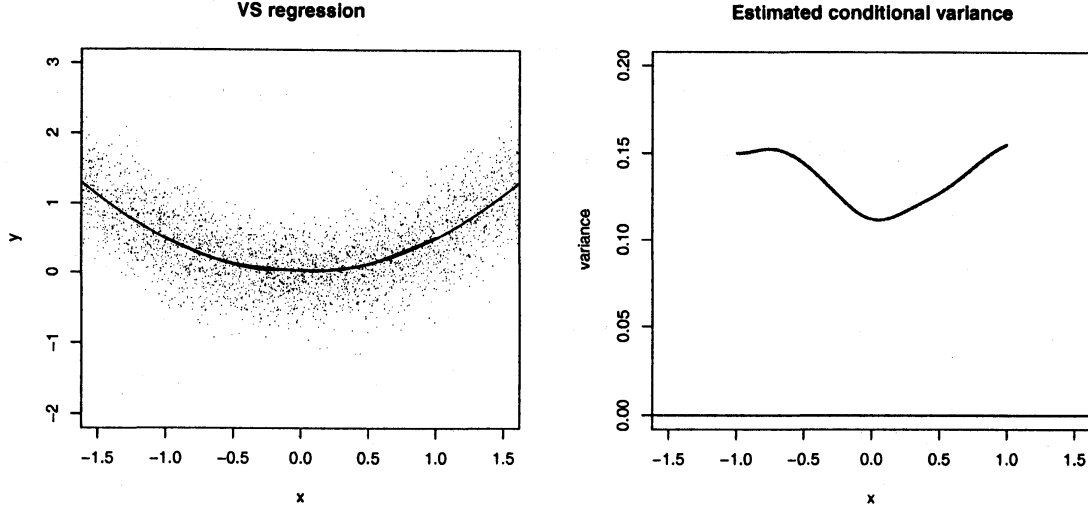
Figure 1: The left panel plots the variance-stabilizing regression obtained by the estimating procedure. The right panel is the nonparametric regression of the conditional variance function obtained in the process of the estimating procedure.
