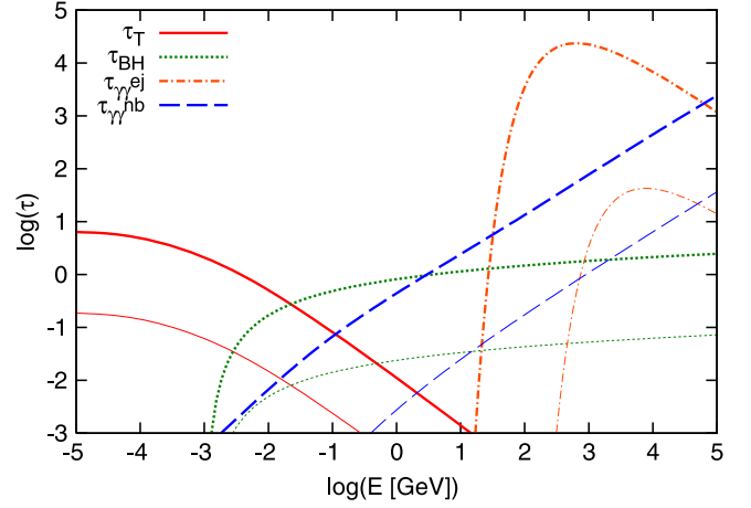
Figure 3. Optical depths to Compton (solid curves), Bethe–Heitler (dotted curves), and two-photon annihilation (dotted–dashed curves) for thermal targets; dashed curves for non-thermal targets) processes, for (P_i, B_{\text{dip}}, M_{\text{ej}}) = (2 \text{ ms}, 10^{14} \text{ G}, 5 M_\odot) . Thick and thin curves are for t = 10^{6.75} \text{ s} and t = 10^{7.5} \text{ s} , respectively. One sees that not only SN photons but also synchrotron photons are relevant for two-photon annihilation. Synchrotron photons can prevent multi-GeV gamma rays from leaving the emission.
