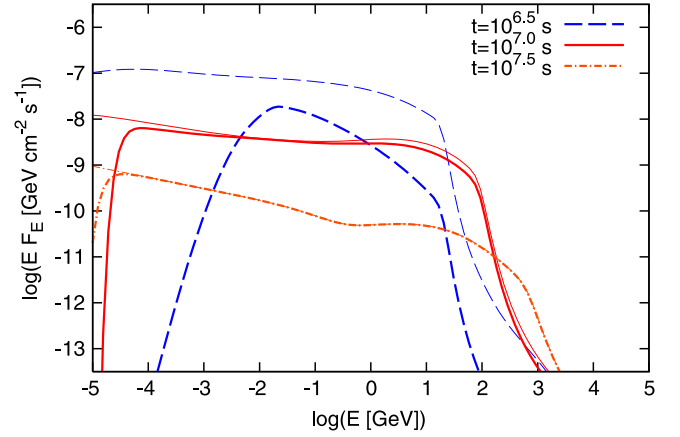
Figure 6. The same as Figure 5, but at different observation times.
