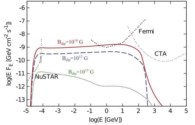
Figure 9. High-energy photon spectra of the early PWN embedded in the SN ejecta for P_i = 10 ms at t = 10^{7.25} s \approx 206 days. Different magnetic field strengths are considered.
