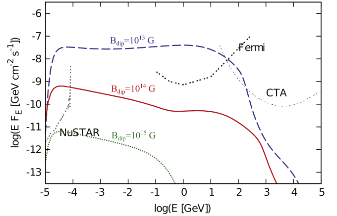
Figure 7. High-energy photon spectra of the early PWN embedded in the SN ejecta for P_i = 2 \text{ ms} at t = 10^{7.5} \text{ s} \simeq 316 days. Different magnetic field strengths are considered. Detections with CTA are possible for B_{\text{dip}} = 10^{13} \text{ G} .
