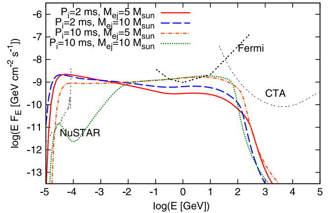
Figure 11. High-energy photon spectra of the early PWN embedded in the SN ejecta for different values of P_i and M_{\text{ej}} . The observation time is set to t = 10^{7.25} s \approx 206 days.
