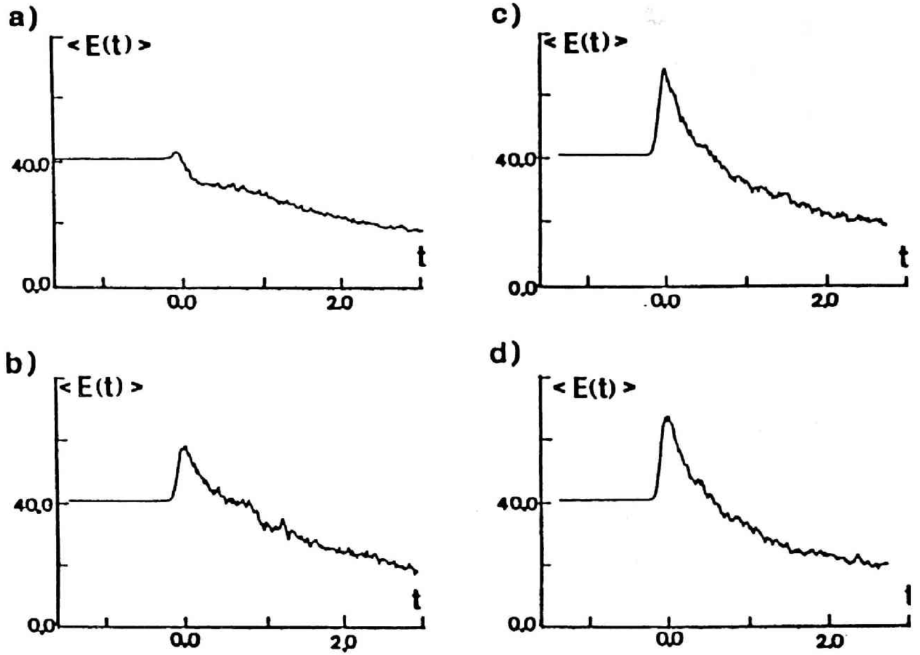
Fig 7.3 The time evolution of the total energy per particle, \langle E(t) \rangle is shown for a) A \xrightarrow{\quad} B reaction and b)-d) A \xleftrightarrow{\quad} A^* \xleftrightarrow{\quad} B reaction. Here the parameters are chosen as nd^2 = 0.770 , \varepsilon = 10.0 , \Delta Q = 40.0 and c_R = 0.5 for all cases and \varepsilon' = b) 0.0, c) 10.0 and 15.0, respectively.
