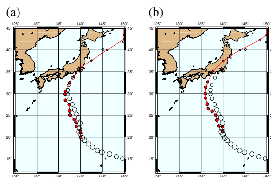
Fig. 3: Track forecast from (a) 0000 UTC, and (b) 1200 UTC. Black circles indicate the best track.
