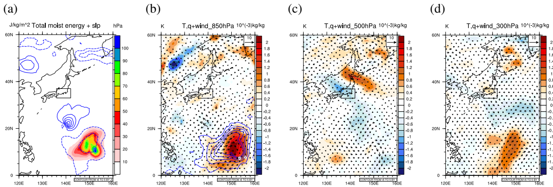
Fig. 5: The 1st mode of ensemble sensitivity analysis at the initial time in terms of (a) the total moist energy (color, \text{J kg}^{-1} \text{m}^{-2} ) and sea level pressure (contour, every 0.5 hPa), winds (vector, \text{m s}^{-1} ), temperature (color, K), and specific humidity (contour, every 10^{-3} \text{kg kg}^{-1} ) at (b) 850 hPa, at (c) 500 hPa, and at (d) 300 hPa, respectively. The black box indicates the verification region.
