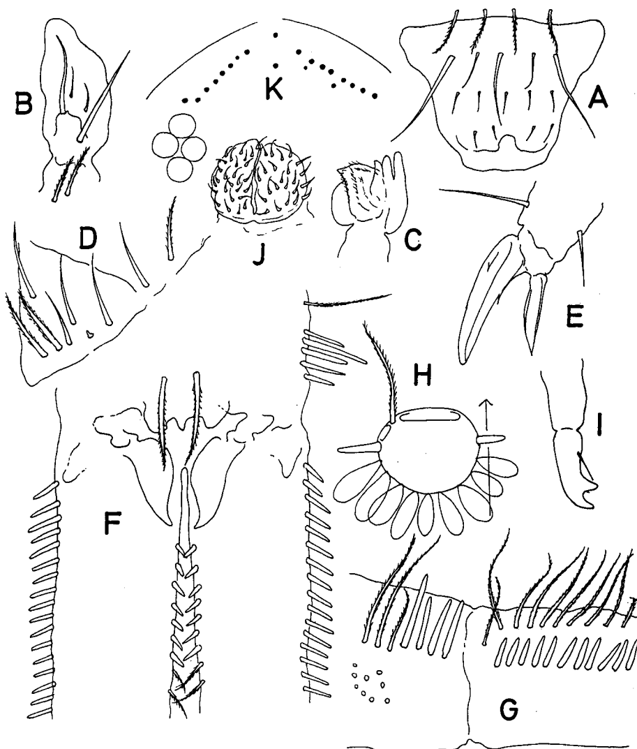
Fig. 1. Pseudosinella (Astrocyrtus) speciosa sp. n. A: labrum, B: outer maxillary lobe, C: maxillar head, D: labial basis, E: hind claw, F, G: manubrium and dens (ventral and outer lateral view), H: cross section of dens (diagram), I: mucro, J: male genital orifice, K: frontal area and eyes.
