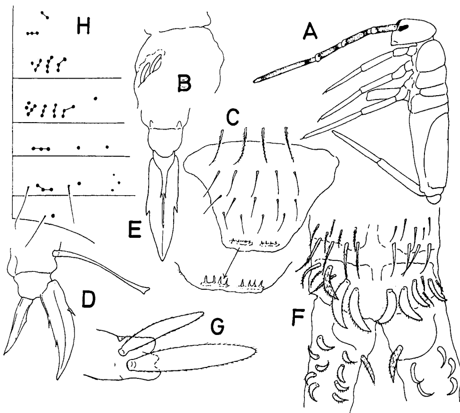
Fig. 10. Pseudoparonella (Oceaniella) shibatai Yosii A: habitus, B: ant. III-organ, C: labrum, D: hind claw, E: unguis (inner view), F: distal area of manubrial dor- sum, G: mucro, H: macrochaetotaxy of the trunk.
