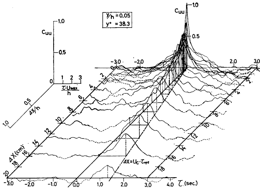
Fig. 7. Longitudinal space-time correlation of C_{uu} obtained at y^+ = 38 .
