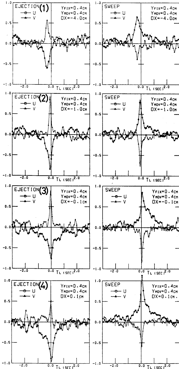
Fig. 14. Conditionally averaged space-time correlations \langle u \rangle(\tau) and \langle v \rangle(\tau) in the wall region (i.e. at y^+=38 ) when the ejection motion or the sweep motion occurs at the fixed probe ( y_{fix}^+=38 ).
