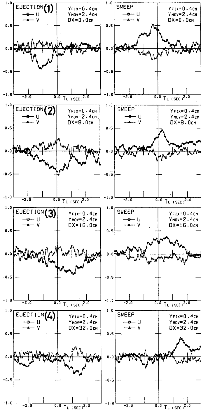
Fig. 15. Conditionally averaged space-time correlations \langle u \rangle(\tau) and \langle v \rangle(\tau) in the equilibrium region (i.e. at y/h=0.9 ).
