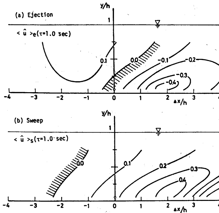
Fig. 22. Spatial iso-patterns of \langle u \rangle at the time when \tau U_{max}/h = 2.6 passed after the occurrence of the bursting motion at the detecting probe.
