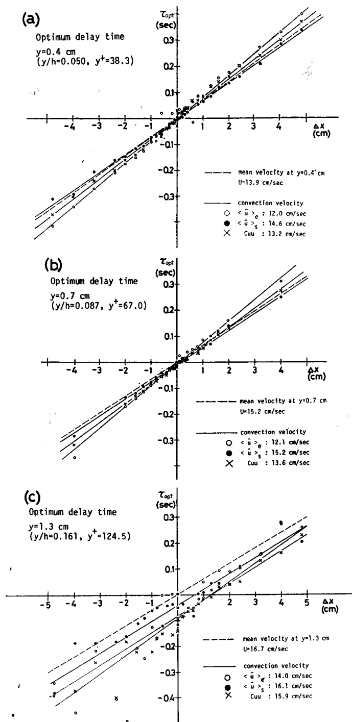
Fig. 23. Optimum delay time \tau_{opt} of \langle u \rangle against the separation \Delta x .
