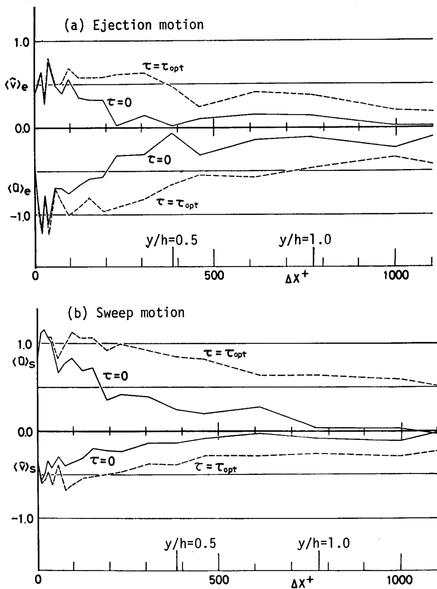
Fig. 17. Space structures of \langle u \rangle(\Delta x) and \langle v \rangle(\Delta x) of the ejection and sweep motions observed at y^+=38 .
