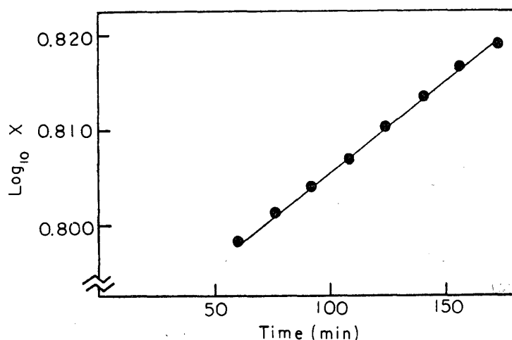
Fig. 7. Sedimentation velocity data of \log_{10} x vs. time (min) in 0.15 M KCl.
