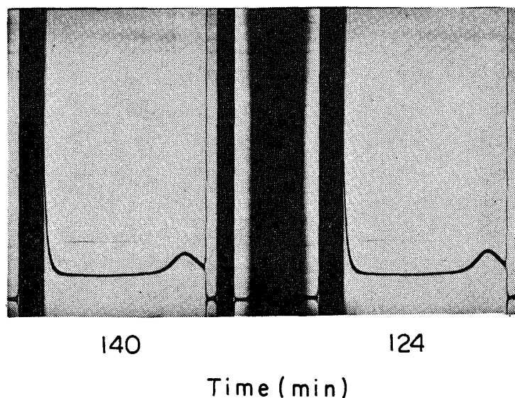
Fig. 8. Sedimentation patterns of bamboo xylan (AX-1) in 0.15 M KCl. Sedimentation proceeds from right to left. The photographs were taken at indicated times after reaching full speed at 52,640 rpm.
