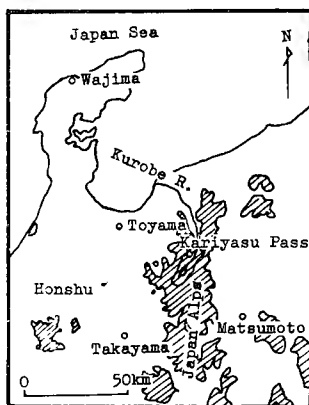
Fig. 1. General topography (Shaded area is higher than 1500 m)
