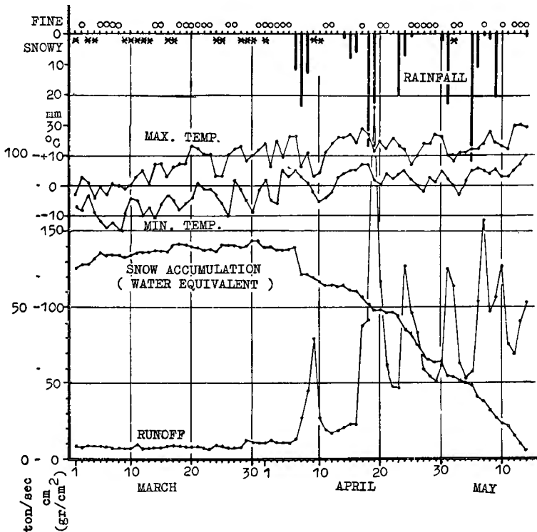
Fig. 2. Snow melting and runoff. (Temperature, rainfall and weather are observed at the dam control office near the dam site (1460 m))
