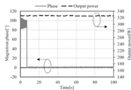
Fig.2: Magnetron phase and output power when the PLL circuit start working.
