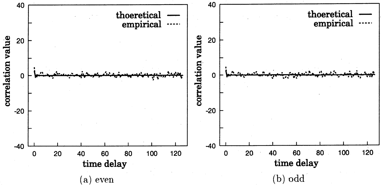
Figure 3: (a) \langle R_N^E(\ell; A_8, A_9) \rangle and \hat{R}_{N,M}^E(\ell; A_8, A_9) , (b) \langle R_N^O(\ell; A_8, A_9) \rangle and \hat{R}_{N,M}^O(\ell; A_8, A_9) , where N = 127 , M = 100 , and k = 16 .
