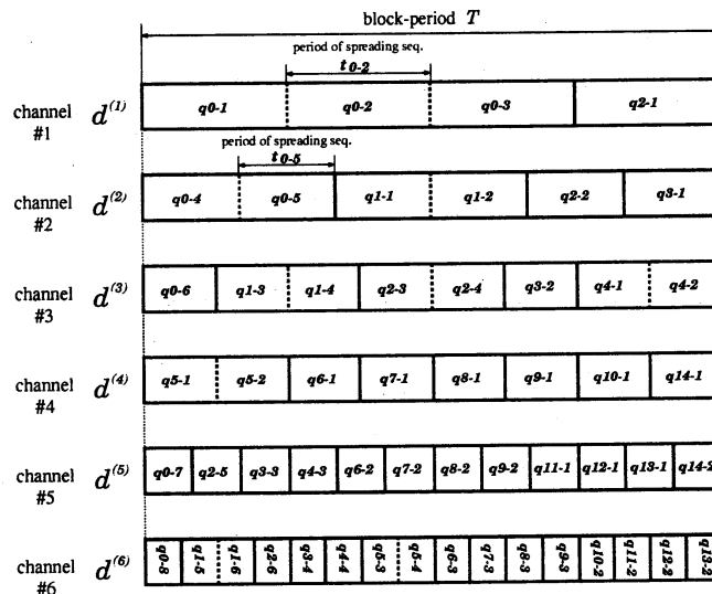
Figure 16: Model-2 with spreading sequences of variable-period.
