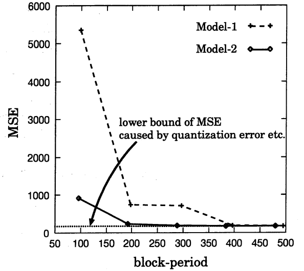
Figure 19: MSEs versus block-periods.
