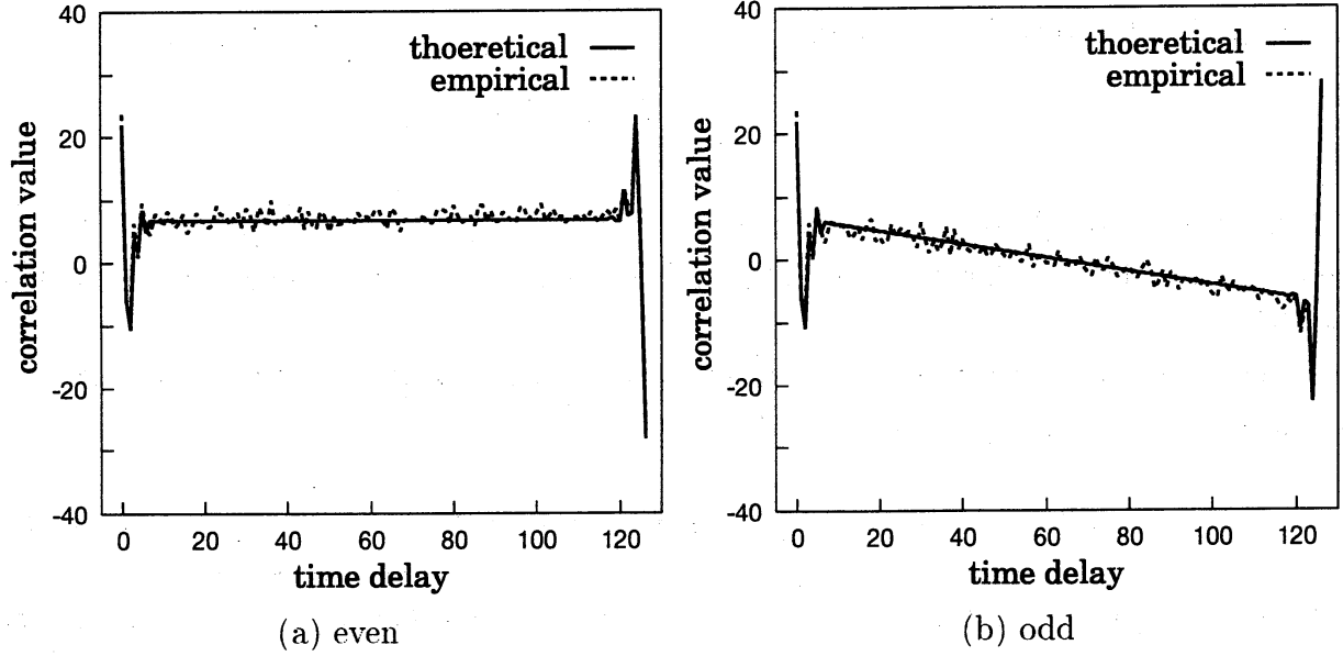
Figure 2: (a) \langle R_N^E(\ell; A_2, A_3) \rangle and \hat{R}_{N,M}^E(\ell; A_2, A_3) , (b) \langle R_N^O(\ell; A_2, A_3) \rangle and \hat{R}_{N,M}^O(\ell; A_2, A_3) , where N = 127 , M = 100 , and k = 2 .
