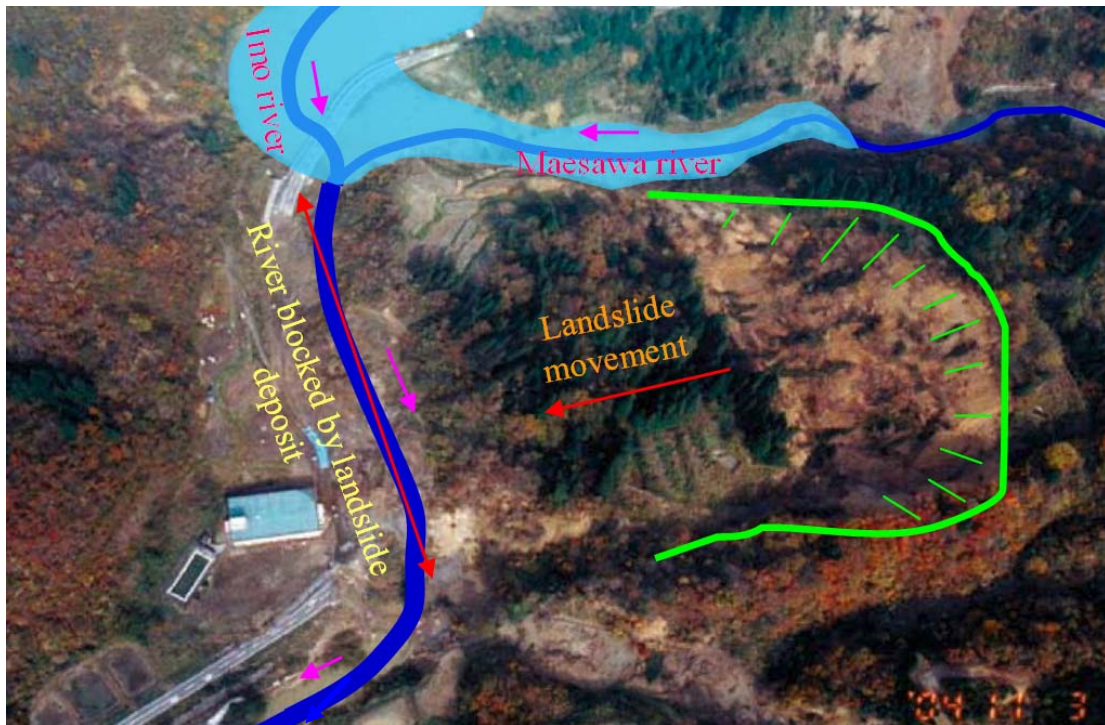
Plane view of the Higashi-Takezawa Landslide
