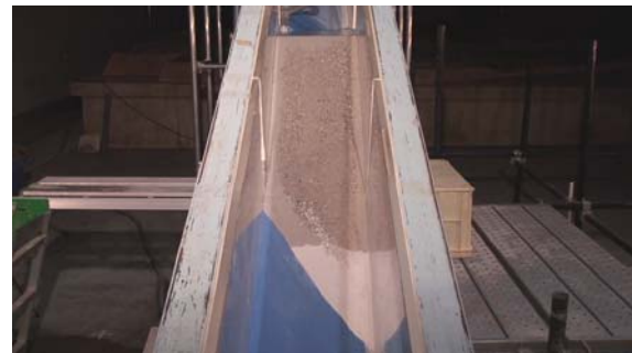
Figure 4.13 Movement of slide at different time steps - Experiment C
