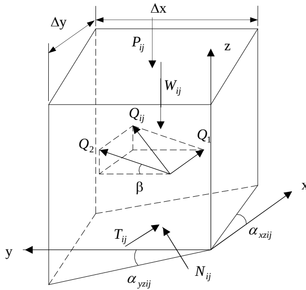
Figure 4.9 Forces acting on a typical column
