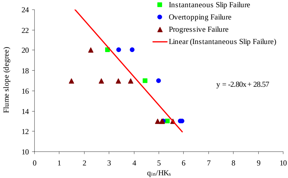
Figure 2.12 Graphical relationship to predict failure modes (Sediment Mix 1-6)
