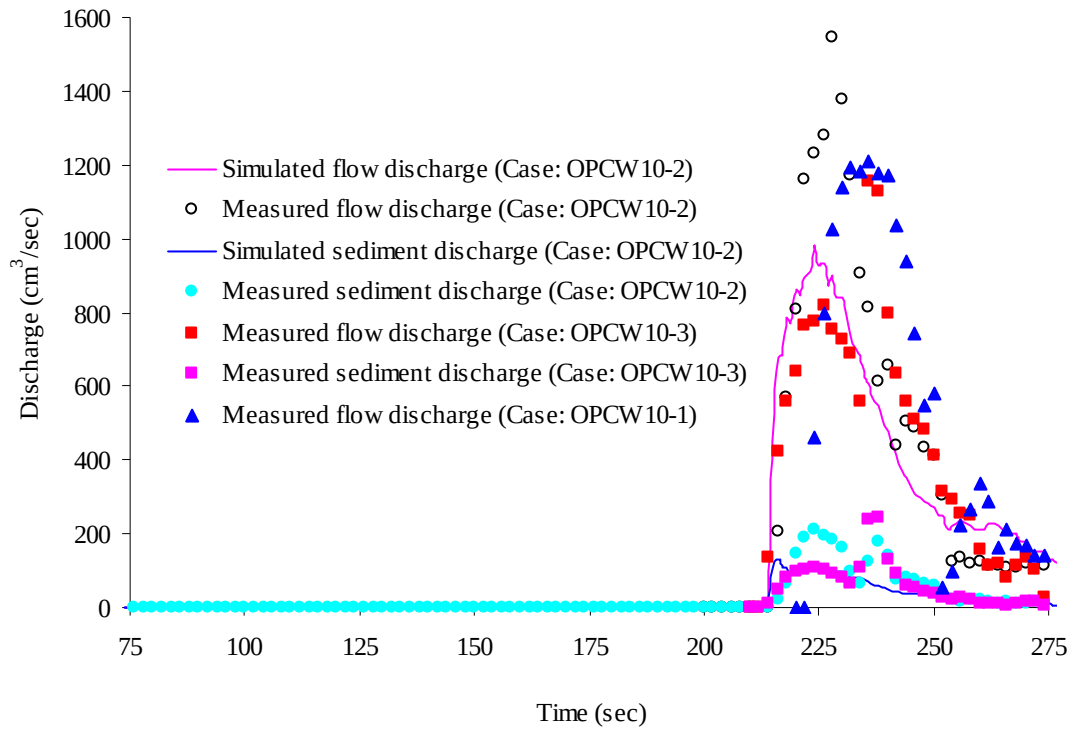
Figure 5.11 Outflow hydrograph (channel slope = 10^\circ )
