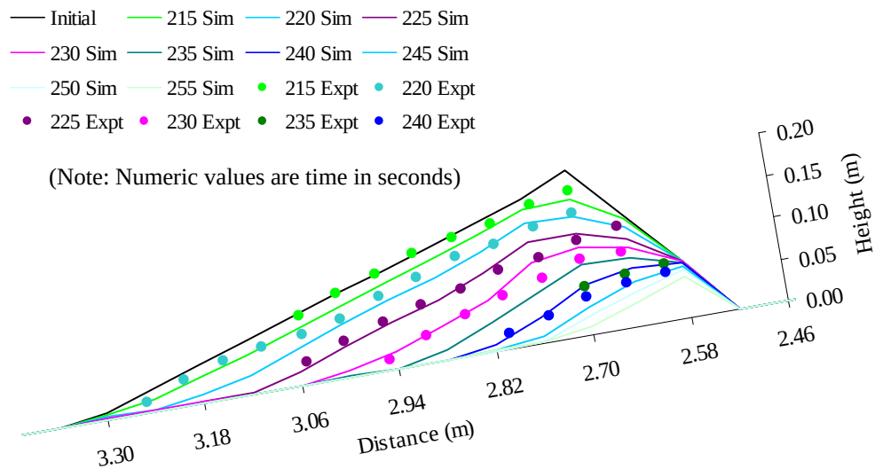
Figure 5.12 Comparison of dam surface erosion at incised channel, (channel slope = 10^\circ )
