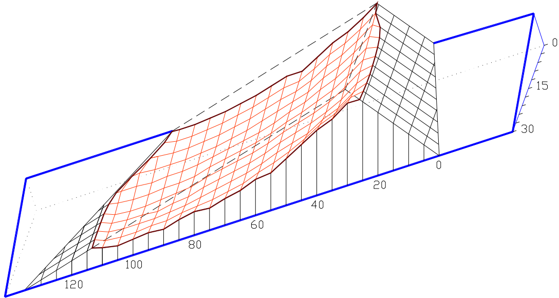
Figure 4.15 Simulated critical slip surface at t = 0\text{sec} .
