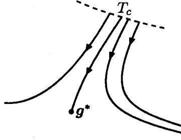
FIG. 1: Typical RG trajectories near a phase transition. As T changes, an initial value moves on the dashed line. The trajectory with T = T_c is absorbed into the fixed point g^* .
