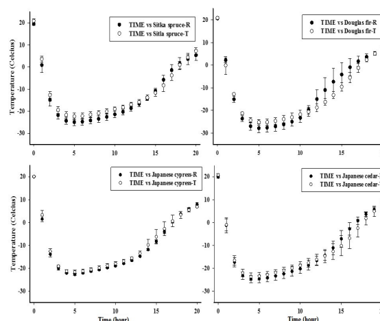
Figure 1. Comparison of the thermal conductive properties values obtained in both tangential and radial direction using solid carbon dioxide slabs
