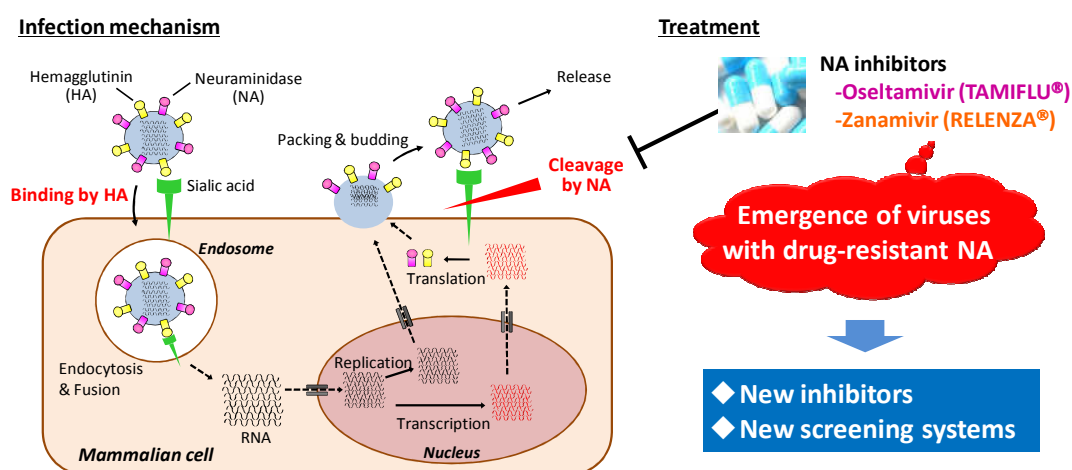
Fig. 6. Infection and expansion mechanisms of influenza virus and neuraminidase inhibition by small molecules
