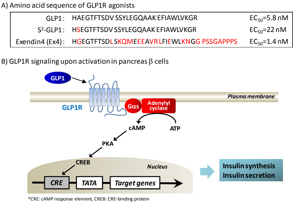
Fig. 5. Amino acid sequence of GLP1R agonists and GLP1R signaling in pancreas β cells
