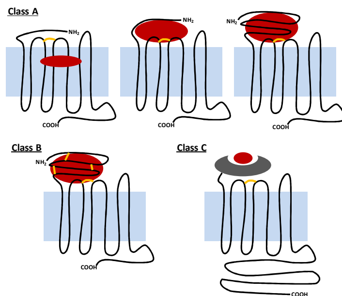
Fig. 3. Classification of human GPCRs [24] Red: ligand, Yellow: disulfide bond, sky blue: membrane lipid bilayer
