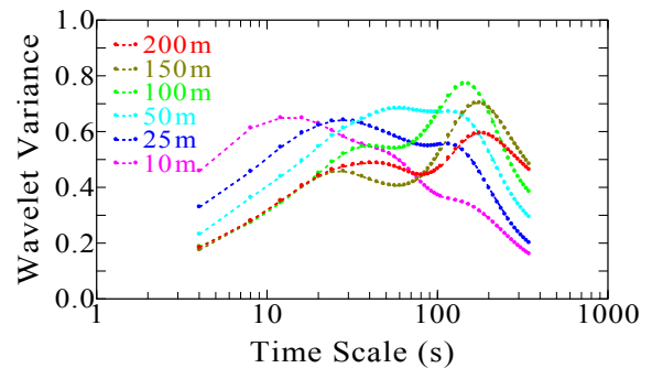
Fig. 2 Wavelet variance spectra for the u velocity component (case No. 29, 1330–1700 LST on March 29, 2000)
