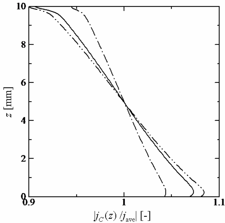
Figure 3.10: Steady state vertical current density distribution along the cathode surface for (j_{\text{ave}} [\text{mA}/\text{cm}^2], L [\text{mm}]) = (2, 2) (solid line), (1, 2) (dashed-dotted line), and (2, 1) (dashed-two dotted line).
