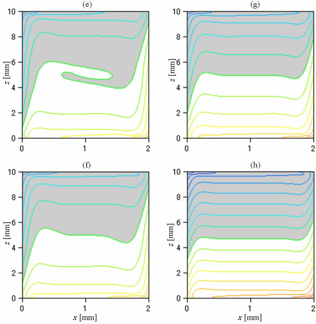
Figure 3.6: Transient variations in contour of concentration profile. (a) t [s]=24, (b) 54, (c) 96, (d) 132, (e) 258, (f) 414, (g) 906, (h) 6000. The region where the concentration is less than the initial value of 0.6 M is shaded. The contour interval is m_0/30 .
