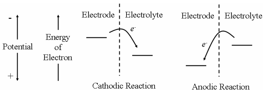
Figure 2.2: Schematic description of the relative energy difference of the electron in anodic and cathodic reactions. The dashed line indicates the electrode/electrolyte interface.
