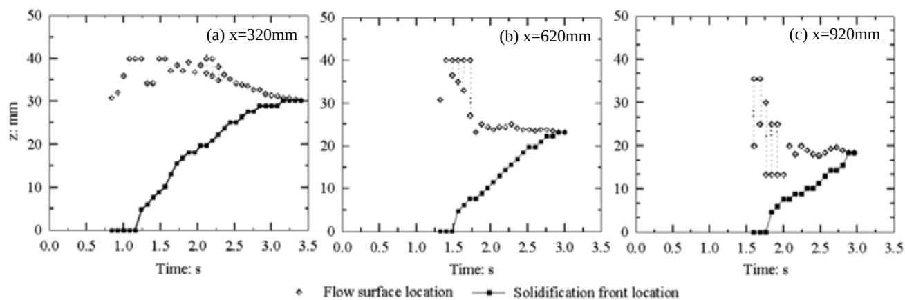
Fig. 10 Evolutions of flow surface and solidification front at three different stations in sediment gravity flow ( c=38\% )
