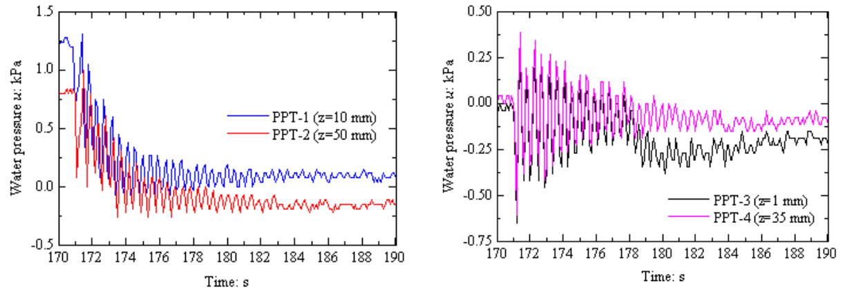
Fig. A-5 Measured time histories of water pressures after the release of the gate (PPTFLOW-1)
