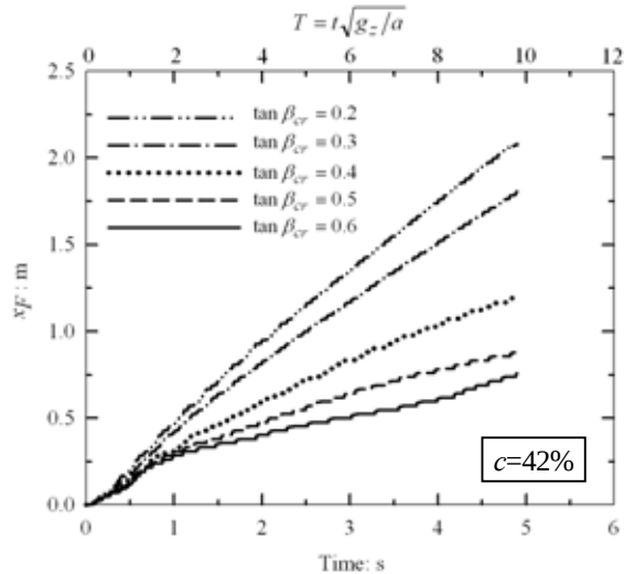
Fig. 12 Predicted time histories of location of gravity flow head for five different values of \tan \beta_{cr}
