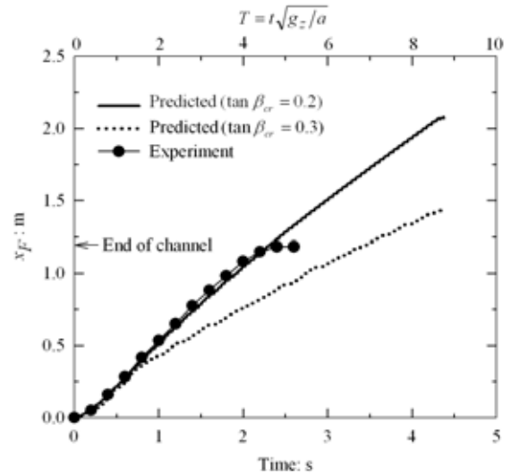
Fig. 14 (b) Predicted and measured time histories of location of gravity flow head for c=34\%
