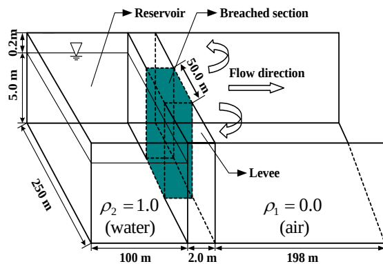
Fig. 16 Definition sketch for three-dimensional levee breaching problem
