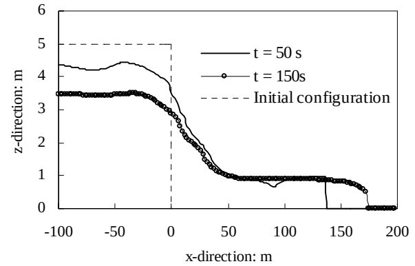
Fig. 17 Predicted flow configurations
