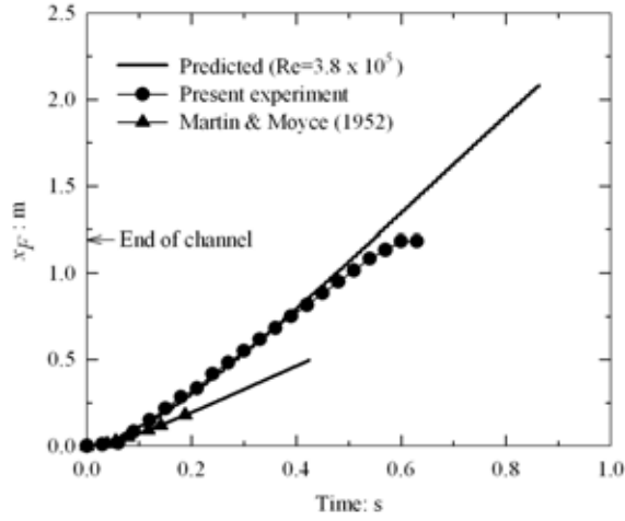
Fig. 11 Measured and predicted time histories of location of gravity flow head for clear water
