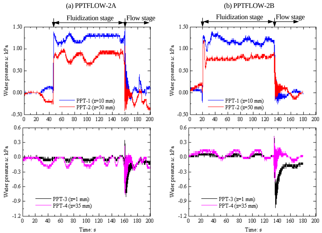
Fig. A-2 Measured time histories of water pressures in sediment gravity flow experiment (PPTFLOW-2)
