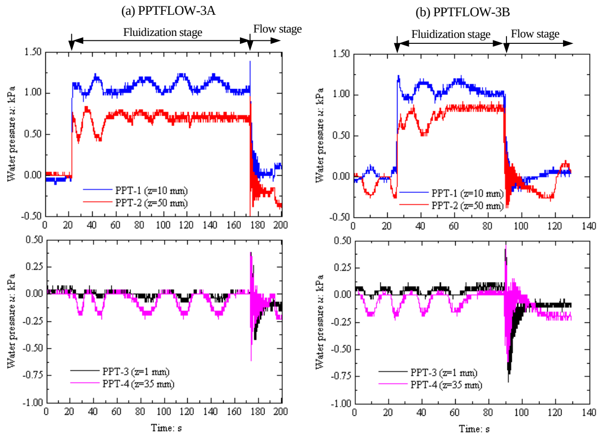
Fig. A-3 Measured time histories of water pressures in sediment gravity flow experiment (PPTFLOW-3)
