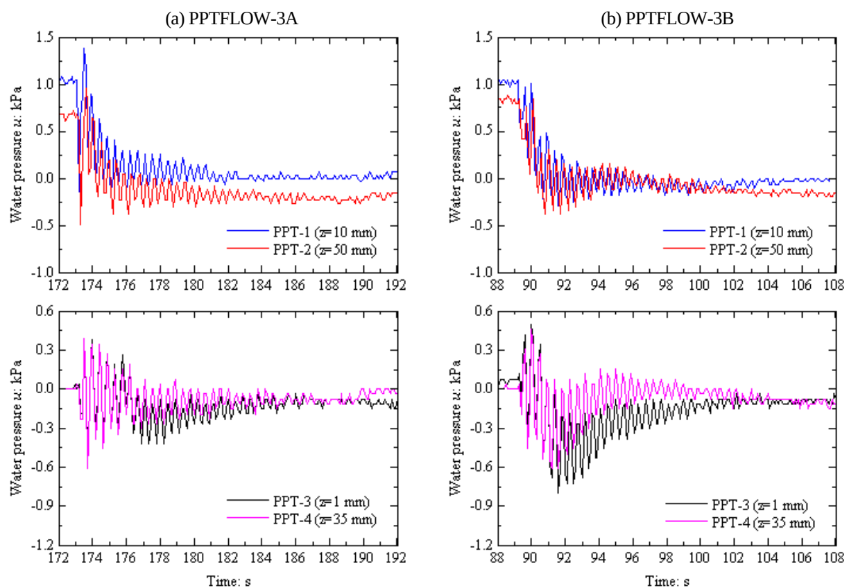
Fig. A-7 Measured time histories of water pressures after the release of the gate (PPTFLOW-3)
