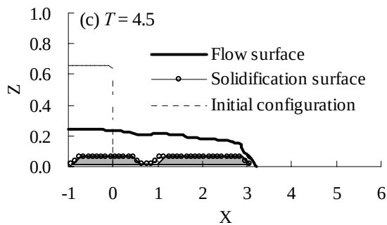
Fig. 15 Predicted flow configurations of liquefied soil with c=42\% ( \tan \beta_{cr} = 0.3 ): (a) initial configuration (b) configuration at T = 1.5 ; (c) configuration at T = 4.5 and (d) configuration at T = 9.5
