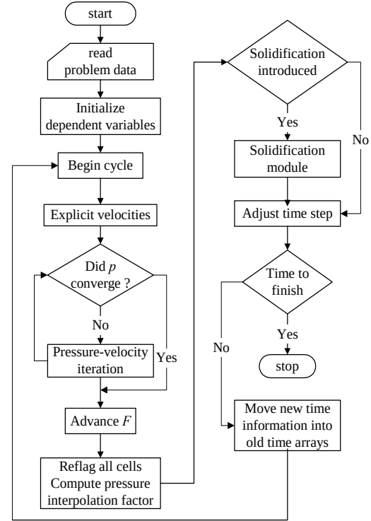
Fig. 2 Flowchart of the computer program
