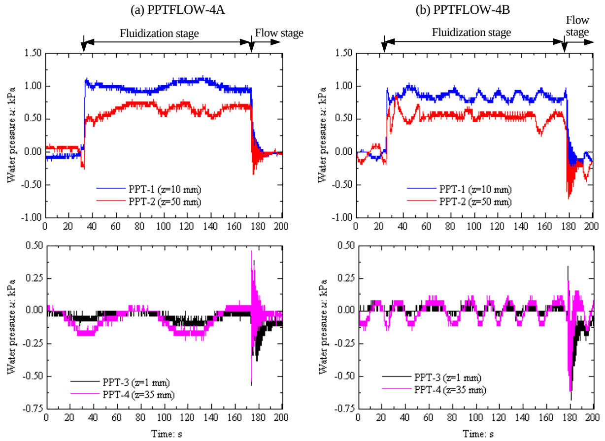
Fig. A-4 Measured time histories of water pressures in sediment gravity flow experiment (PPTFLOW-4)
