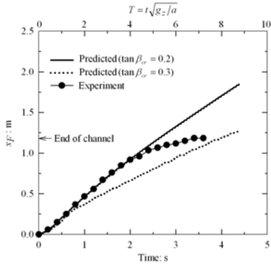
Fig. 14 (c) Predicted and measured time histories of location of gravity flow head for c=38\%
