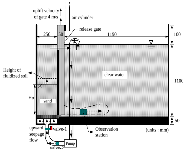
Fig. 3 Setup for experiment on sediment gravity flow following fluidization
