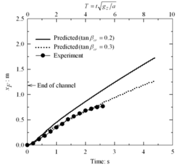
Fig. 14 (d) Predicted and measured time histories of location of gravity flow head for c=42\%
