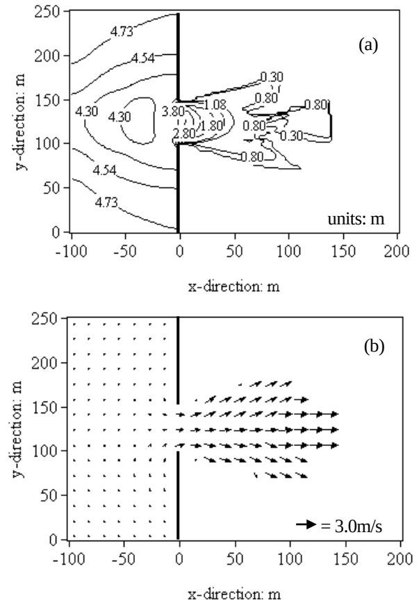
Fig. 18 Predicted flow-out pattern at t=50 s: (a) contours of equal elevations in free surface; and (b) distributions of velocity vectors on a horizontal plane, z = 1.0 m.
