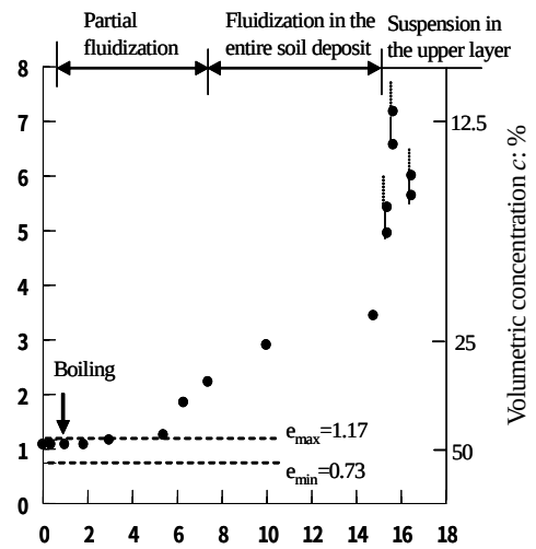
Fig. 4 Void ratios of sediment plotted against imposed vertical seepage velocities, showing transformation of the state of sediment
