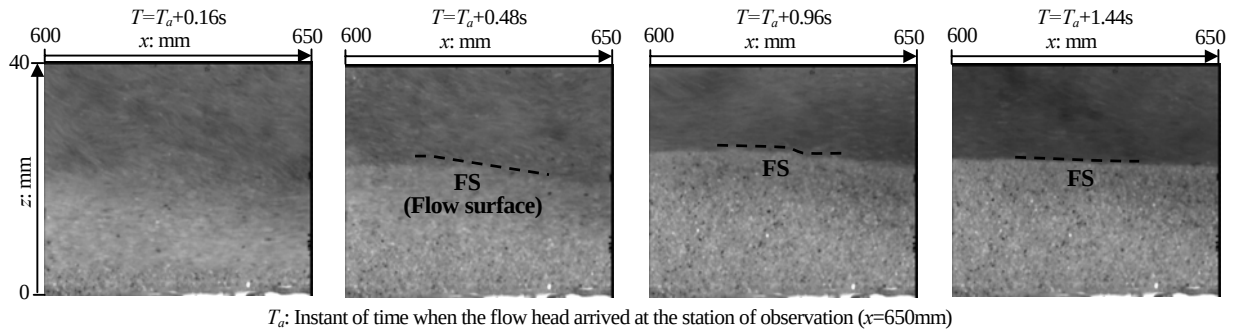
Fig. 8 (a) Snapshots of fluidized sediment gravity flow (test PPTCCD-11) from a fixed station using the high-speed CCD camera
