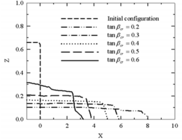
Fig. 13 Predicted configurations of liquefied soil for c=42\% at a dimensionless time T=9.5
