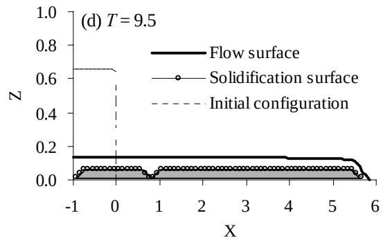
Fig. 15 Predicted flow configurations of liquefied soil with c=42\% ( \tan \beta_{cr} = 0.3 ): (a) initial configuration (b) configuration at T = 1.5 ; (c) configuration at T = 4.5 and (d) configuration at T = 9.5
