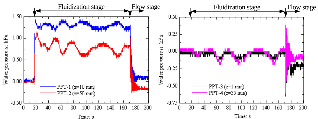
Fig. A-1 Measured time histories of water pressures in sediment gravity flow experiment (PPTFLOW-1)
