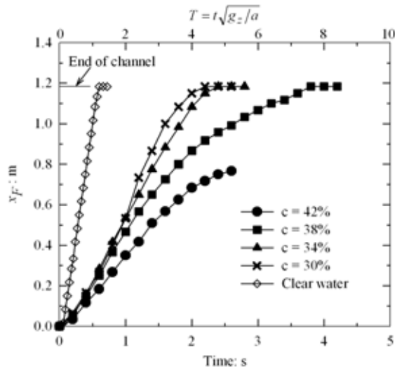
Fig. 7 Measured time histories of location of gravity flow head in second series of experiment
