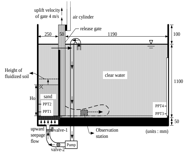
Fig. 3b Setup for experiment on sediment gravity flow following fluidization, with four PPTs installed
