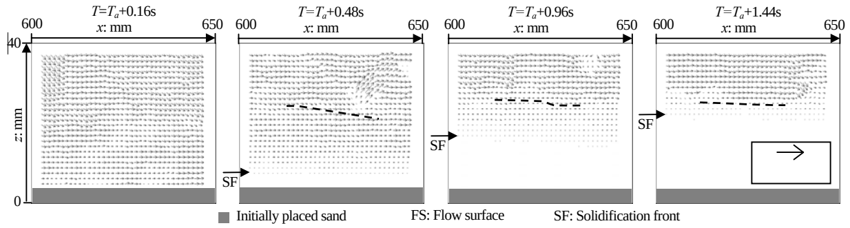
Fig. 8 (b) Velocity fields of sediment gravity flow in test PPTCCD-11 obtained through PIV technique, showing upward advance of solidification front
