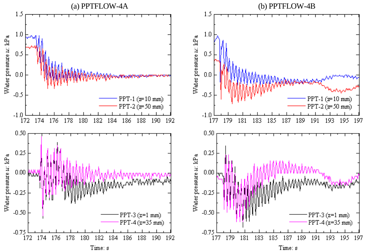
Fig. A-8 Measured time histories of water pressures after the release of the gate (PPTFLOW-4)
