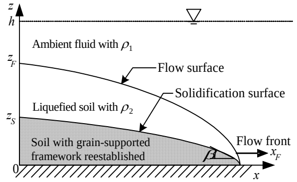
Fig. 1 Flow stratification with two moving interfaces
