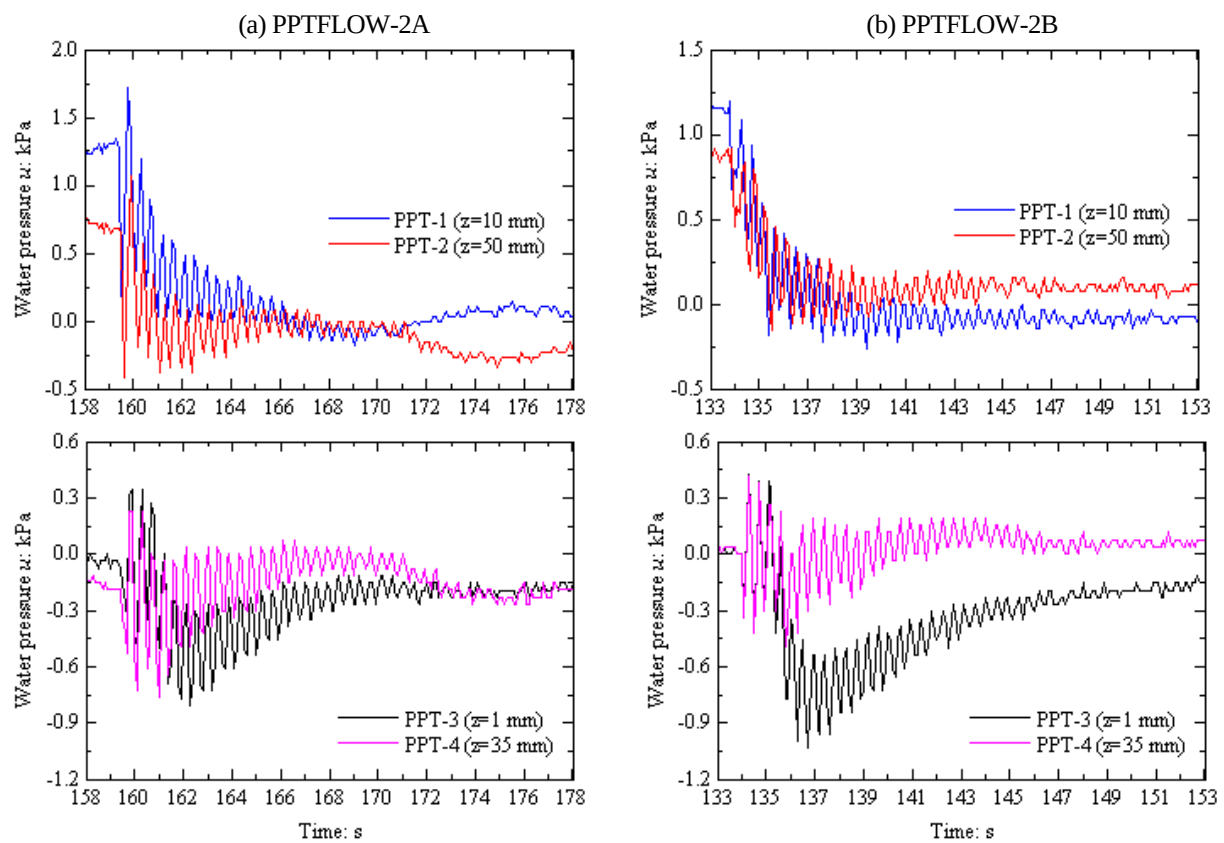
Fig. A-6 Measured time histories of water pressures after the release of the gate (PPTFLOW-2)
