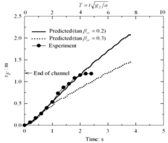
Fig. 14 (a) Predicted and measured time histories of location of gravity flow head for c=30\%
