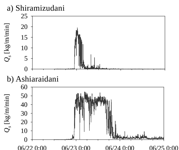
Fig. 9 Calculated bed load from 22 to 25 of June, 2009 for a) Shiramizudani and b) Ashiaraidani
