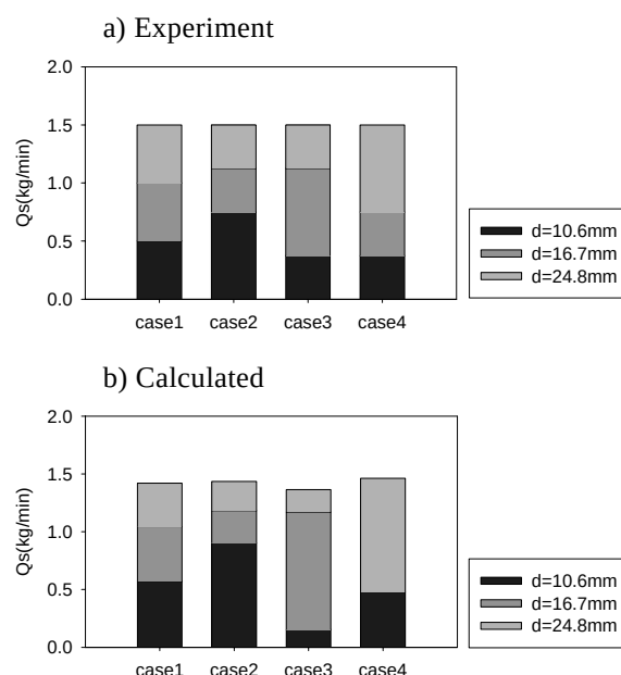
Fig. 8 Size classification of sediment load using hydrophone pulse; a) sediment ratio used in the experiment, b) calculated result
