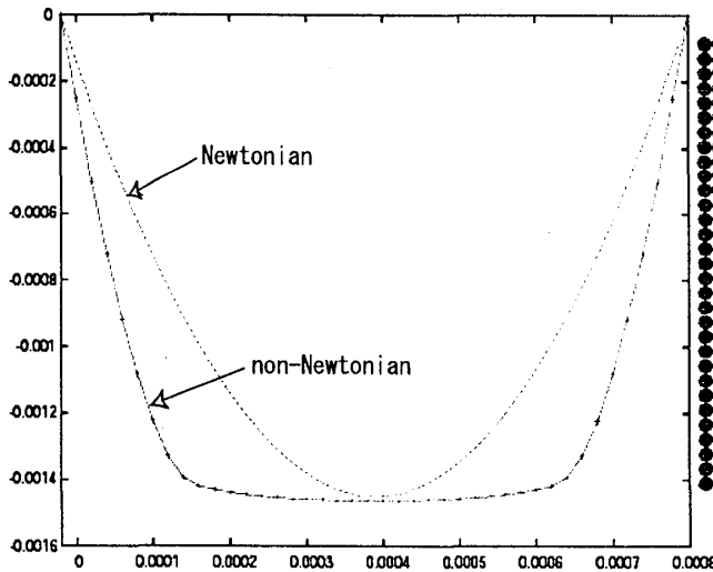
Figure 1: plug flow
