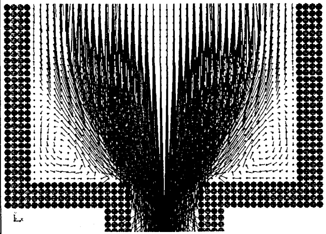
Figure 2: contraction flow
