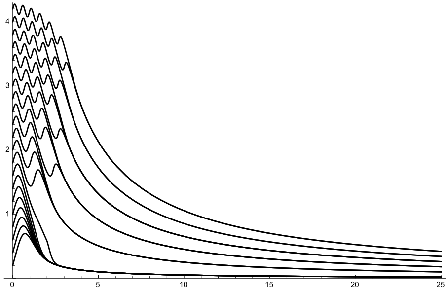
Figure 1. Graph of the solutions of (2.1) with y(0) = 0.2k ( k = 1, 2, \dots, 21 ).
