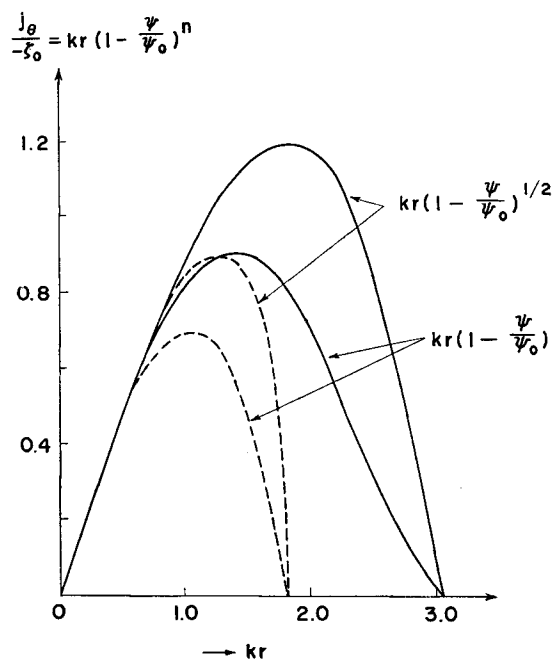
Fig. 3(a). Profile of an azimuthal current which satisfies an equilibrium state. Solid lines show the state just under the negative coil, while dotted lines show the state under the positive coil.
