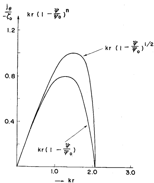
Fig. 3(b). Profile of an azimuthal current which satisfies an equilibrium state. Curves are plotted in the middle position of coils.
