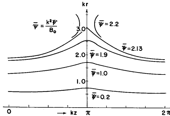
Fig. 2(b). Axisymmetric Heliotron magnetic field with \alpha=0.2 and kd=3.03 .
