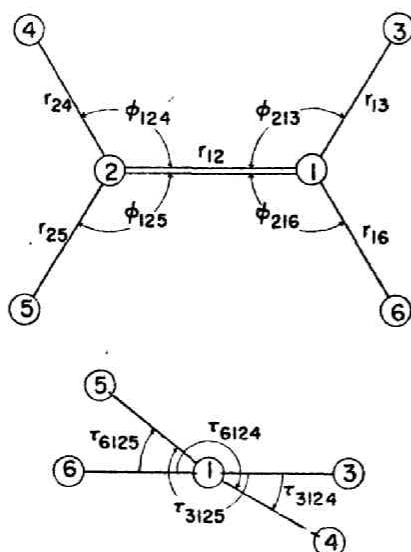
FIG. 1. Internal coordinates.
