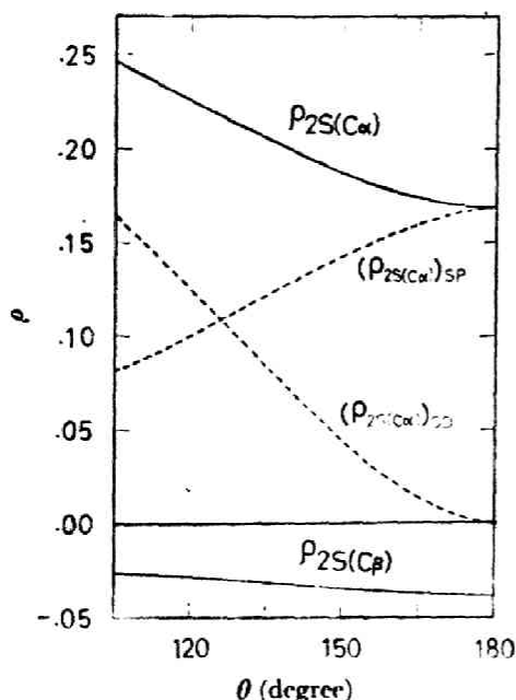
Fig. 5. 2s AO spin densities of carbon atoms versus the bending of \text{CCH}_a in the vinyl radical. Only the curves obtained before annihilation are shown, but the characteristic features are the same in both stages.
