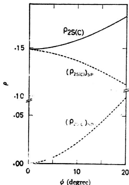
Fig. 3. \langle \rho_{2s(C)} \rangle_{ho} and its mechanistic contributions versus the bending angle \phi in the methyl radical. Only the curves obtained before annihilation are given, but the characteristic features are the same in both stages.
