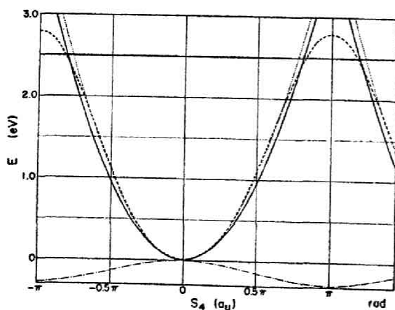
FIG. 4. Potential energy curve for the torsional coordinate: —, E (calculated); ---, E (experimental); ... E_{el} ; - · - E_{core} .
